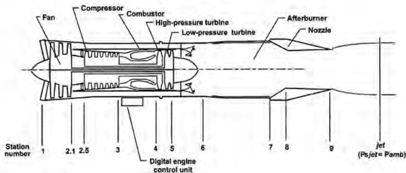
A cutaway view of the General Electric F110-GE-129 turbofan engine shows the engine station number locations. (NASA)
