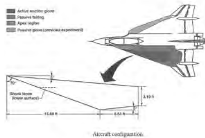
The physical dimensions of the F-16XL-2 SLFC active suction wing glove and the location of the shock fence on the underside of the left wing are shown in this NASA drawing. (NASA)
