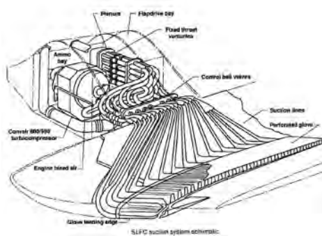
The SLFC active suction system used a turbocompressor adopted from the Convair 880 and 990 jetliners. It was tightly tailored to fit the confines of the F-16XL-1 aircraft. (NASA)
