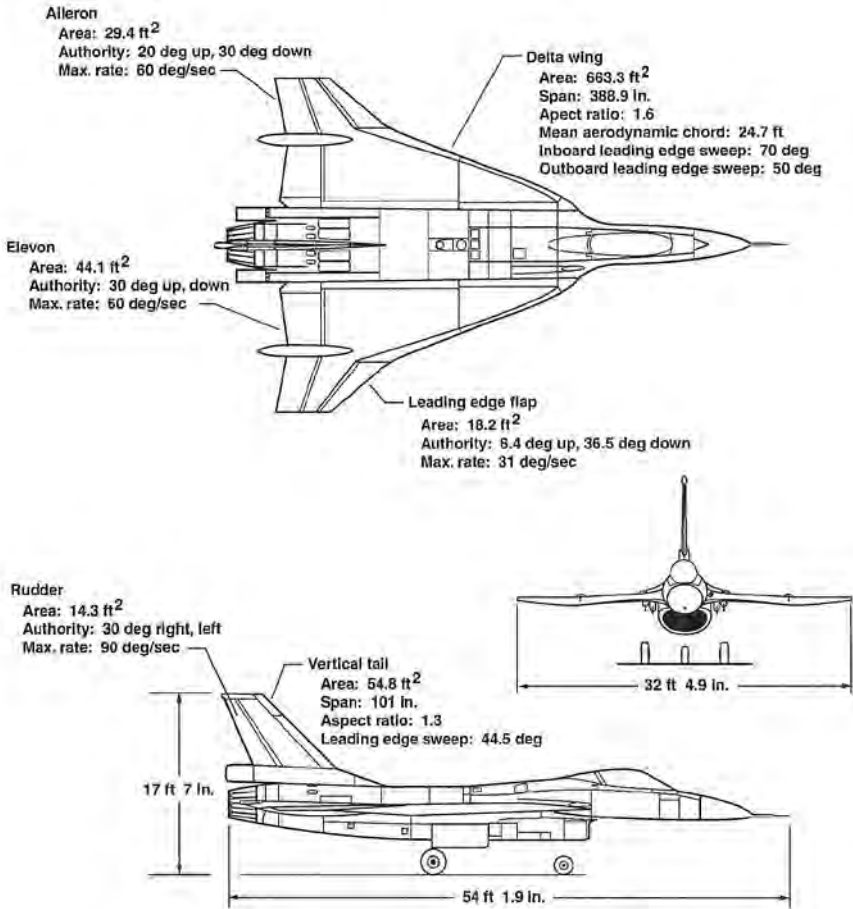
The physical and geometric properties of the F-6XL aircraft are illustrated in this NASA drawing. The effects of conical camber and twist on the wing are evident in the front view of the aircraft. (NASA)
