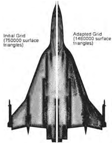
The geometric grids used for precisely modeling F-16XL geometry were very intricate in order to produce high-fidelity CFD results. (NASA)
