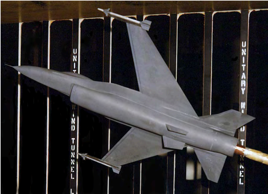
A wind tunnel test model of a modified F-16 fuselage fitted with a forward-swept wing mounted in the NASA Langley Unitary Plan Wind Tunnel in 1980. (NASA)
