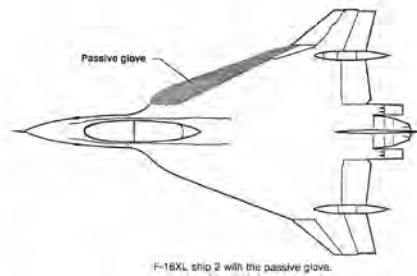
F-16XL passive and active glove configurations. (NASA)
