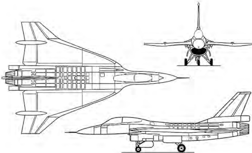
Three-view drawing of the two-seat F-16XL. (NASA)
