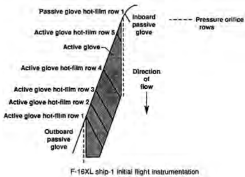
Test instrumentation used on the F-16XL-1 active suction wing glove. (NASA)
