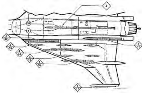
A complex hard-point arrangement was developed for the F-16XL to enable external stores to be mounted in dense conformal arrangements. (Lockheed Martin)
