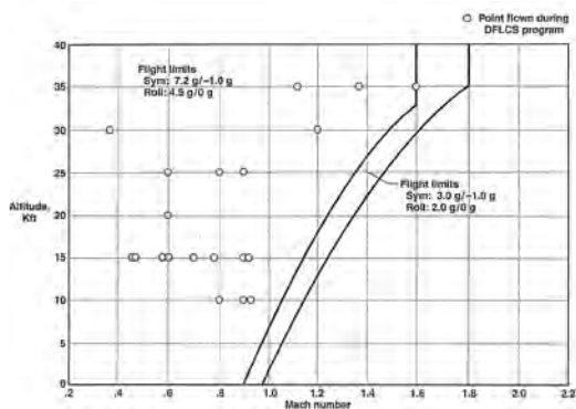
Flight envelope restrictions and maneuver limits were imposed on F-16XL-1 during the DFCS evaluation. (NASA)
