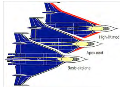
The CAWAP flight-test program was originally intended to be conducted in three phases, with the F-16XL-1 wing planform progressively modified for each phase as depicted above. (NASA)
