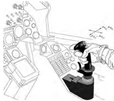
The F-16XL used the force-displacement sidestick controller adopted from the standard F-16. (NASA)
