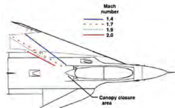
The canopy-closure shock wave impingement locations on the upper surface of F-16XL-2 are illustrated for several representative cruise Mach numbers. (NASA)
