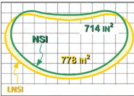
The Large Normal Shock Inlet compared to the smaller normal shock inlet. (Lockheed Martin)
