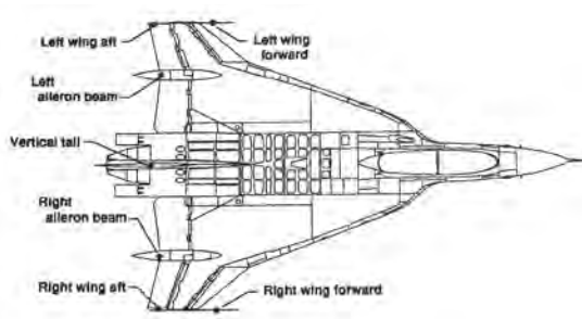
Accelerometer locations on the F-16XL airframe for use in flutter testing. (NASA)
