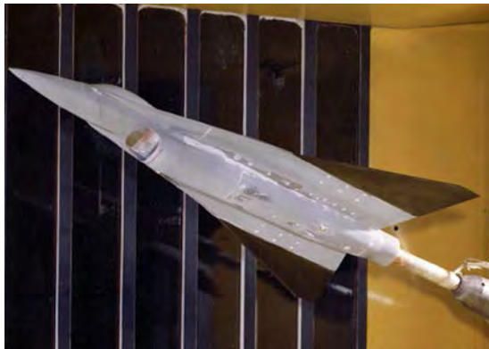
Test model of an interim SCAMP concept mounted in the NASA Langley Unitary Plan Wind Tunnel in 1978. (NASA)
