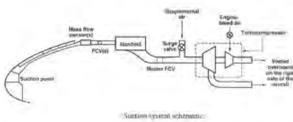
Schematic of the F-16XL-2 active wing glove suction system. (NASA)
