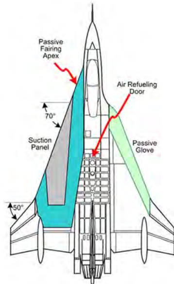
The F-16XL-2 was fitted with a General Electric F110-GE-129 engine. The passive wing glove on the right wing and active suction glove on the left wing give it a distinctive asymmetric planform. (Lockheed Martin via Robert Wetherall)
