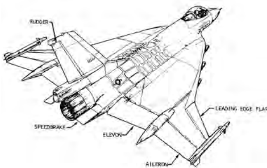
A combination of flight control surfaces provided pitch, roll, and yaw control across the entire F-16XL flight envelope. (NASA)
