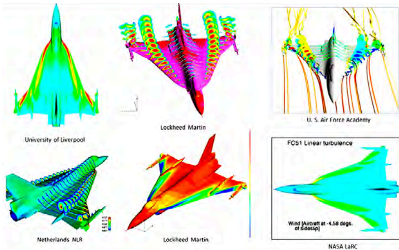
Some examples of vortical airflow over the F-16XL as graphically predicted using the CFD modeling capabilities of various national organizations. (NATO)
