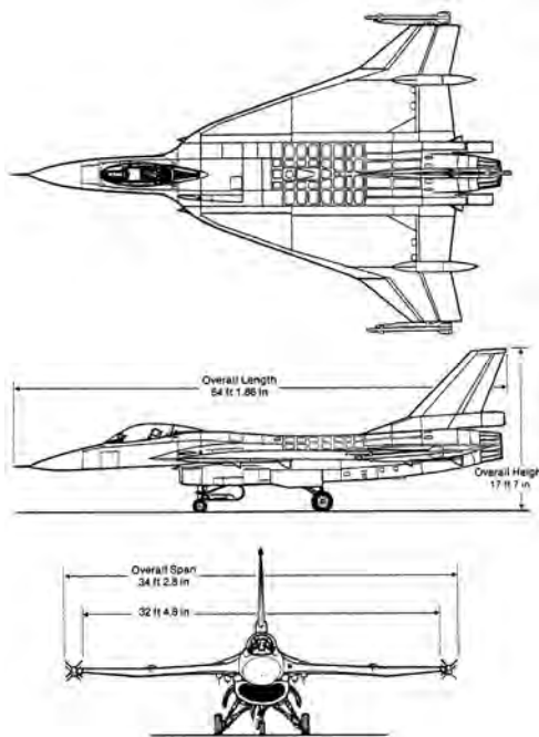
The single-seat F-16XL is illustrated with four semi-submerged AIM-120 AMRAAM radar-guided missiles and two wingtip-mounted AIM-9L infrared-guided Sidewinder missiles. (Air Force)
