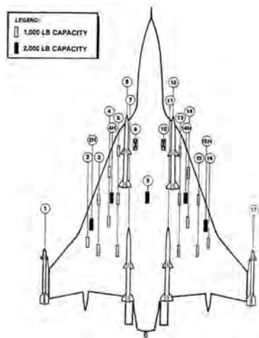
The F-16XL could carry a range of external stores at 29 different locations on the airframe. (USAF)
