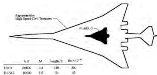
Comparison of the F-16XL with the proposed HSCT. (NASA)
