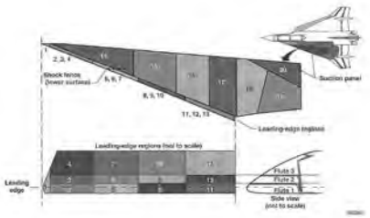
There were 20 separate suction regions on the F-16XL-2 wing glove, and different suction levels could be applied to each region. (NASA)
