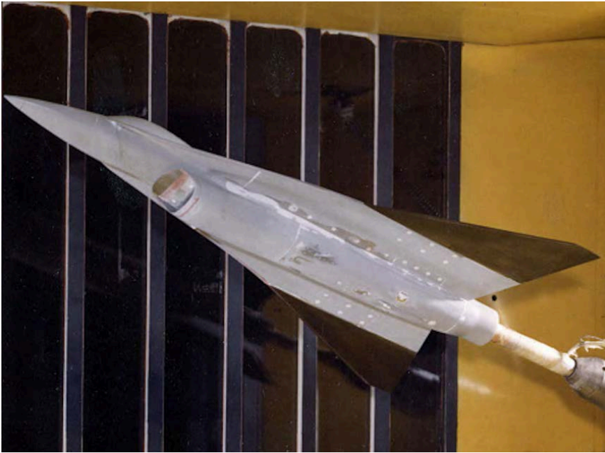
Test model of an interim SCAMP concept mounted in the NASA Langley Unitary Plan Wind Tunnel in 1978. (NASA)
