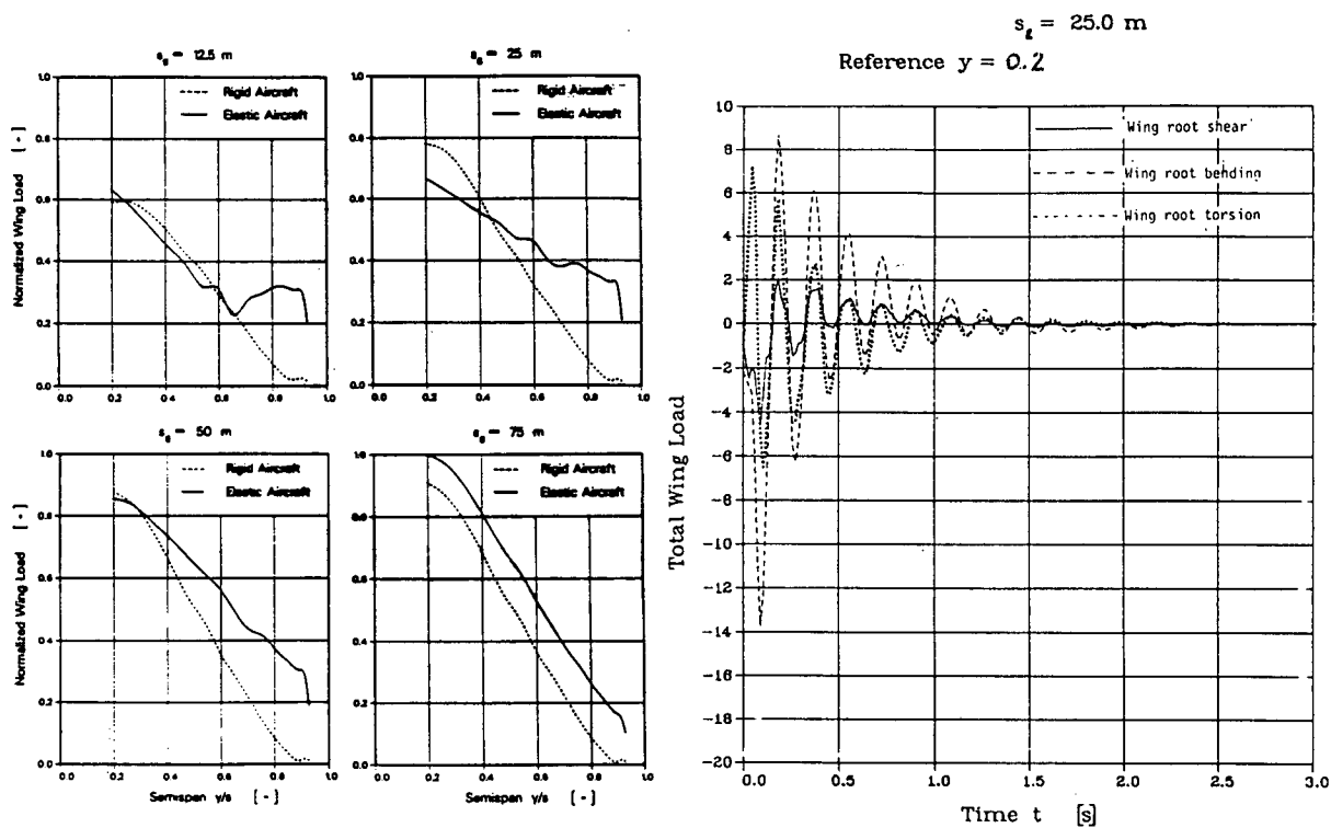
FIG. 9a DESIGN GUST CALCULATION: WING SHEAR FORCE
