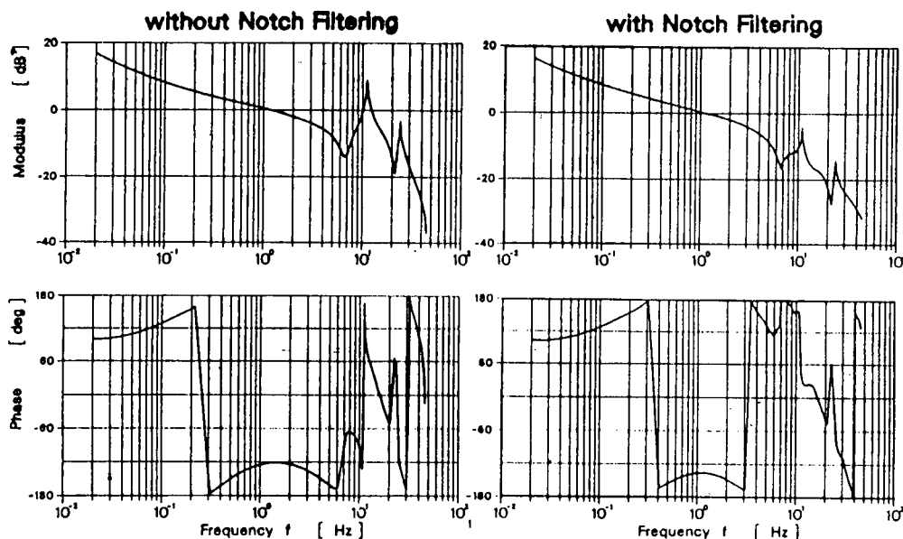
FIG. 14 BODE DIAGRAM OF OPEN LOOP PITCH RATE EFFECT OF NOTCH FILTERING
