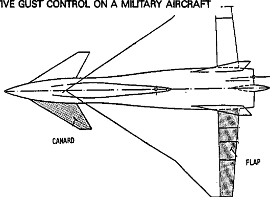
CANARD AND FLAP-ACTUATION FOR THE RIDE IMPROVEMENT SYSTEM ON A DELTA CONFIGURATION
