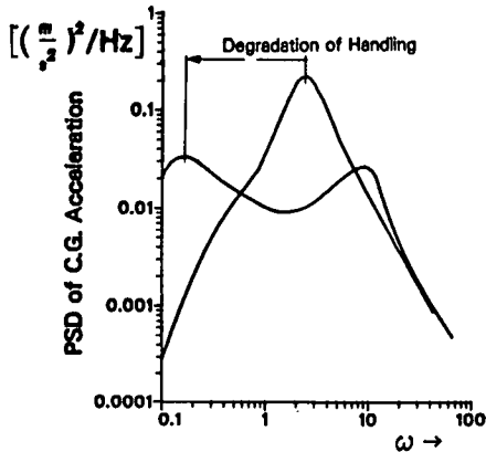
FIG. 22 EFFECT OF A RIDE IMPROVEMENT SYSTEM ON A TRANSPORT AIRCRAFT
