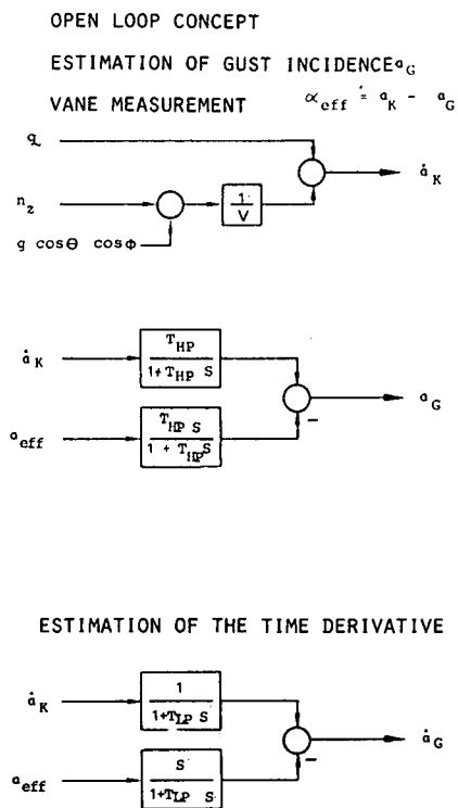
FIG. 17 DERIVATION OF GUST INCIDENCE BY VANE MEASUREMENT
