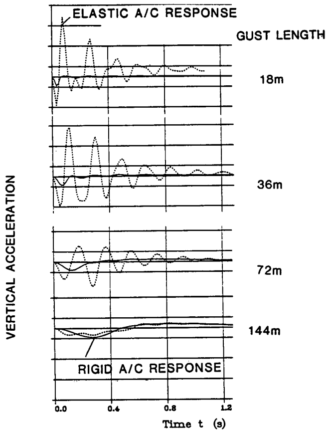
FIG. 8 DISCRETE GUST ANALYSIS: ACCELERATION AT MISSILE NOSE
