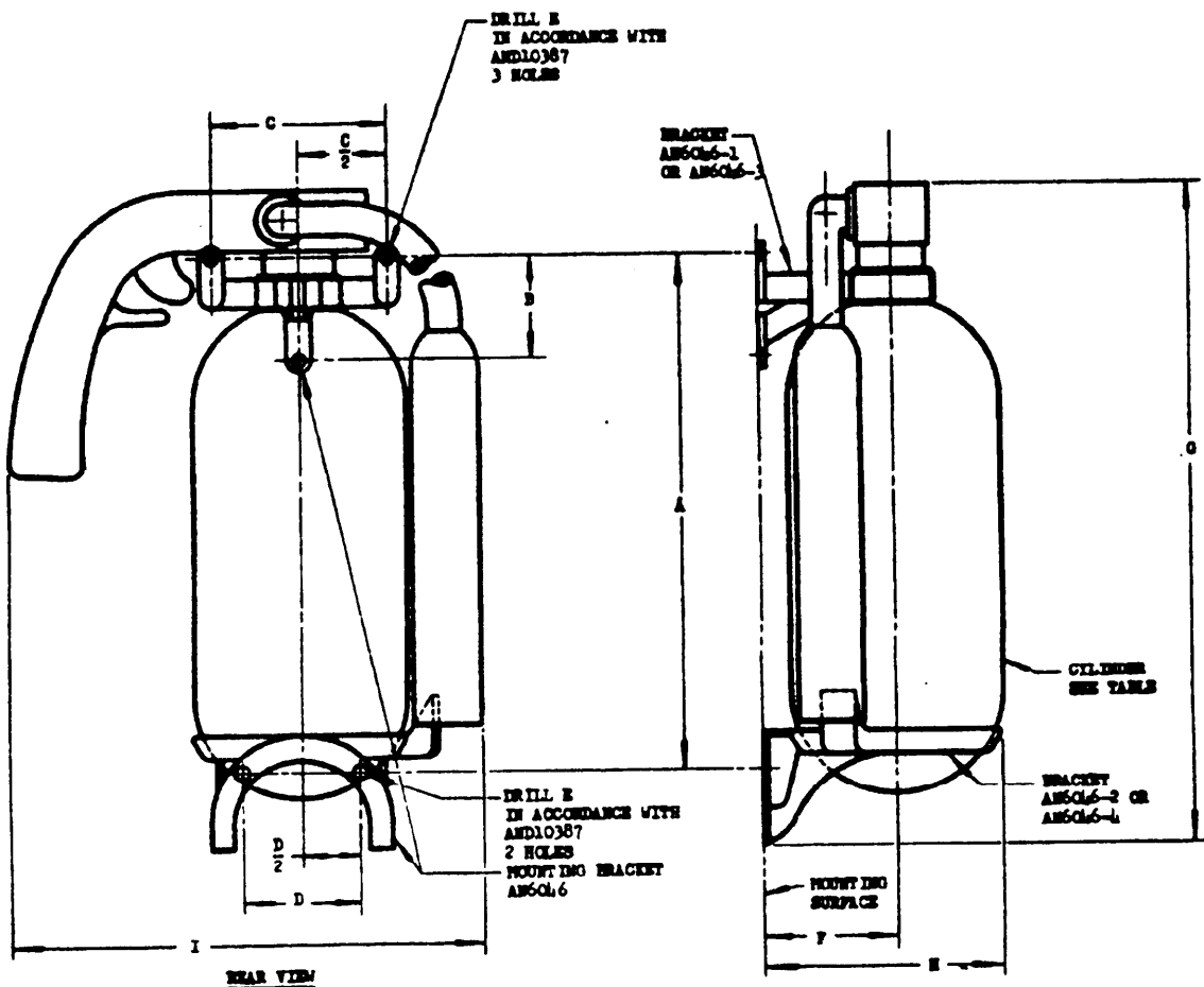
REAR VIEW
