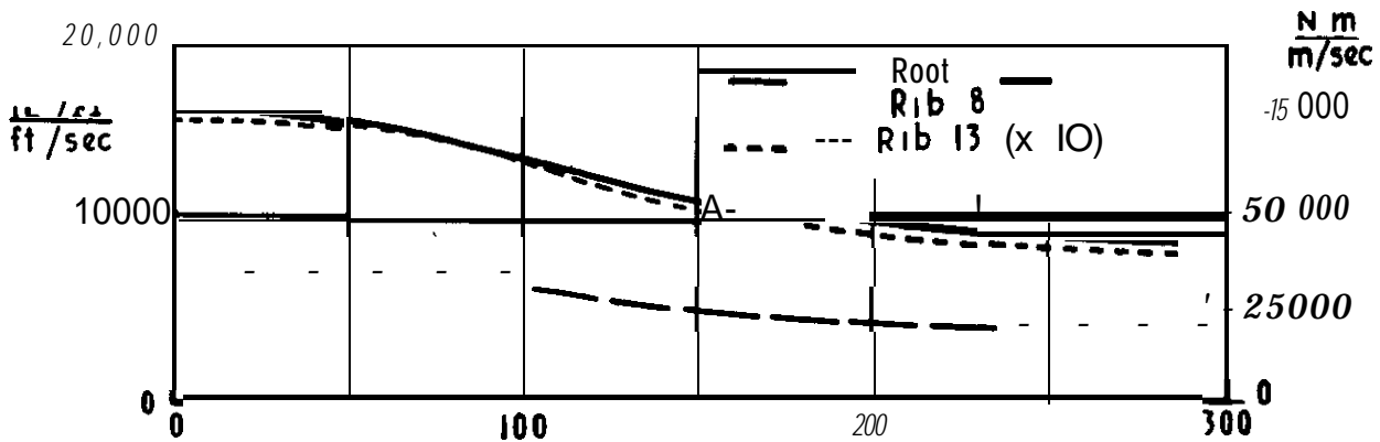
Wing bending moments
