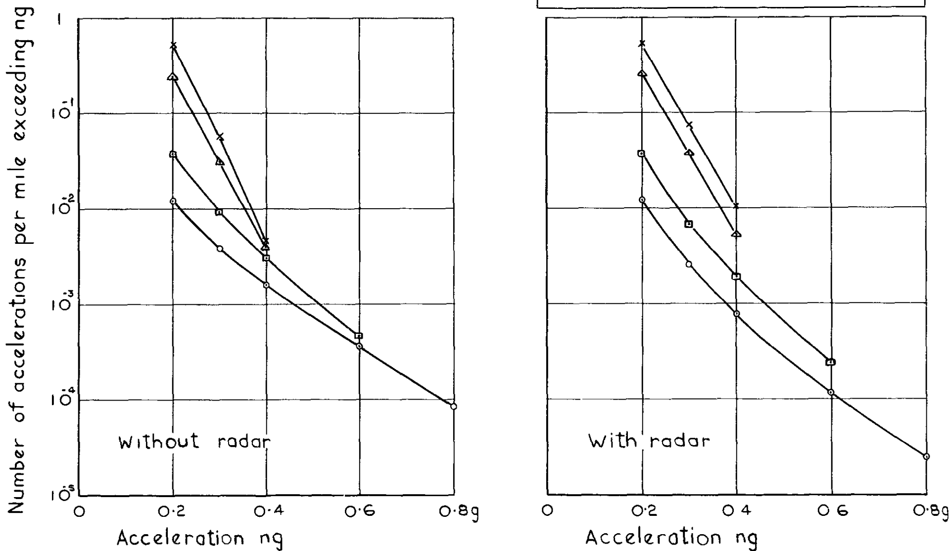
Fig.3 Accelerations experienced without and with radar
