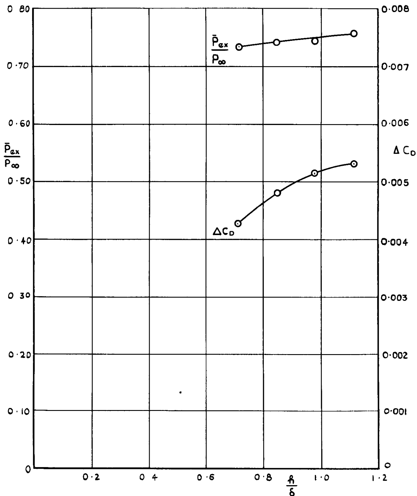
Fig 17 Variation of pressure recovery and \Delta C_D with boundary layer diverter height at zero incidence; \frac{A_{\infty}}{A_{en}} \approx 0.93
