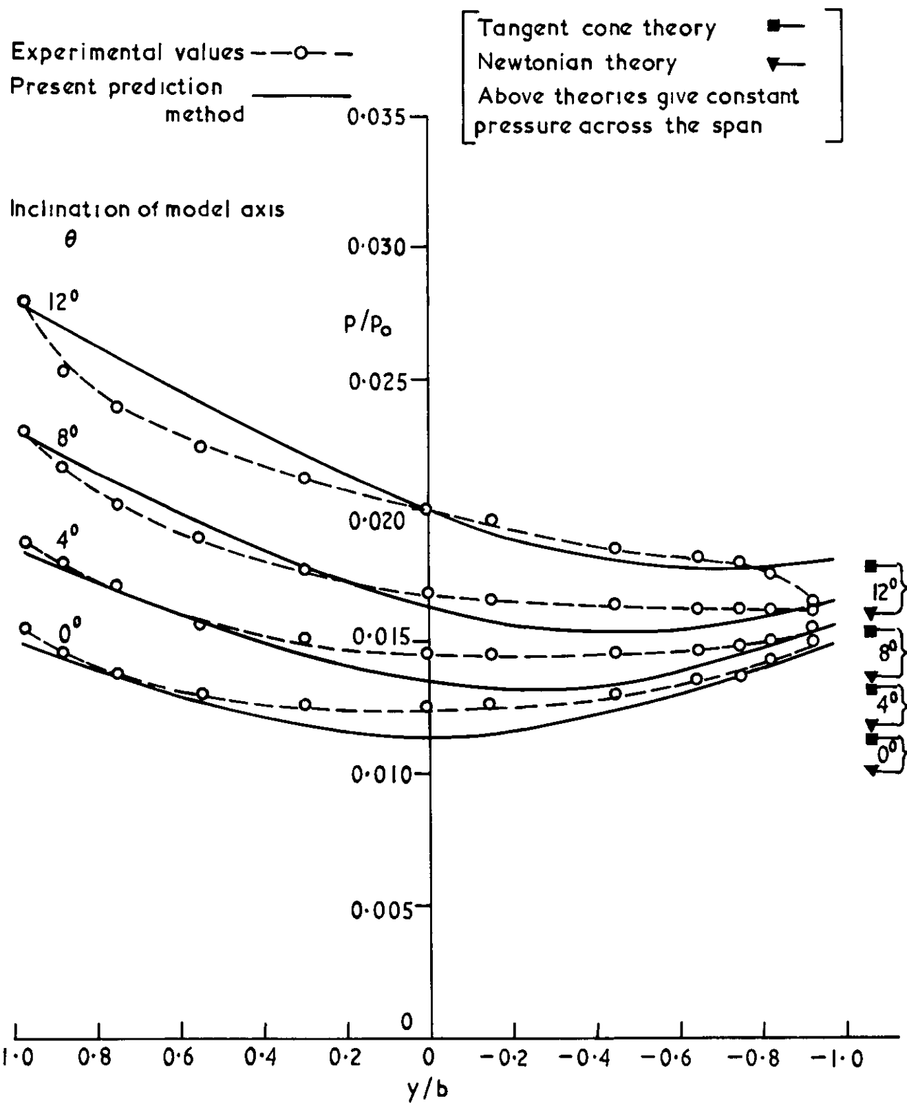
Comparison of experimental pressure distributions with the predicted values (Eqn.2) for the lower surface of the NPL model
