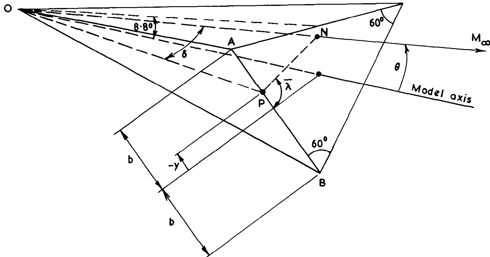
Definition of angles \lambda and \delta and details of NPL model
