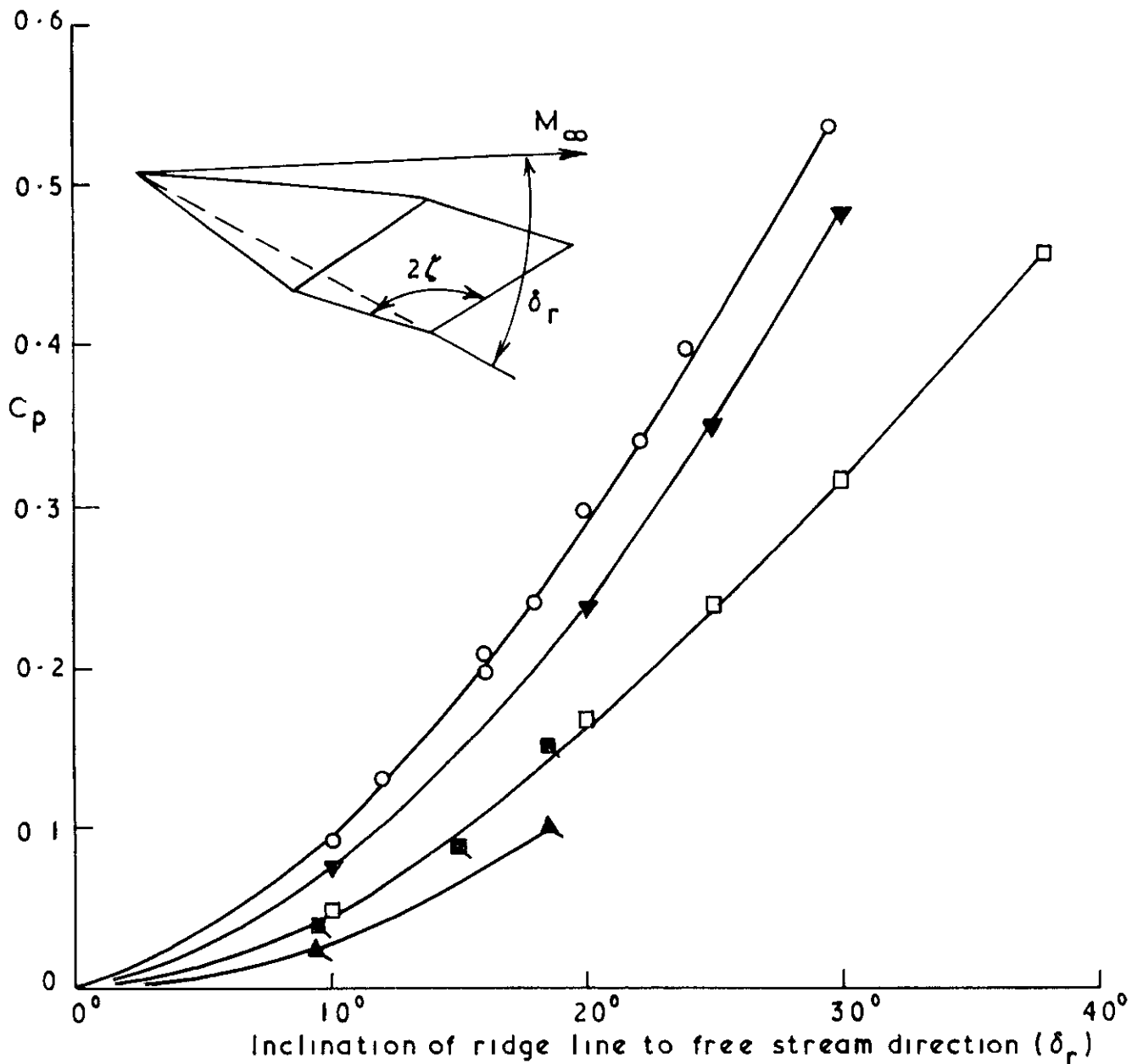
Pressure coefficient at ridge line on low aspect-ratio conical bodies at M_\infty = 4
