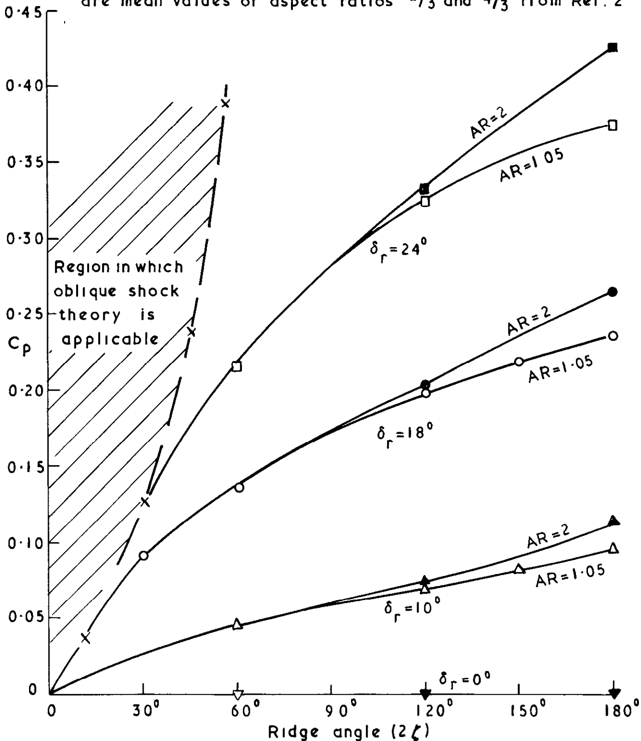
Effects of aspect-ratio on the variation of pressure coefficient at ridge line with ridge angle at M_\infty = 4
