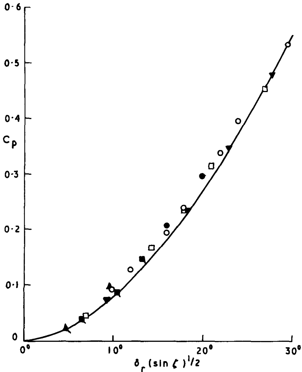
Correlation of pressure coefficient at ridge line of conical bodies at M_\infty = 4
