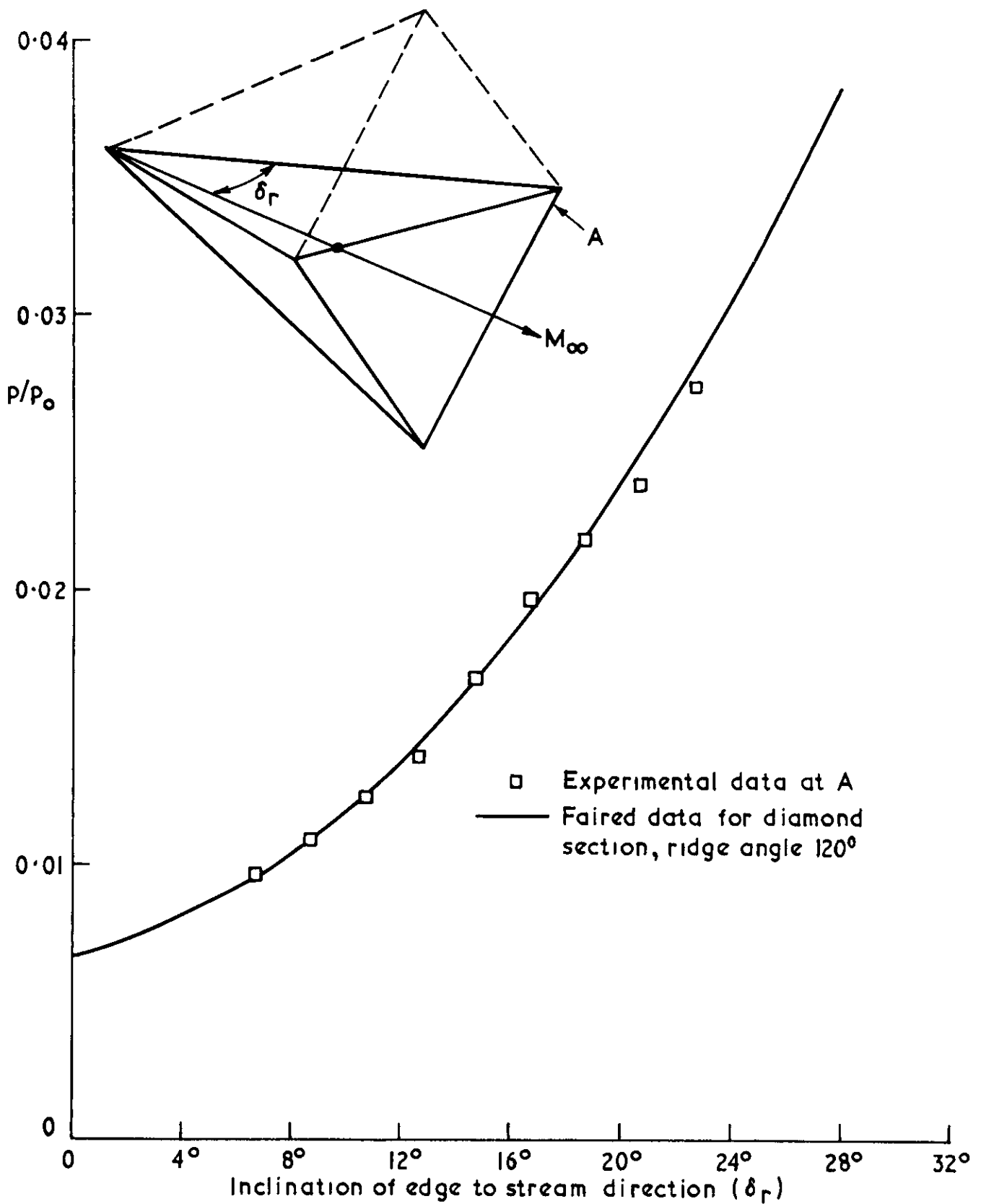
Comparison of pressures at leading edge of triangular section and at ridge line of diamond section ( M_\infty = 4 )
