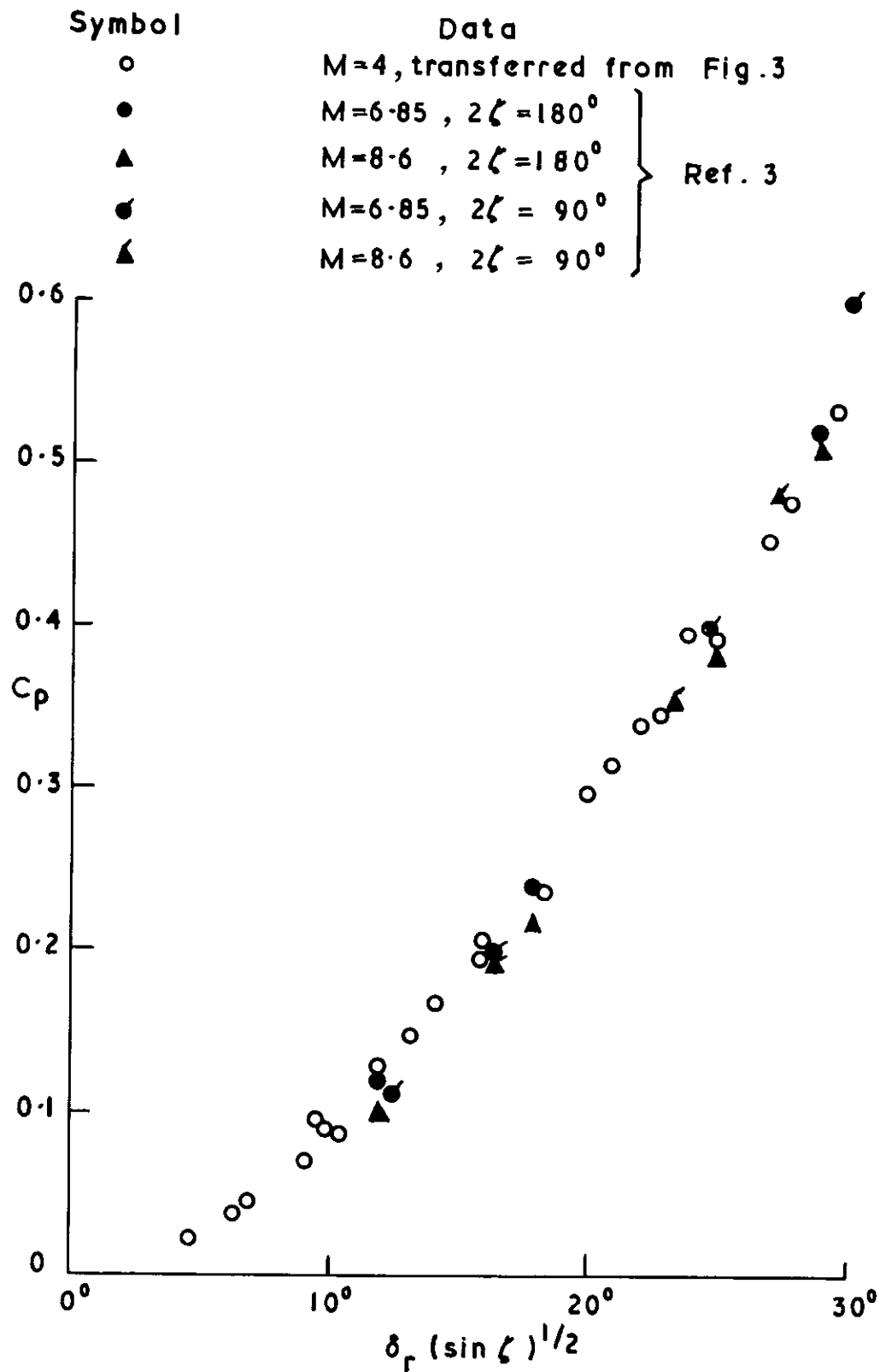
Effects of free stream Mach number on pressure coefficient at ridge line
