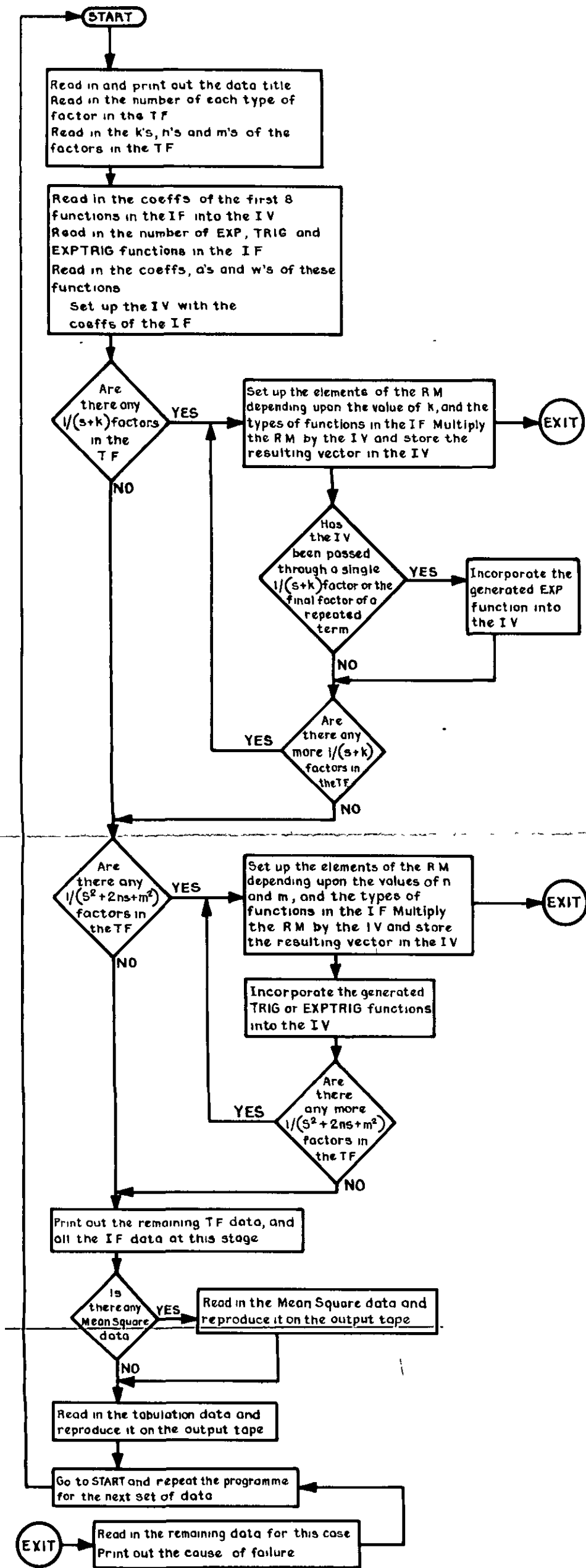
Fig. 1 Flow diagram for Programme 1: Tapes 1 and 2
