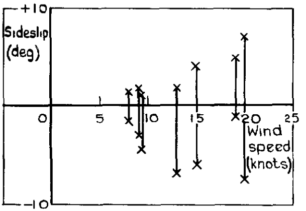
Fig. 5 a & b Maximum amplitudes of rudder and aileron angles, bank and sideslip during approach as functions of crosswind and total wind speed
