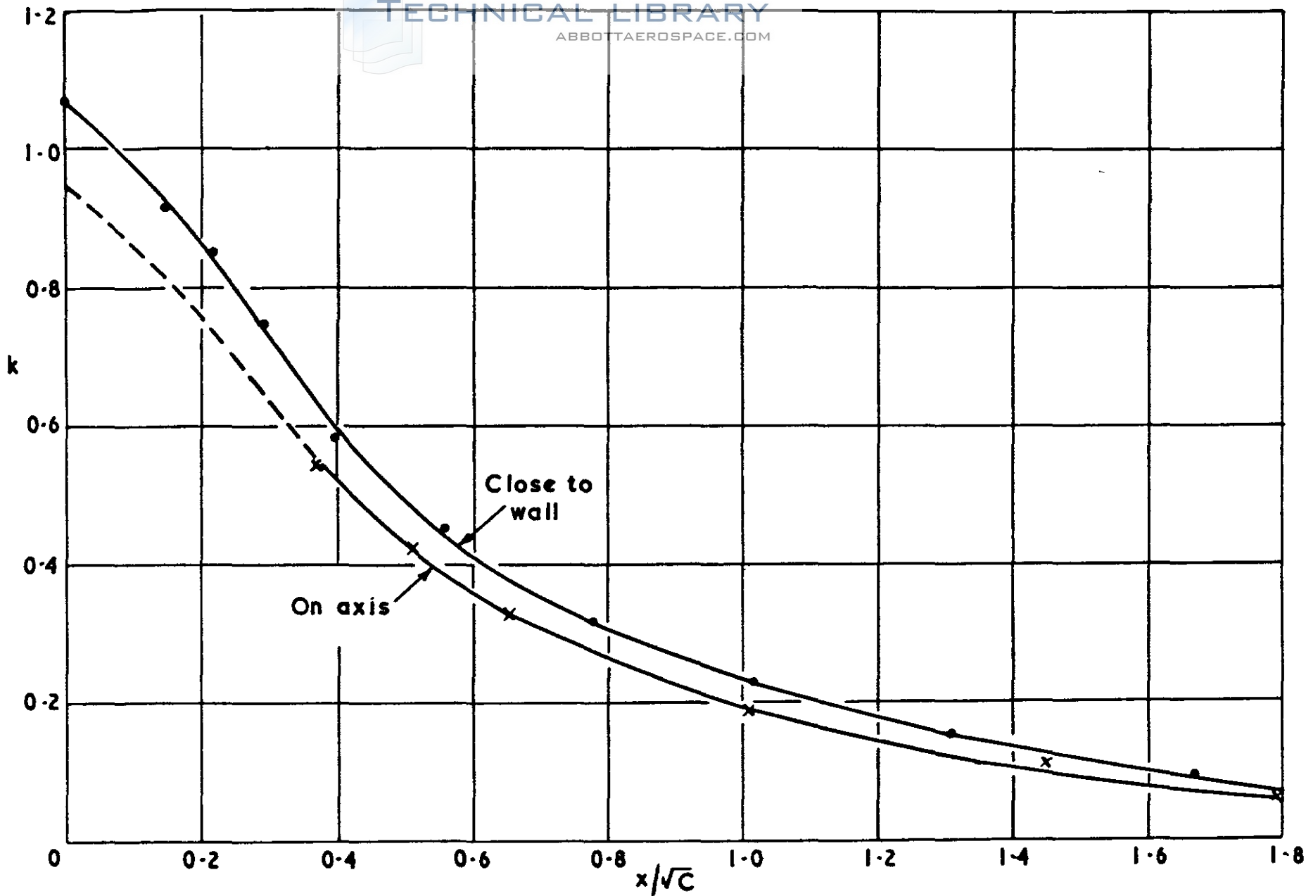
Blockage constants for cylindrical stem of pitot-static tube affecting static pressure measured (a) at tube (b) at wall static tapping
