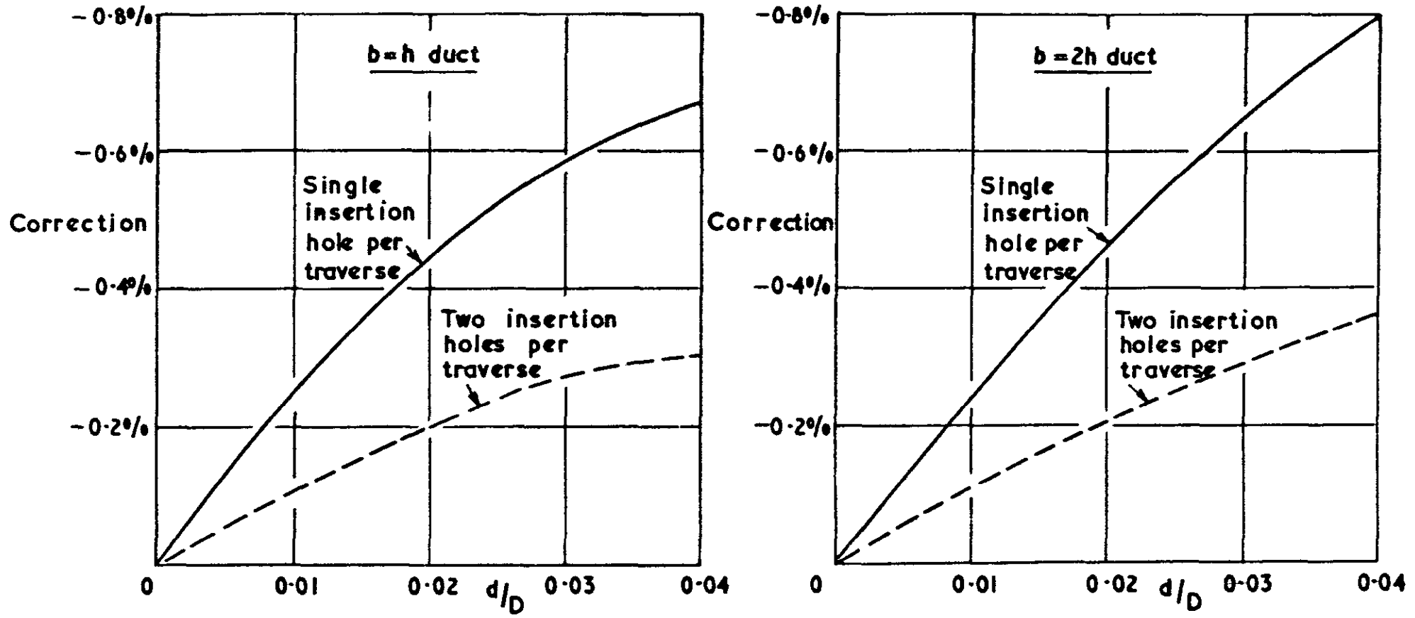
Pitot-stem blockage corrections to volume flow rate measured in rectangular ducts with an x=8d pitot tube using the 26point log-linear method. (Stem parallel to side h)
