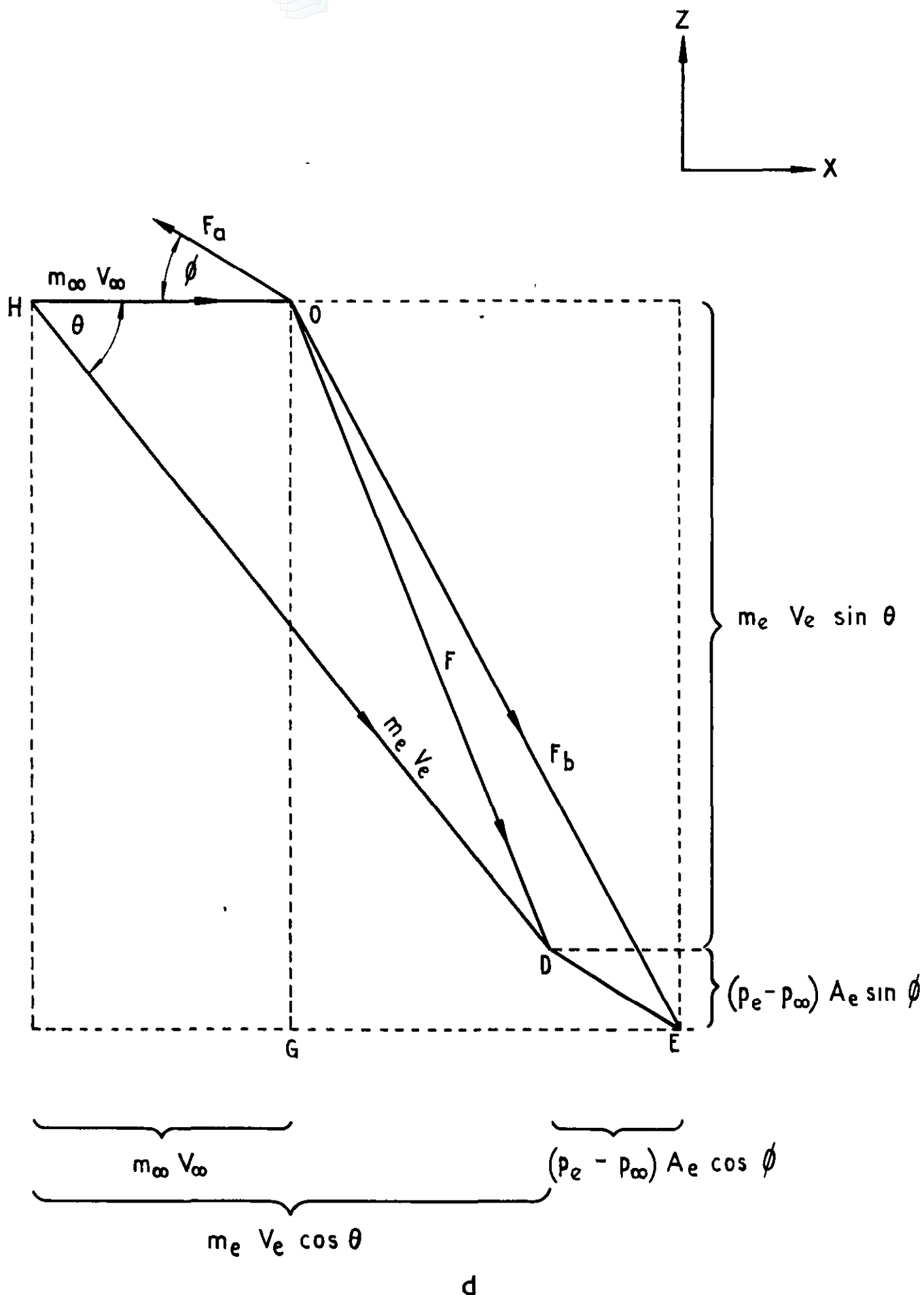
Fig3contd Development of vector diagram appropriate to Fig 1a pressures measured relative to undisturbed static pressure ( p_\infty )
