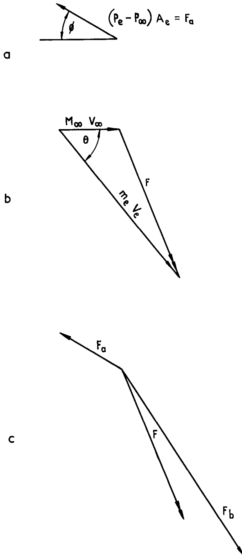
Fig.3a-c Development of vector diagram appropriate to Fig.1a pressures measured relative to undisturbed static pressure ( p_{\infty} )
