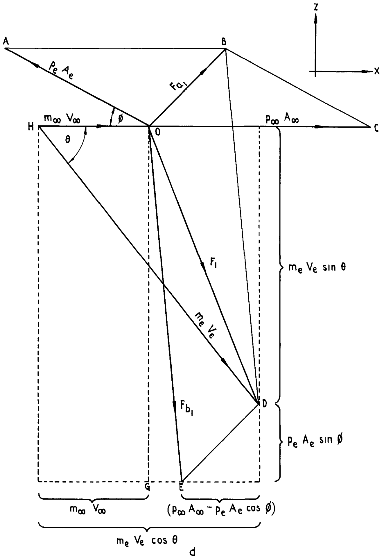
Fig 2 contd Development of vector diagram appropriate to Fig 1a—absolute pressures
