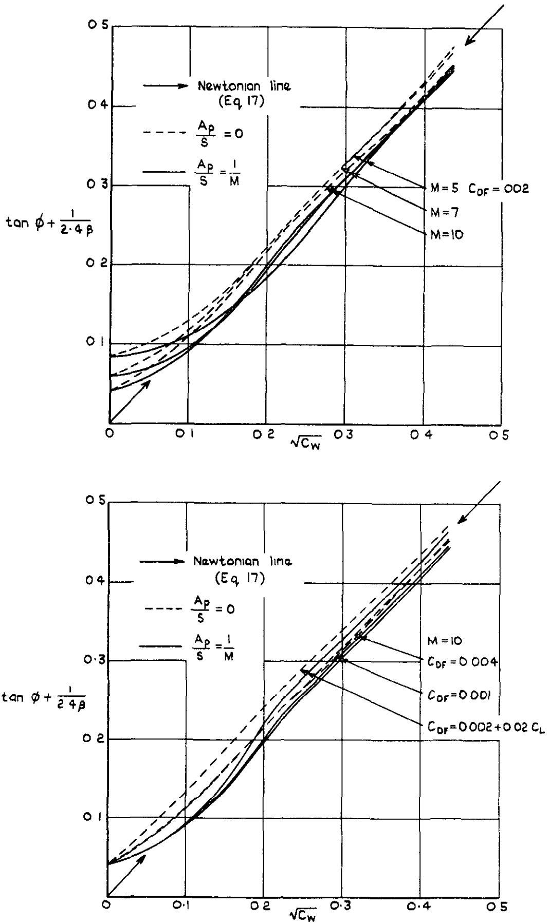
Fig.13 Collapsed plots of \phi values
