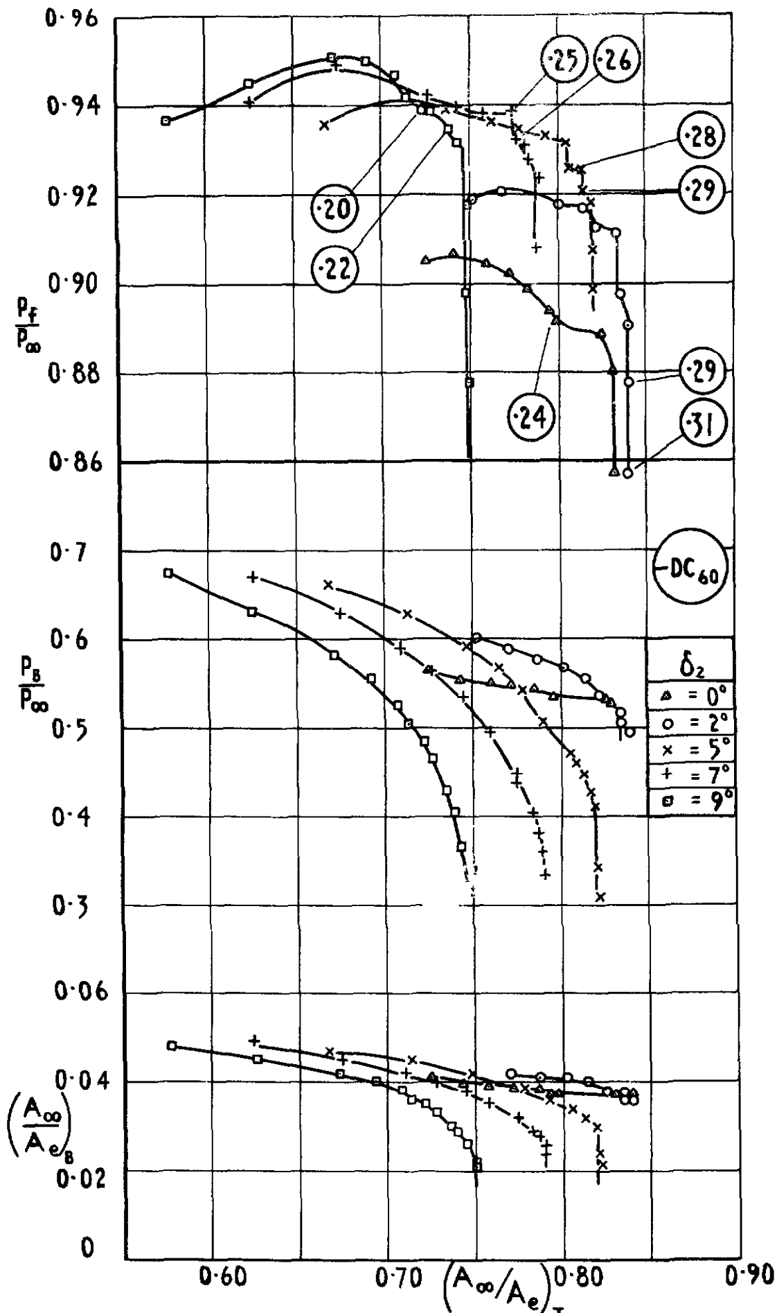
Fig.20 Variation of engine face pressure recovery, bleed pressure recovery and bleed mass flow with total mass flow. Bleed exit plug 4. M_\infty 1.80
