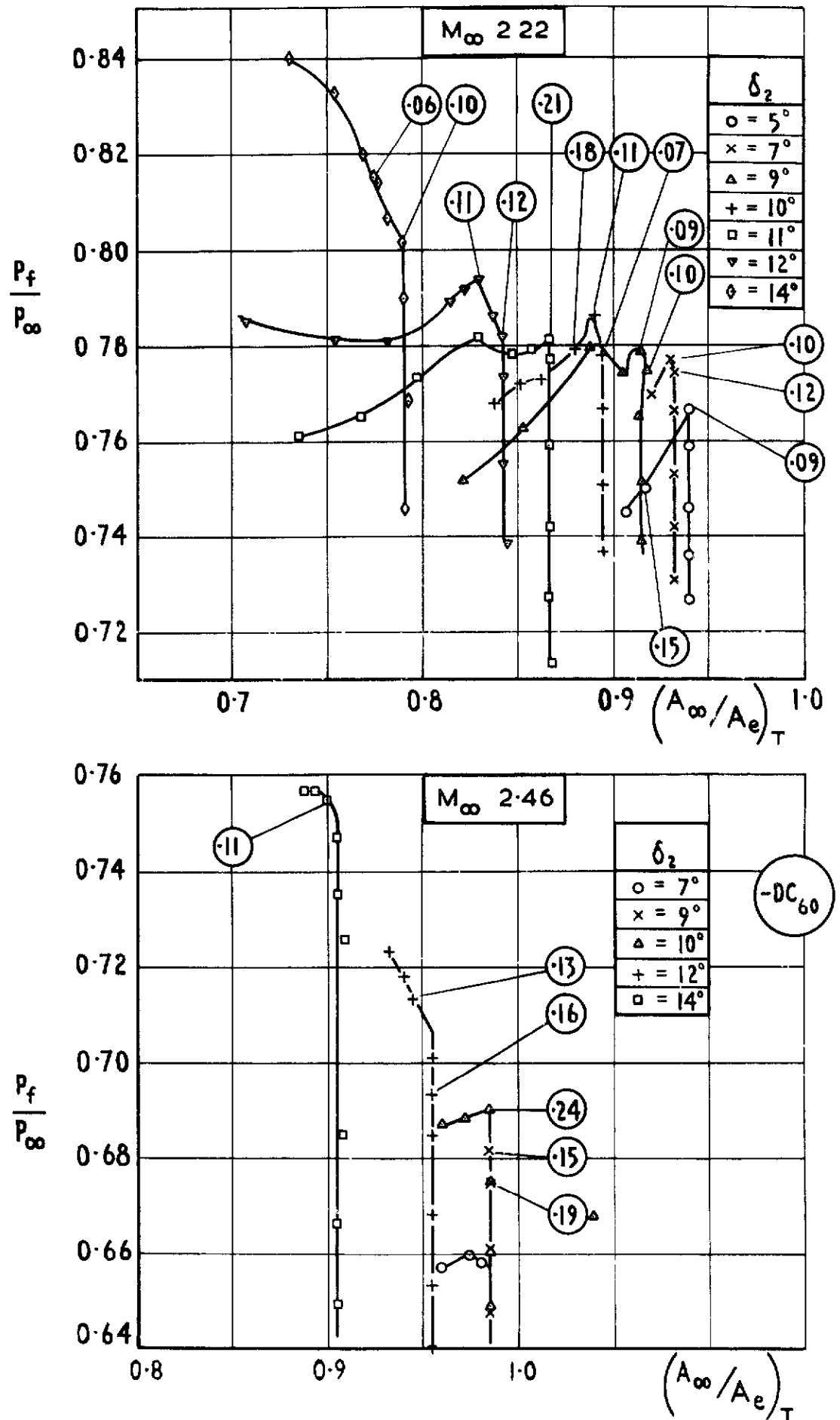
Fig9 Variation of pressure recovery with mass flow. Zero bleed. M_\infty 2.22 and 2.46
