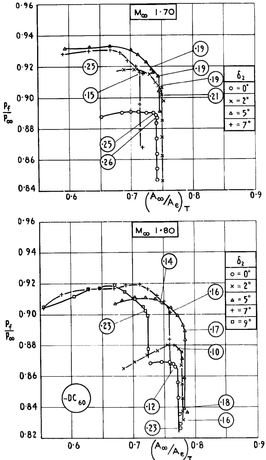
Fig.11 Variation of pressure recovery with mass flow Zero bleed. M_{\infty} 1.70 and 1.80
