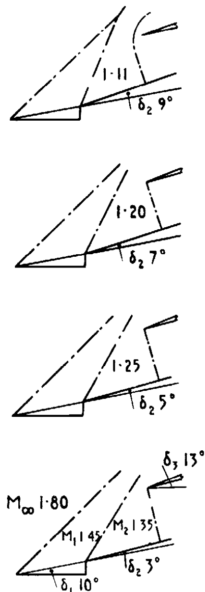
Fig 33 Variation of critical pressure recovery and maximum mass flow with \delta_2 at constant bleed flow. M_\infty 1.80
