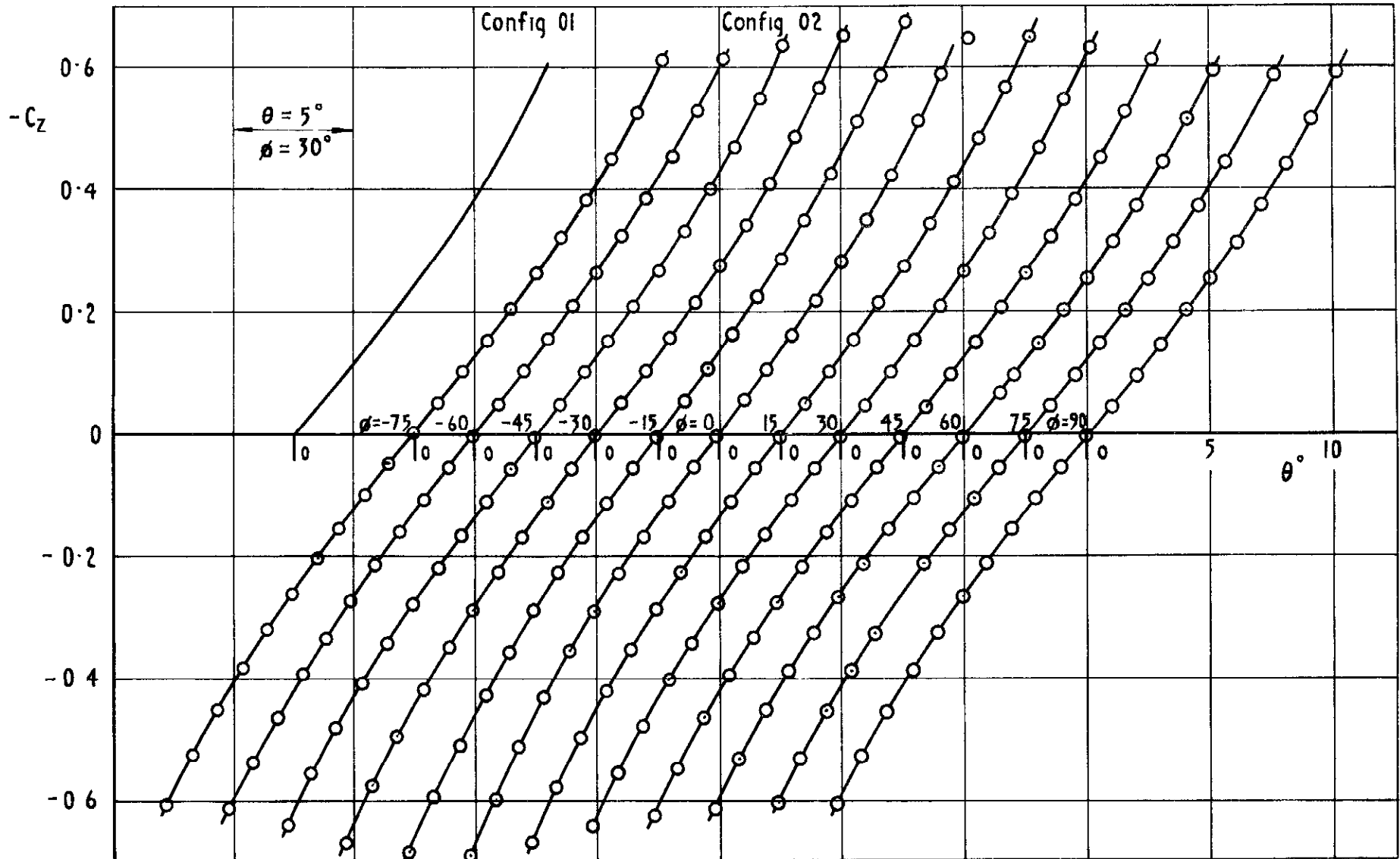
Fig.8 Variation of normal force with incidence and roll M = 2.0 \quad R_D = 1.31 \times 10^6
