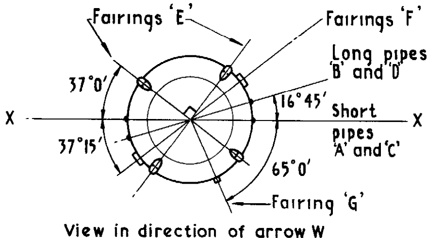
Fig2a General arrangement of the model
