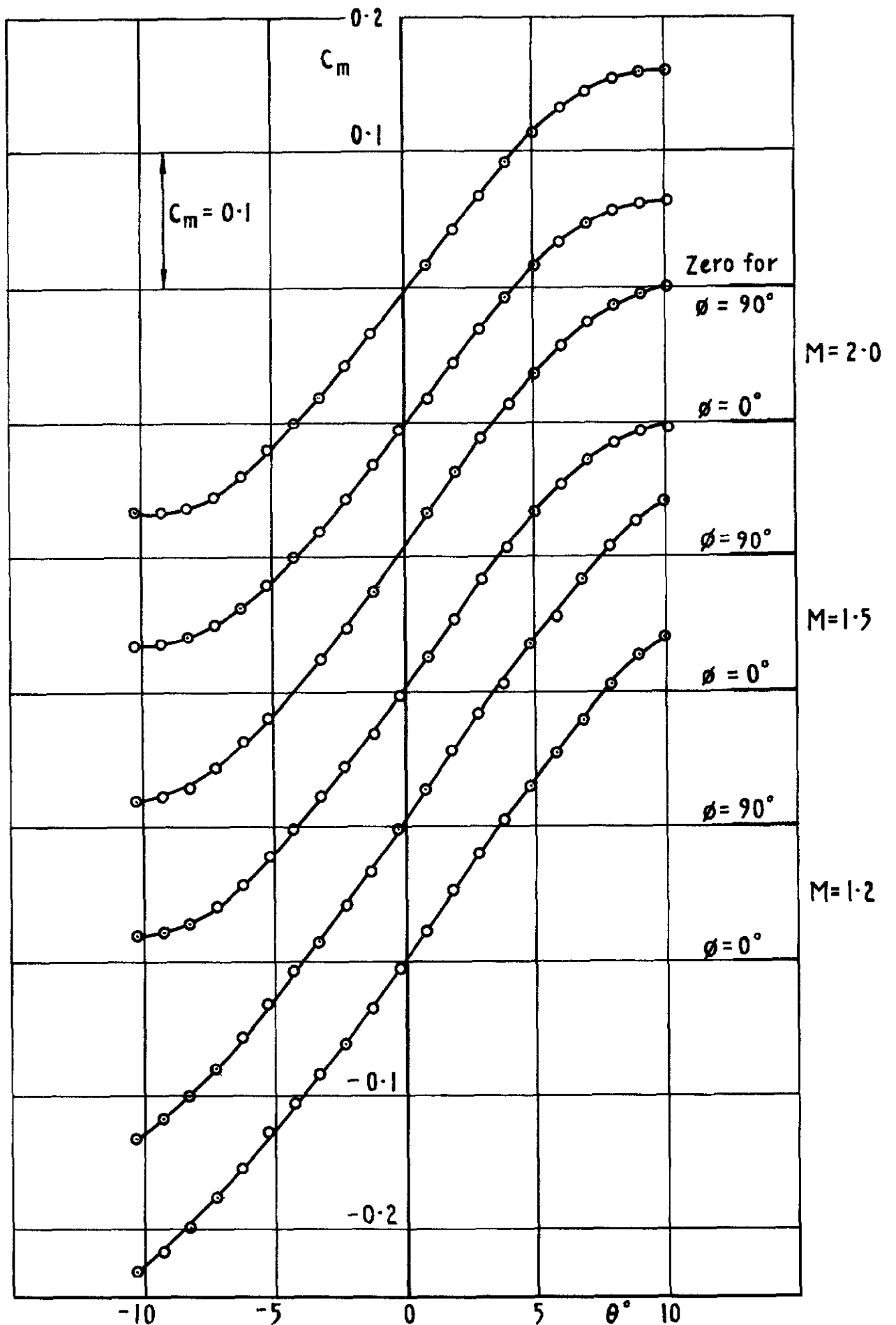
Fig 10 Variation of pitching moment with incidence and roll Config 01 R_D = 1.31 \times 10^6
