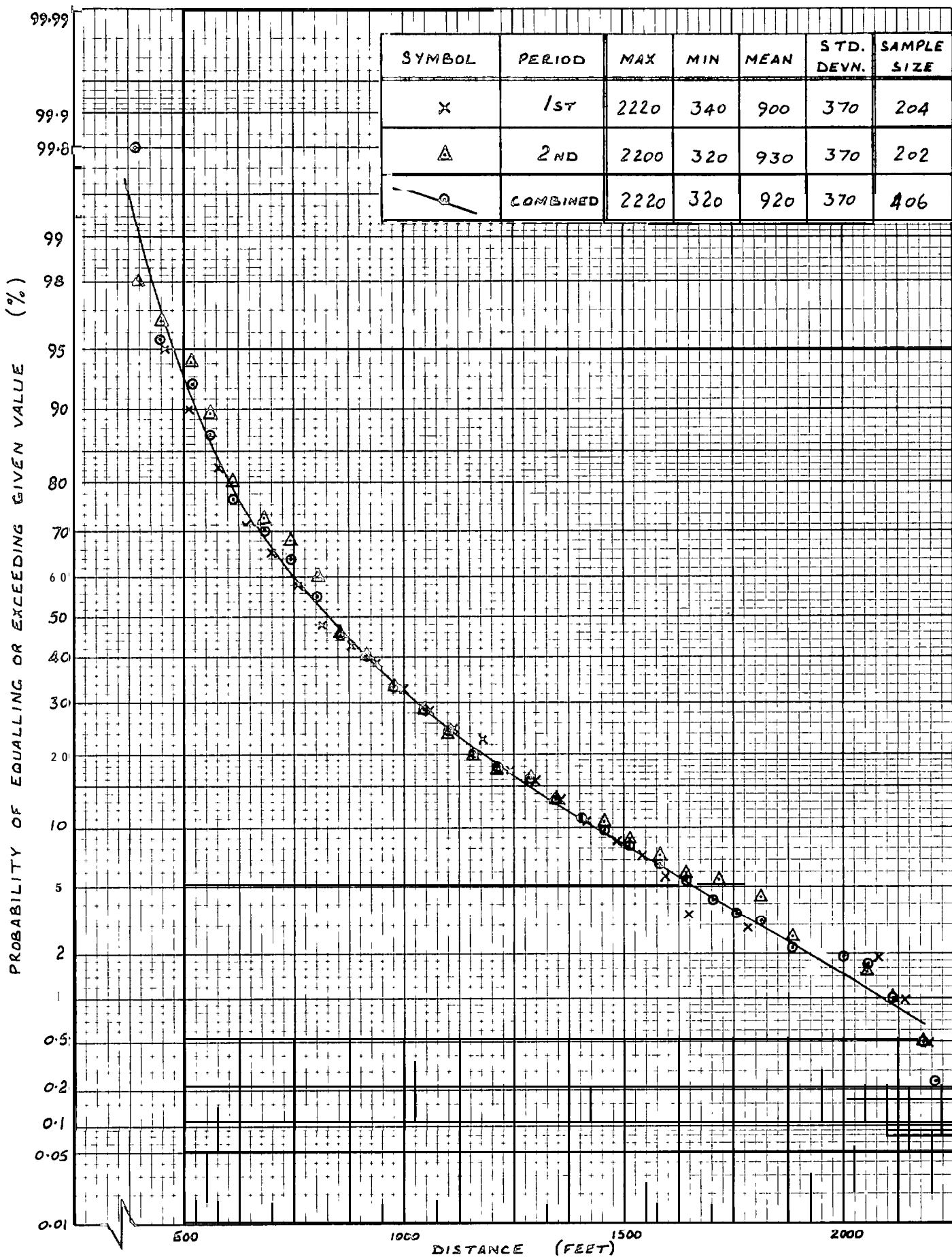
Fig.20 Distance travelled from first impact to nosewheel impact Aircraft Type D 1
