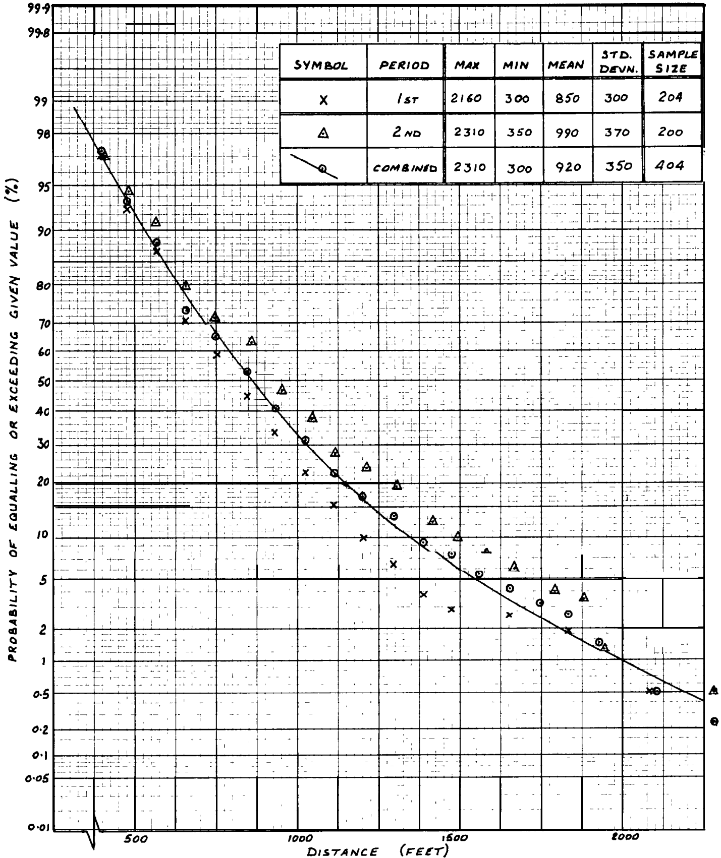
Fig.41 Distance travelled from first impact to nosewheel impact Aircraft Type E 1
