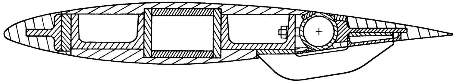
Typical section
