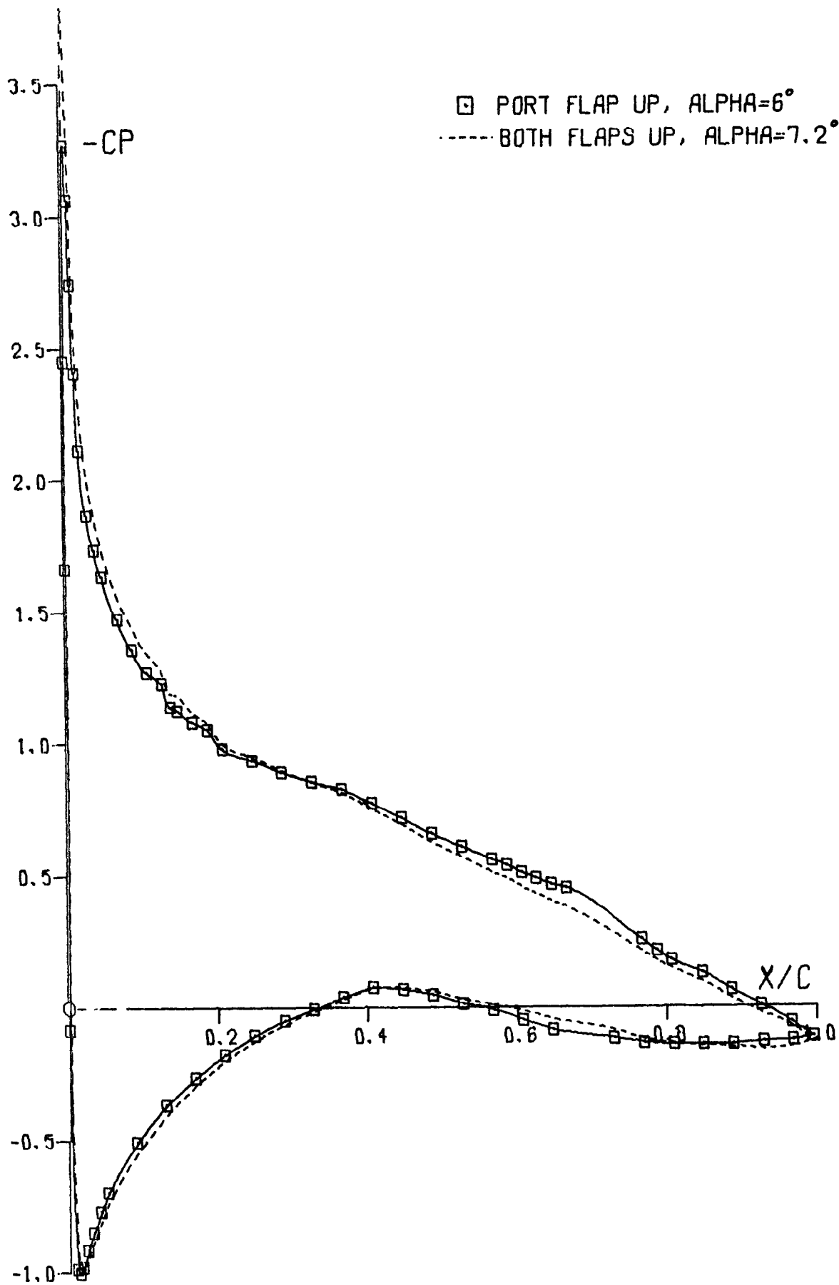
Fig.18 Pressure distributions at a port station with flap up. Row 11, C_N = 0.841
