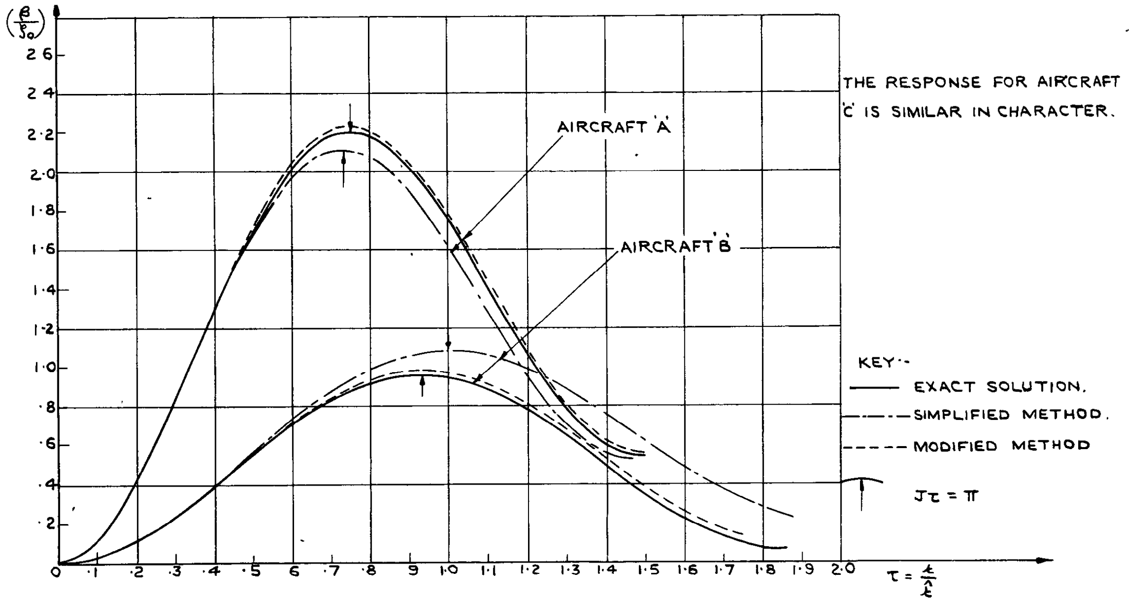
FIG I. RESPONSE TO AN INSTANTANEOUS RUDDER DEFLECTION \delta_0
