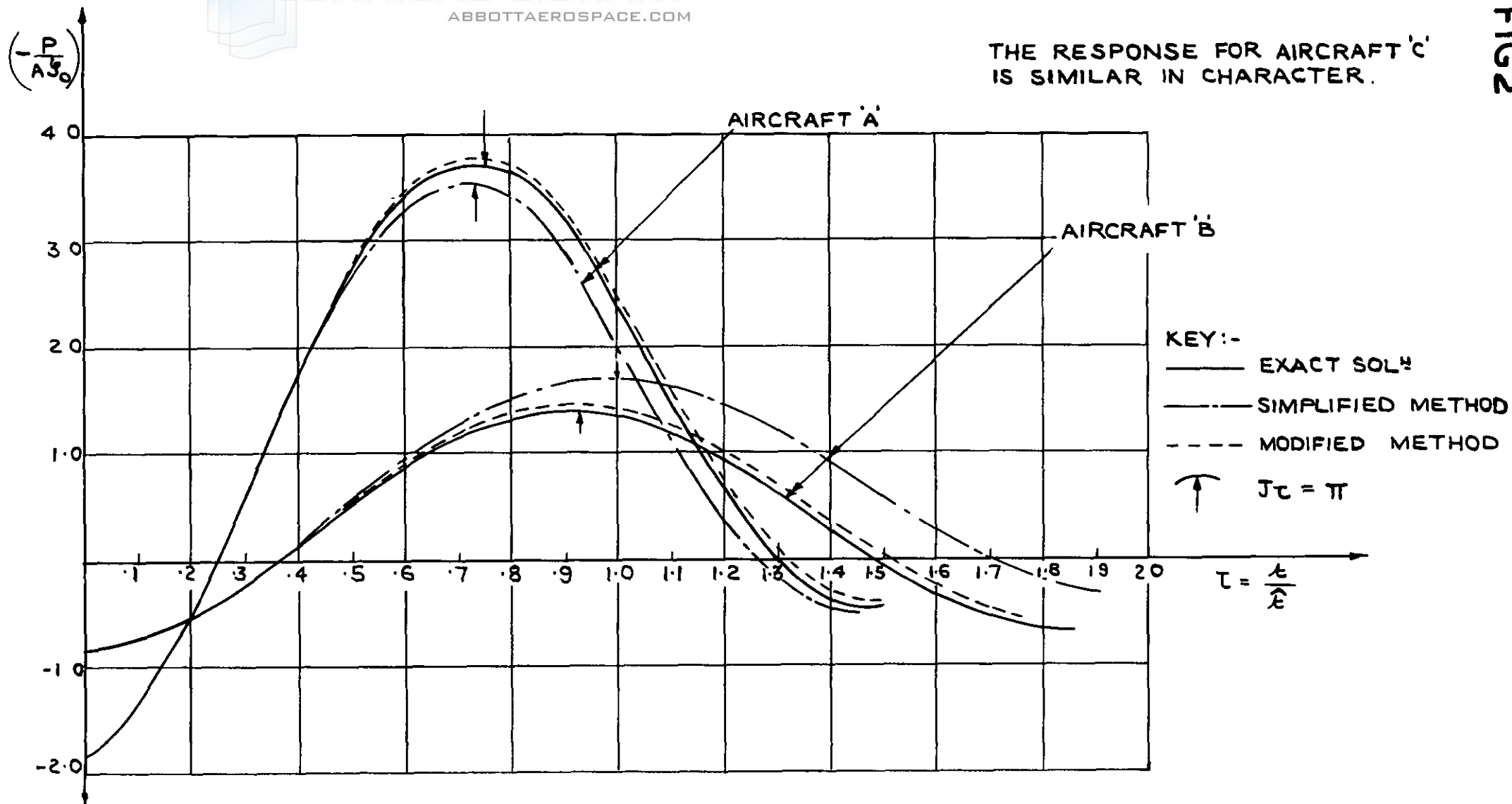
FIG 2. TIME HISTORY OF FIN & RUDDER LOADS AFTER AN INSTANTANEOUS RUDDER DEFLECTION \beta_0
