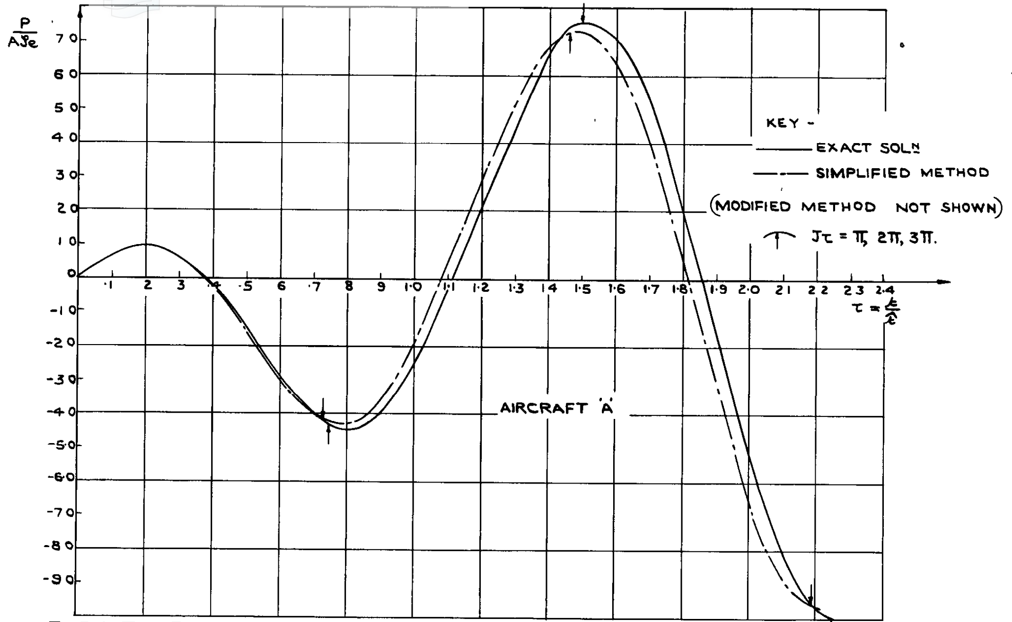
FIG. 4. TIME HISTORY OF FIN & RUDDER LOADS PRODUCED BY A SINUSOIDAL RUDDER DEFLECTION \delta = \delta_e \sin J\tau .
