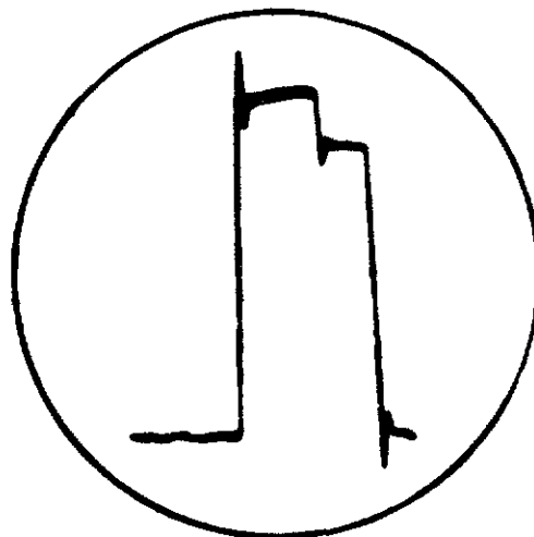
(f) RESONANCE BETWEEN ROTARY VALVE AND PICK-UP.
