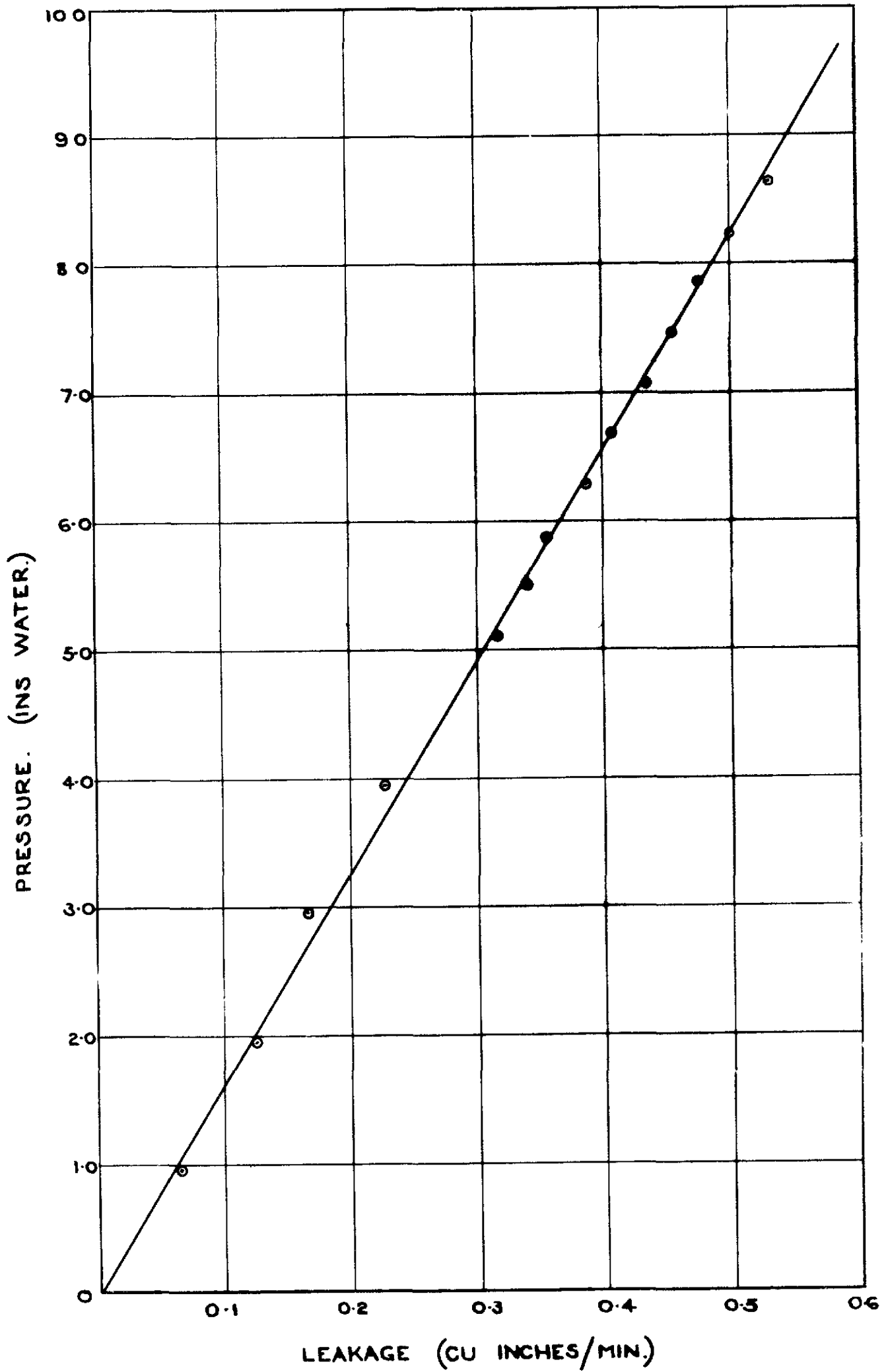
LEAKAGE THROUGH ROTARY VALVE.
