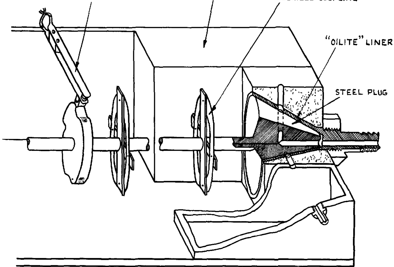
ROTARY VALVE (SCALE - \frac{3}{4} FULL SIZE)
