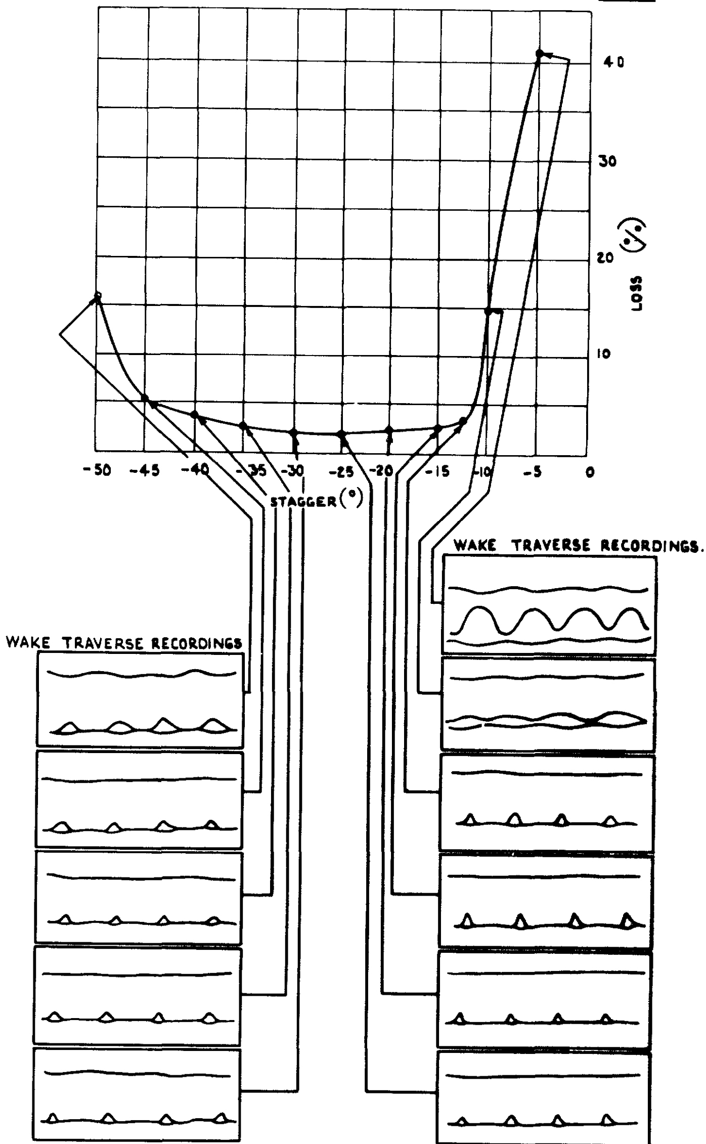
TYPICAL LOSS VARIATION WITH STAGGER FOR COMPRESSOR CASCADE.
