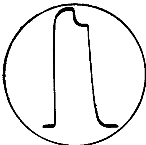
(e) EXCESSIVE RESTRICTION BETWEEN ROTARY VALVE, AND PICK-UP
