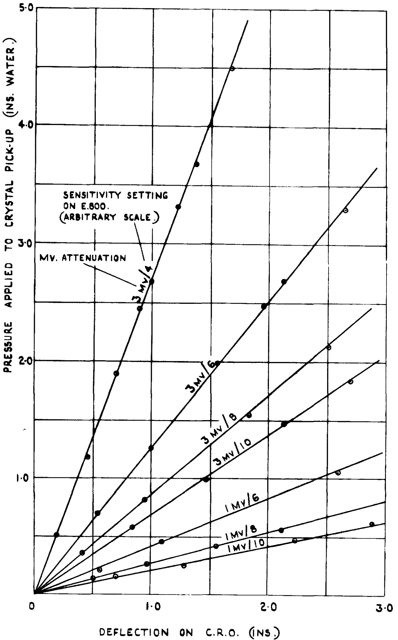
LINEARITY CURVES.
