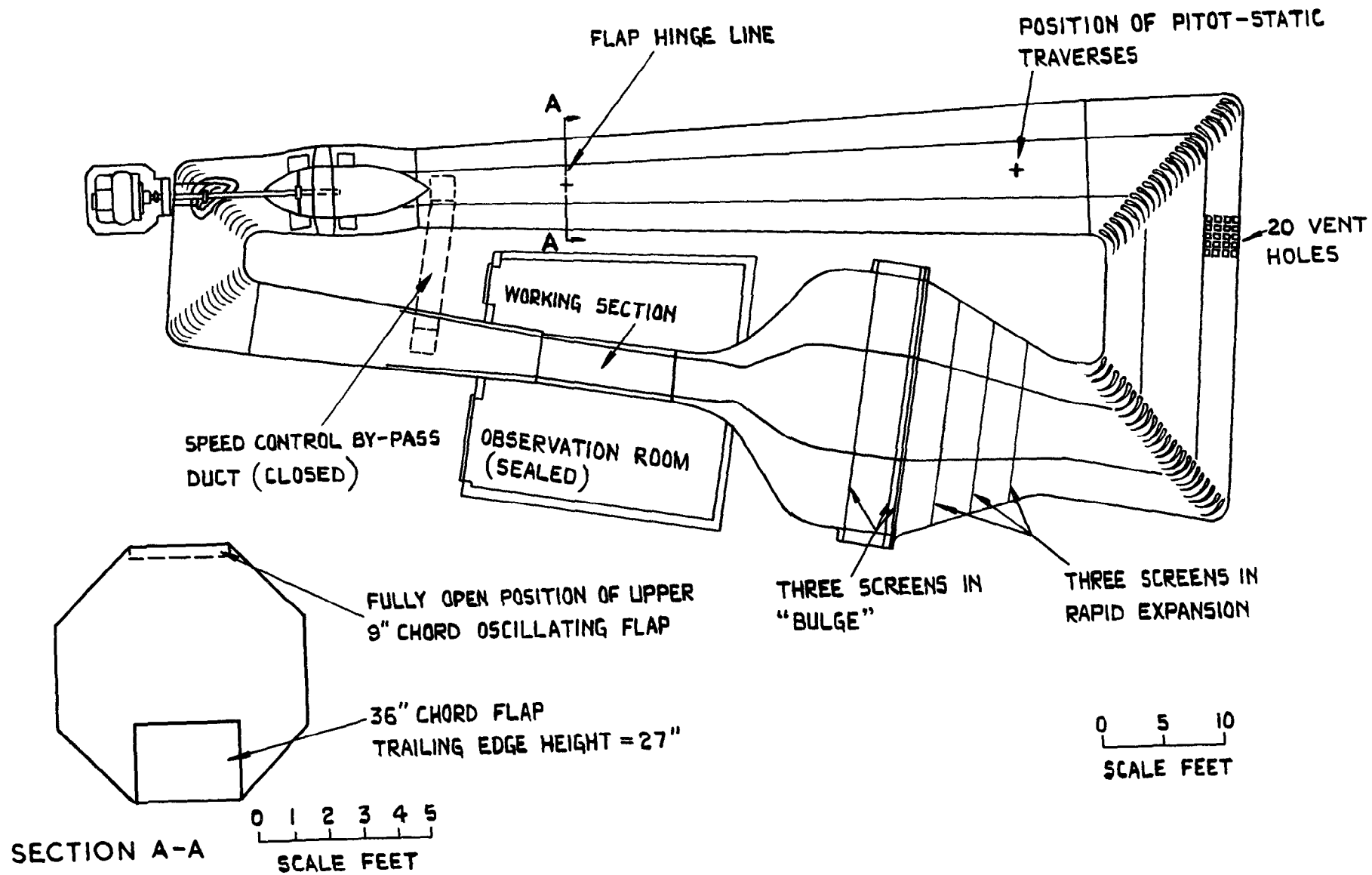
FIG. 1. 4' x 3' WIND TUNNEL PLAN VIEW ON CENTRE LINE.
