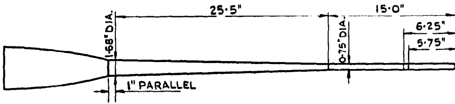
MODIFIED MK.IX HEAD, TEST VEHICLE G
