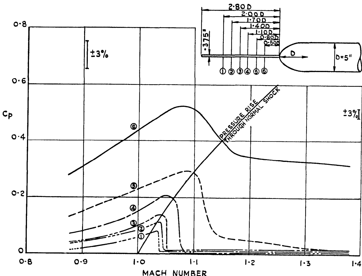
FIG.4. VARIATION OF PRESSURE COEFFICIENT ALONG PROBE AHEAD OF ELLIPSOIDAL NOSE (TEST VEHICLE B).
