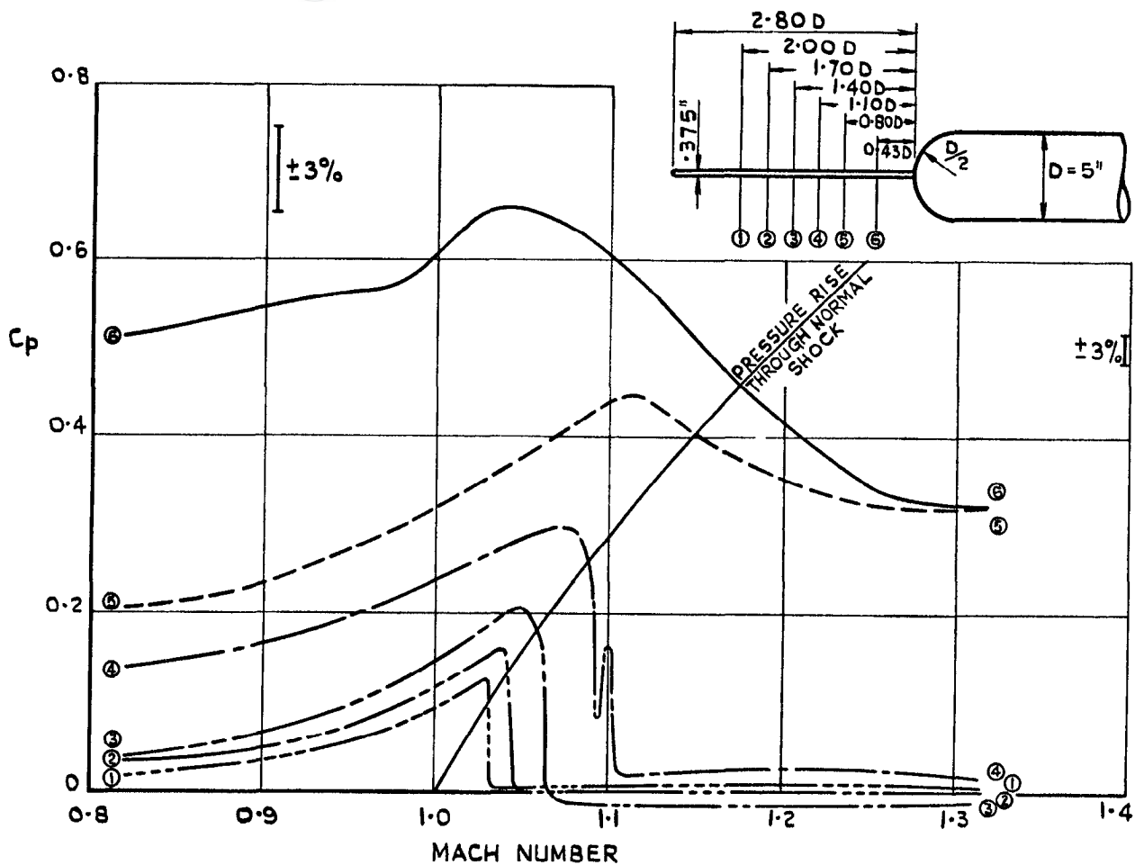
FIG.3. VARIATION OF PRESSURE COEFFICIENT ALONG PROBE AHEAD OF HEMISPHERICAL NOSE (TEST VEHICLE A).
