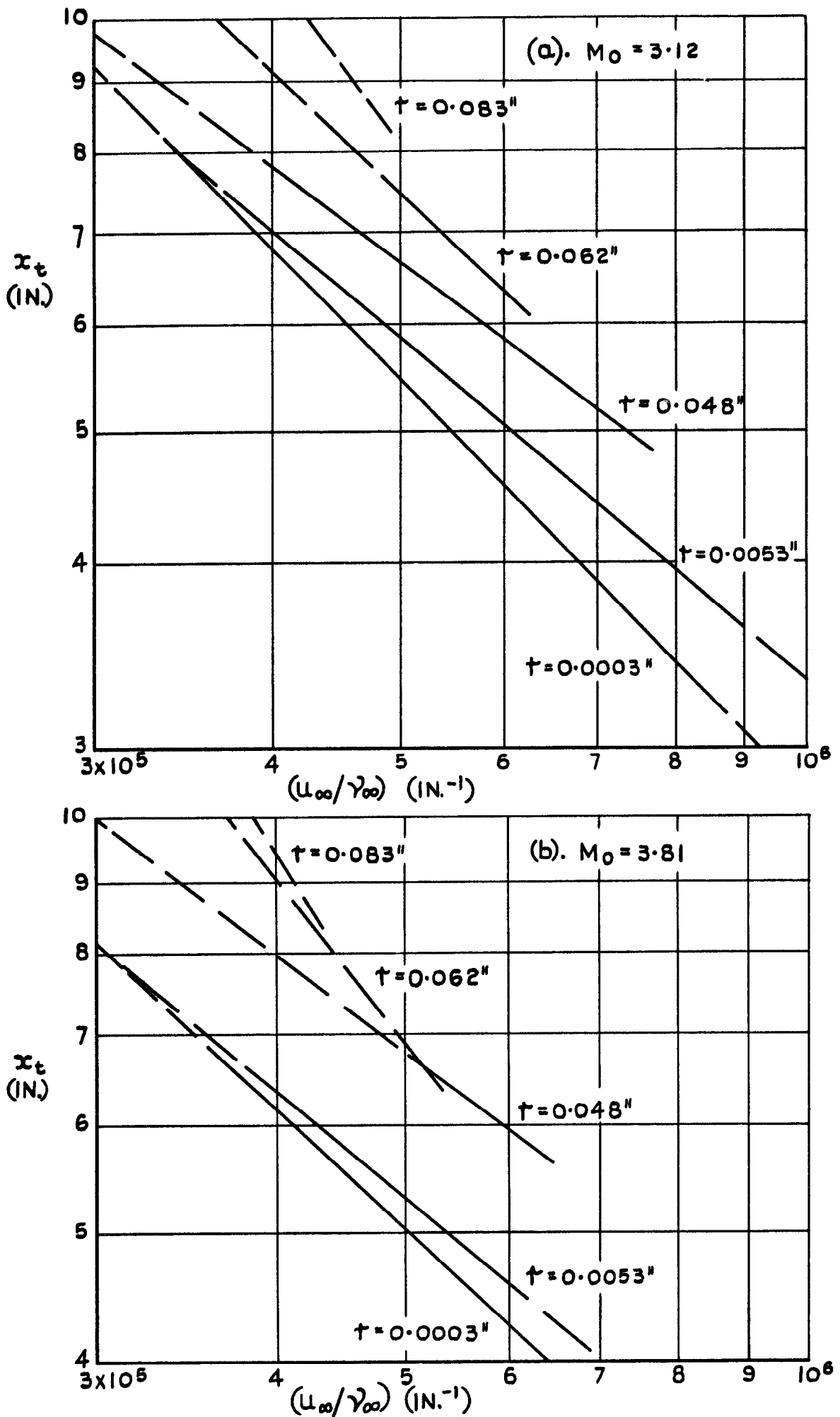
FIG.8. VARIATION OF TRANSITION POSITION, x_t , ON FIVE CONES WITH REYNOLDS NUMBER PER INCH, (u_o/\gamma_o) , FOR x_t > 100 \tau . (CURVES FAIRED AND EXTRAPOLATED FROM MEASURED VALUES). (a). M_0 = 3.12 , (b). M_0 = 3.81 .
