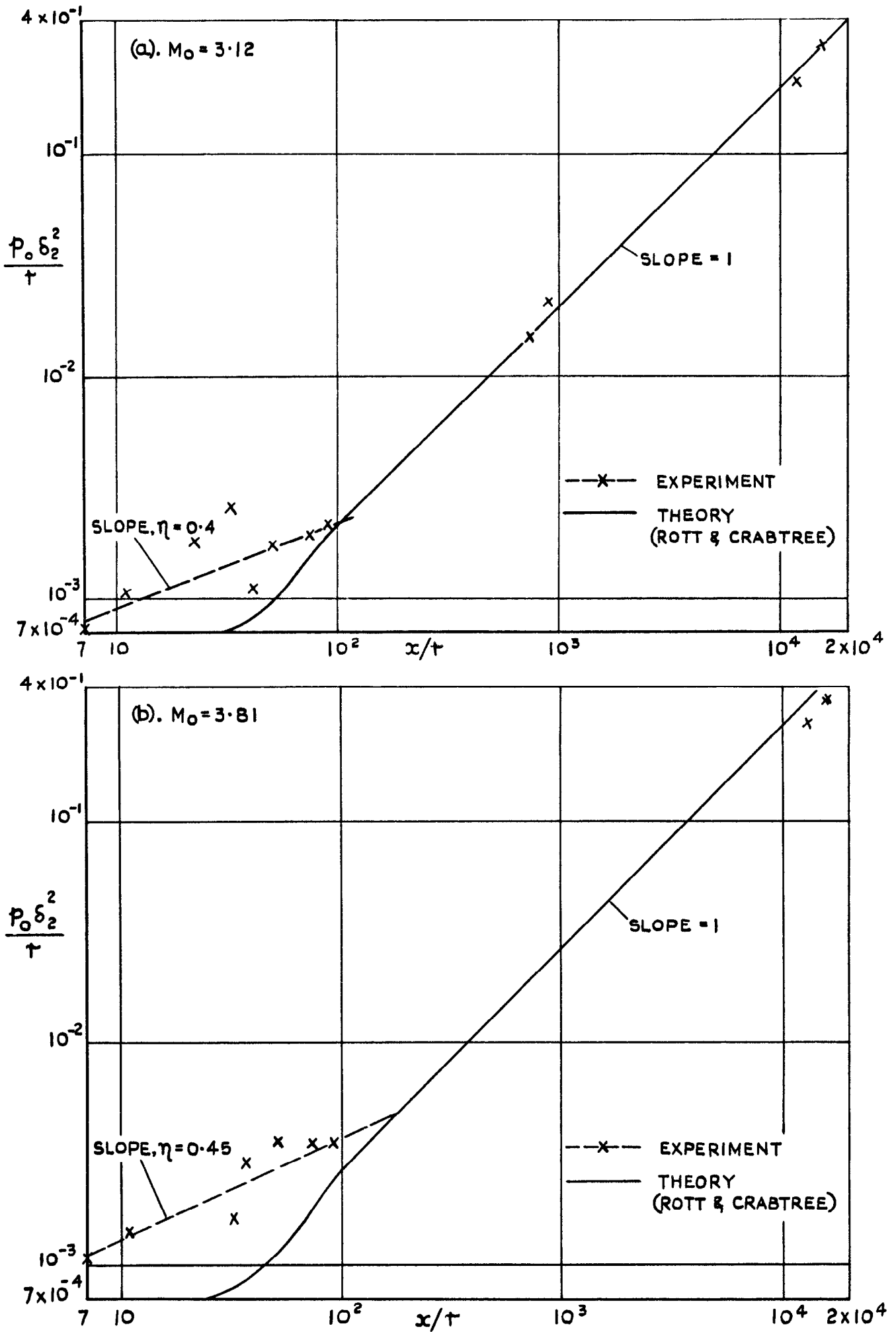
FIG.15. VARIATION OF p_0 \delta_2^2 / \tau WITH x/\tau .
