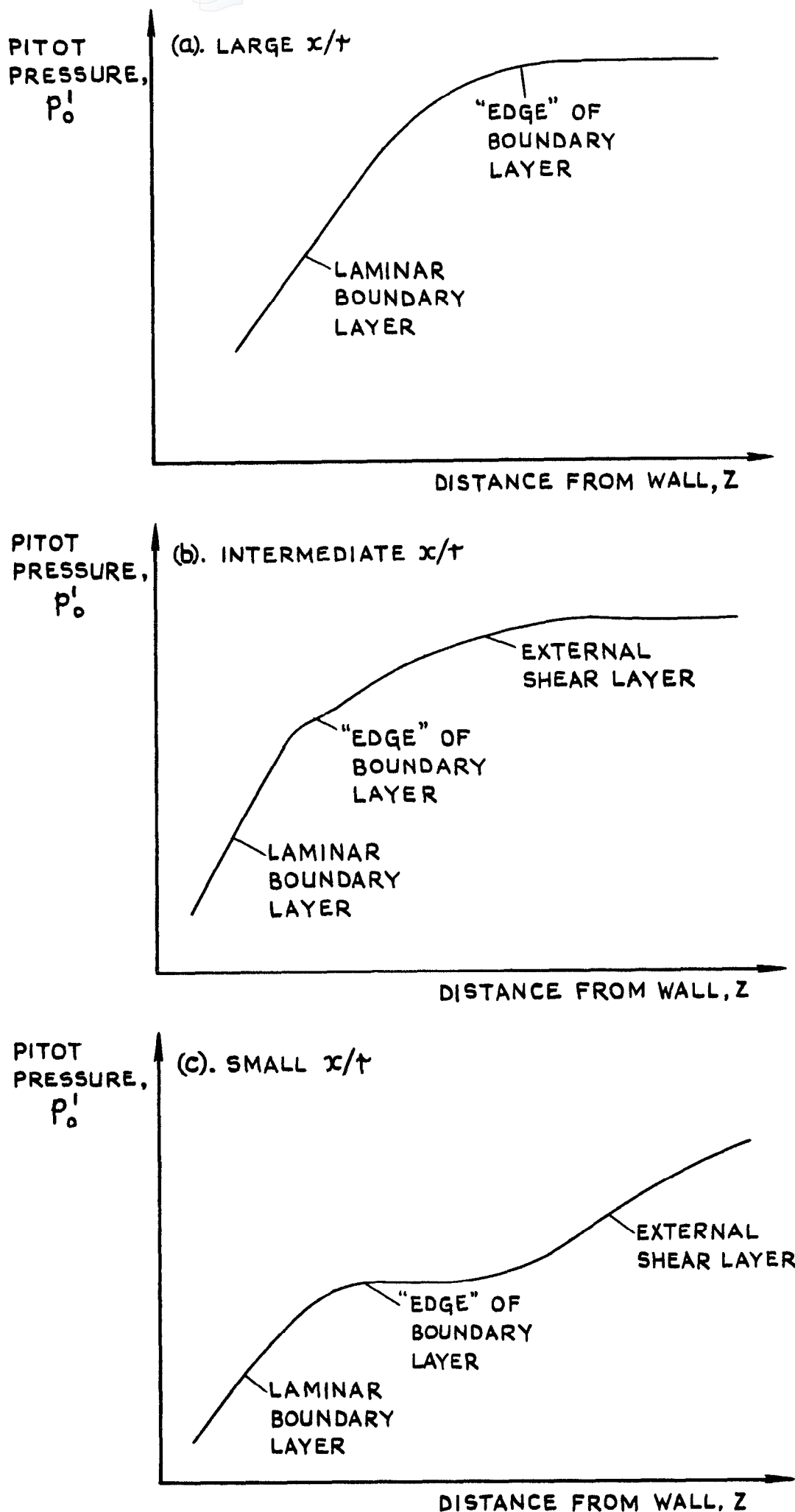
FIG.10. TYPICAL BOUNDARY-LAYER TRAVERSES AT DIFFERENT POSITIONS ON A BLUNT CONE. (NOT TO SCALE).
