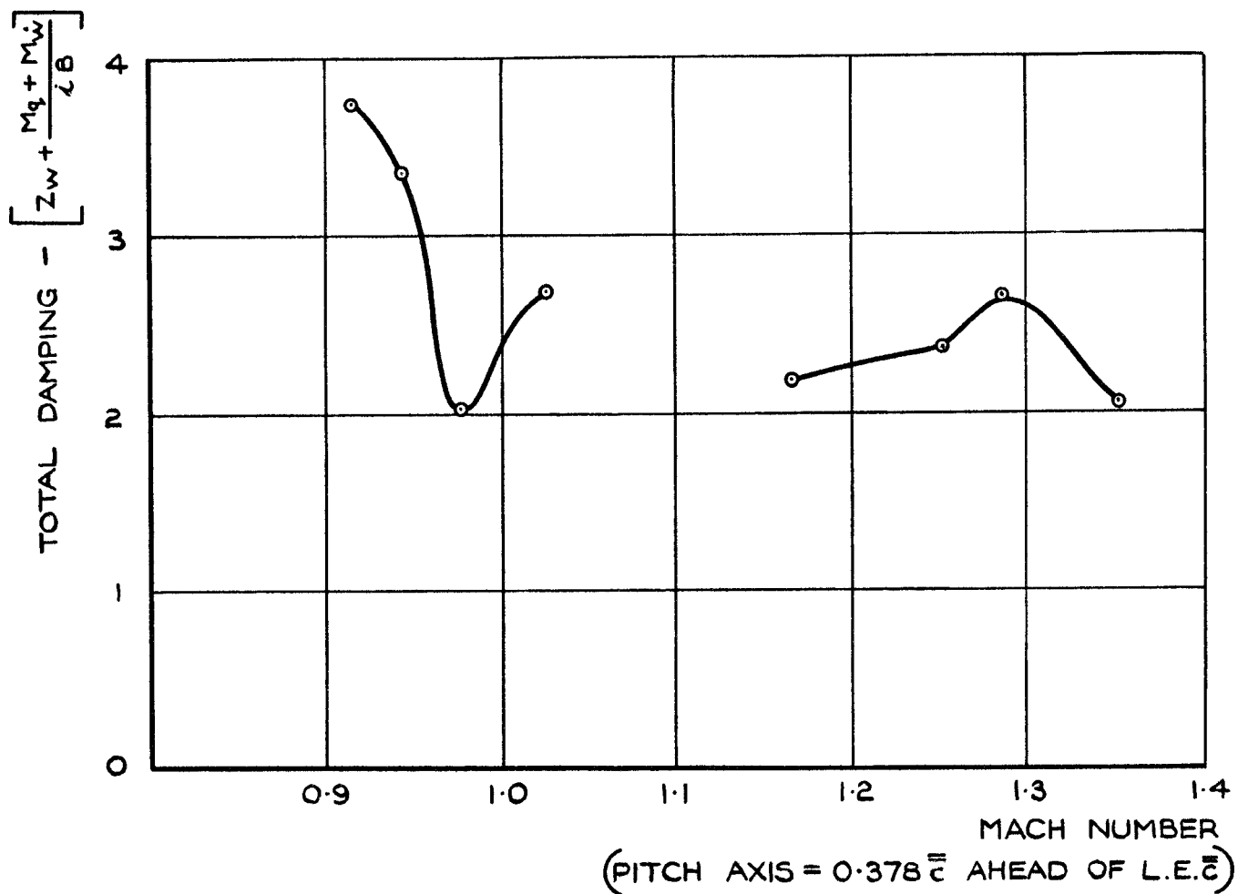
FIG. 12. TOTAL PITCH-DAMPING.
