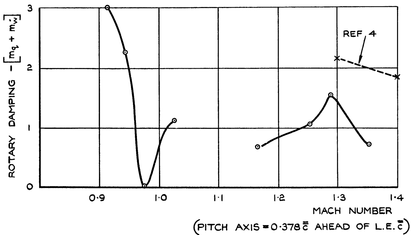
FIG. 13. ROTARY PITCH-DAMPING.
