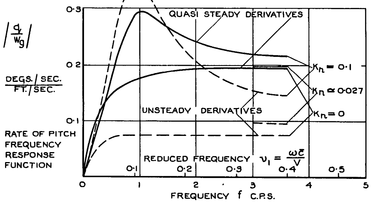
FIG. 16. COMPARISON OF MEASURED AND THEORETICAL RATE OF PITCH / GUST INPUT FREQUENCY RESPONSE FUNCTIONS FOR RIGID AIRCRAFT.
