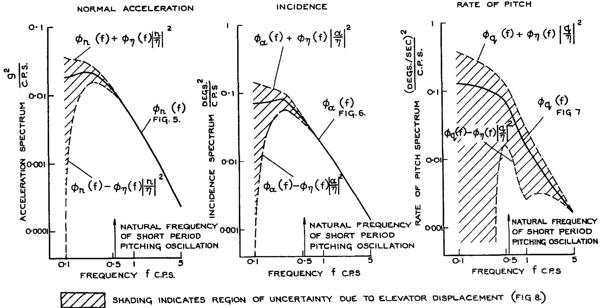
FIG.13. MAXIMUM POSSIBLE EFFECTS OF ELEVATOR DISPLACEMENT ON SPECTRA OF ACCELERATION, INCIDENCE AND RATE OF PITCH.
