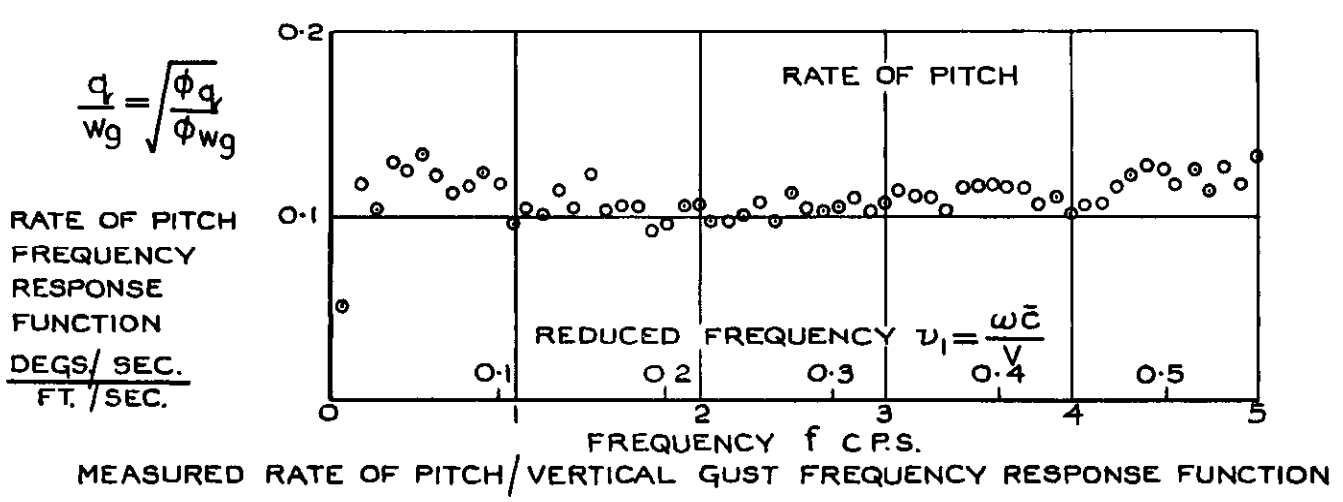
FIG. 9. MEASURED FREQUENCY RESPONSE FUNCTIONS SHOWING RESPONSE OF PILOT-AIRCRAFT COMBINATION TO UNIT VERTICAL GUST.
