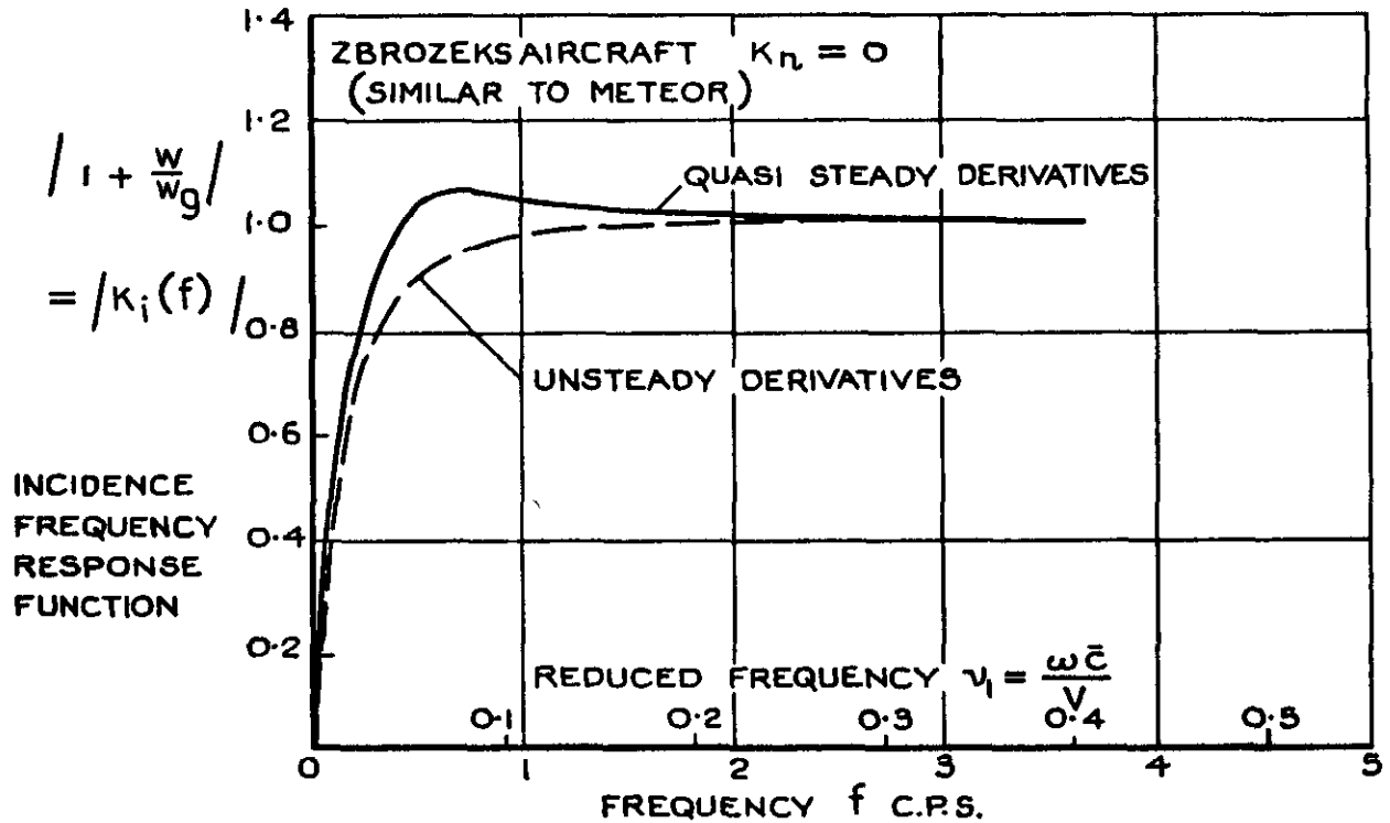
FIG. 15. COMPARISON OF NON DIMENSIONAL MEASURED AND THEORETICAL INCIDENCE/GUST INPUT FREQUENCY RESPONSE FUNCTIONS FOR RIGID AIRCRAFT.
