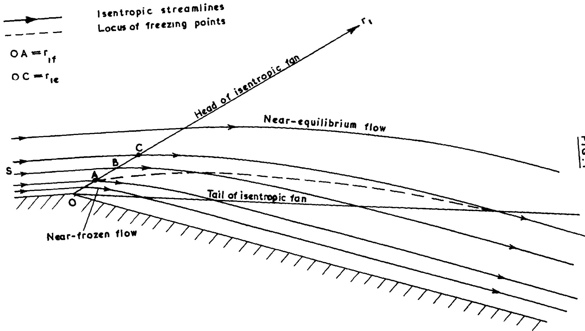
Isentropic streamlines and locus of freezing points (schematic)
