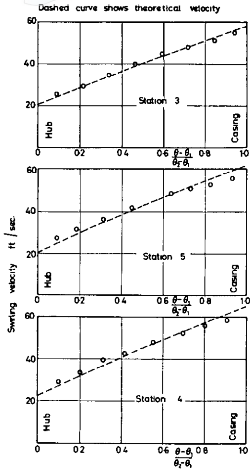
FIG 27(a) SWIRLING VELOCITY COMPONENT AT STATIONS 3,4 & 5
