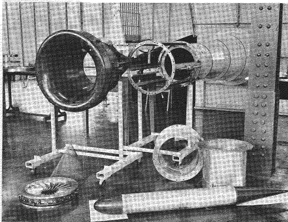
FIG. 9 (b) COMPONENTS OF ANNULAR CASCADE WIND TUNNEL.
