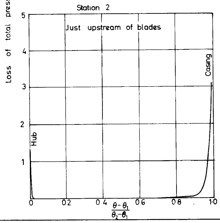
BOUNDARY LAYER TRAVERSES AT STATIONS 1&2 OF CONICAL ANNULAR DUCT.
