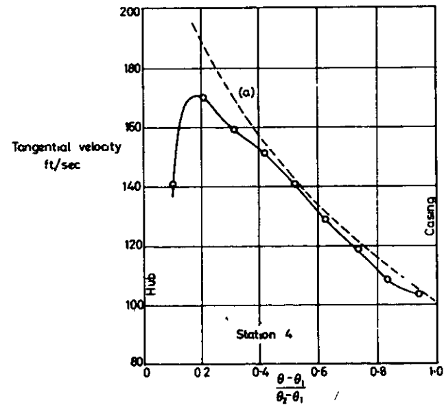
VELOCITY COMPONENTS DOWNSTREAM OF FREE VORTEX ANNULAR CASCADE IN CONICAL ANNULUS WITH NON-UNIFORM INLET STAGNATION PRESSURE
