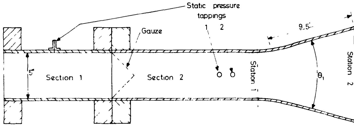
PLAN VIEW OF DUCT
