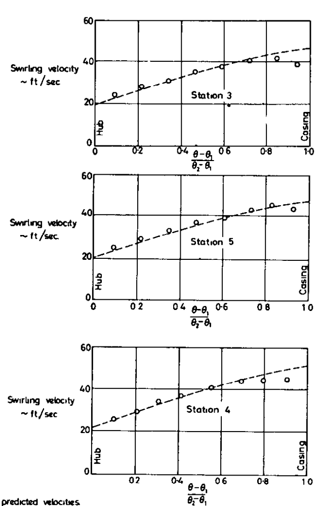
FIG 29 (b) SWIRLING VELOCITY COMPONENT AT STATIONS 3 4 & 5
