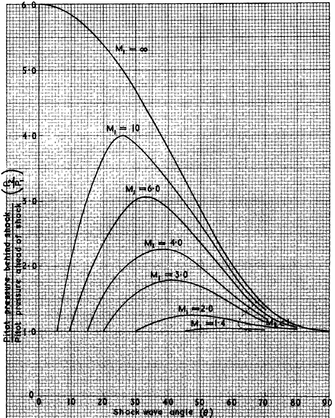
The change of pitot pressure across oblique shock waves
