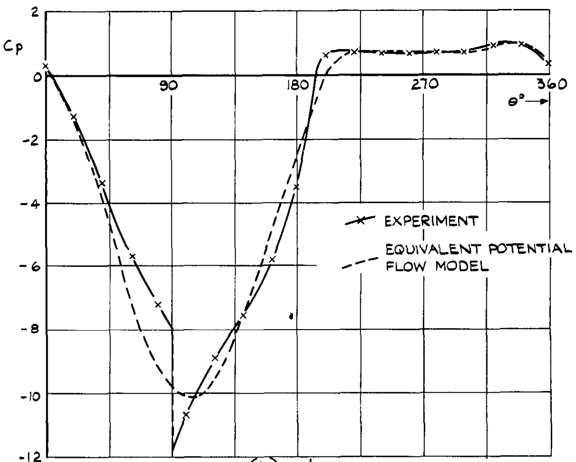
(b) C_{z'} = 7.62
