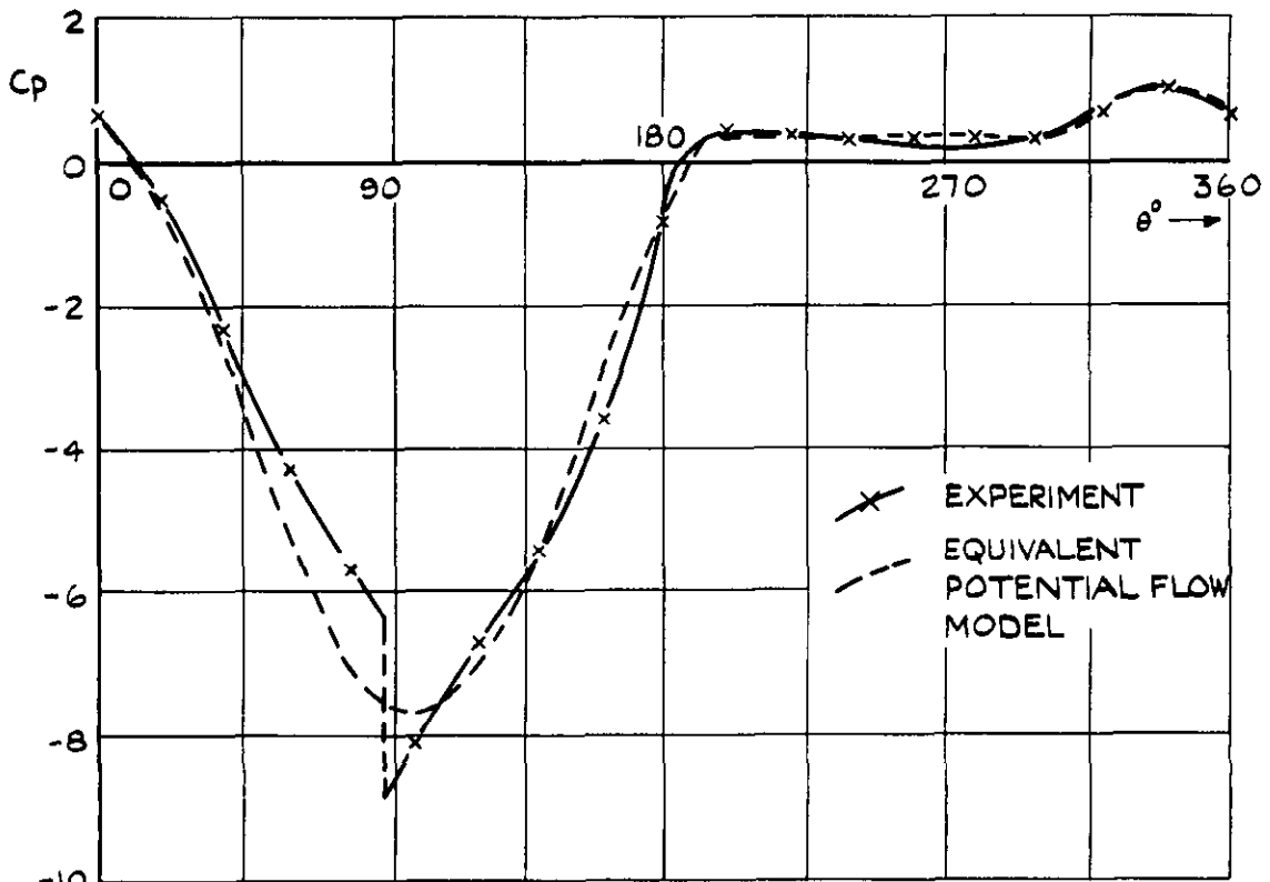
(a) C_{z'} = 5.53
