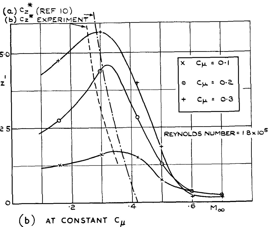
(b) AT CONSTANT c_\mu FIG.17 EFFECT OF MACH No ON NORMAL FORCE CHARACTERISTICS
