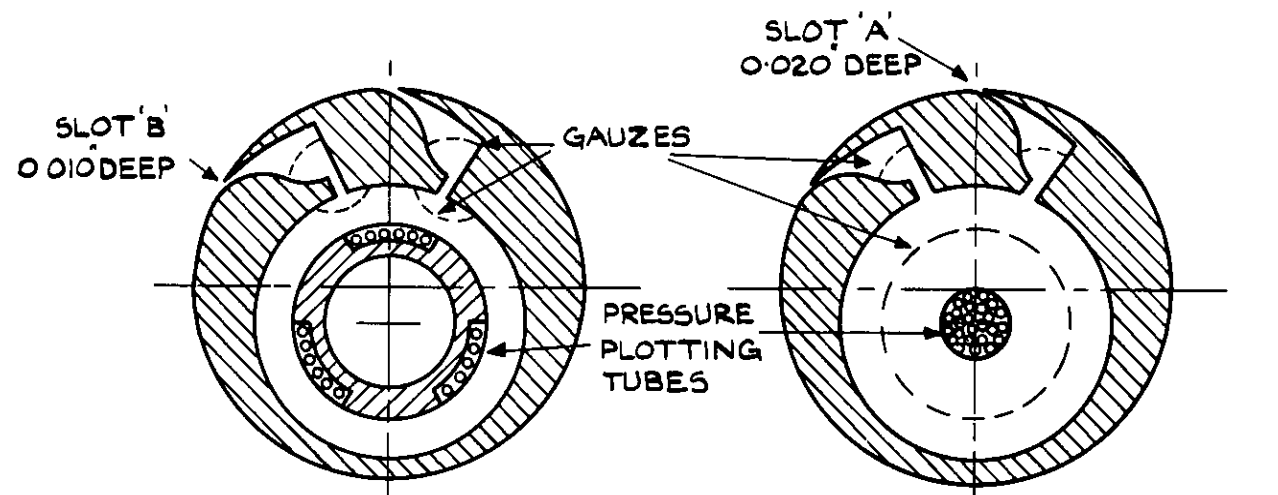
TYPICAL CROSS-SECTION OF "EARTH" SECTION
