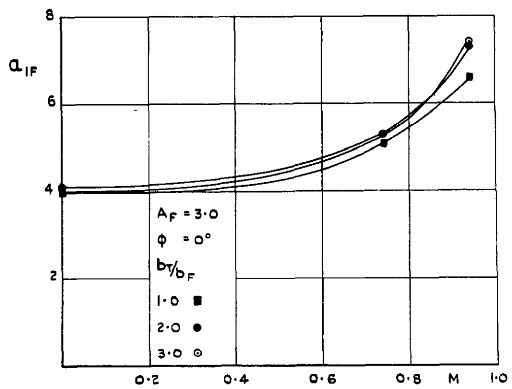
(b). VARIATION OF FIN LIFT CURVE SLOPE WITH MACH NUMBER.
