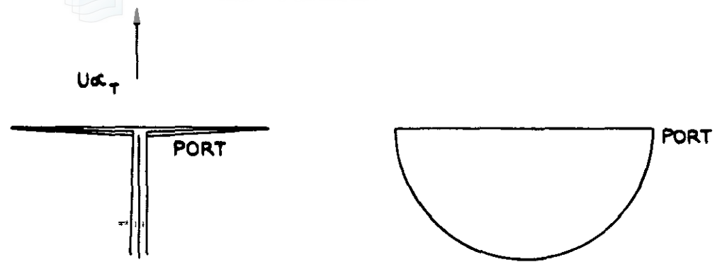
(a) NEGATIVE INCIDENCE LOADING
