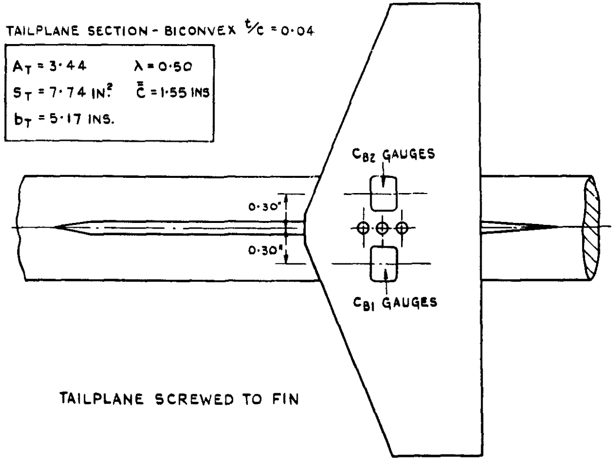
FIG.7. GEOMETRY OF FIN AND TAILPLANE OF MODEL A.
