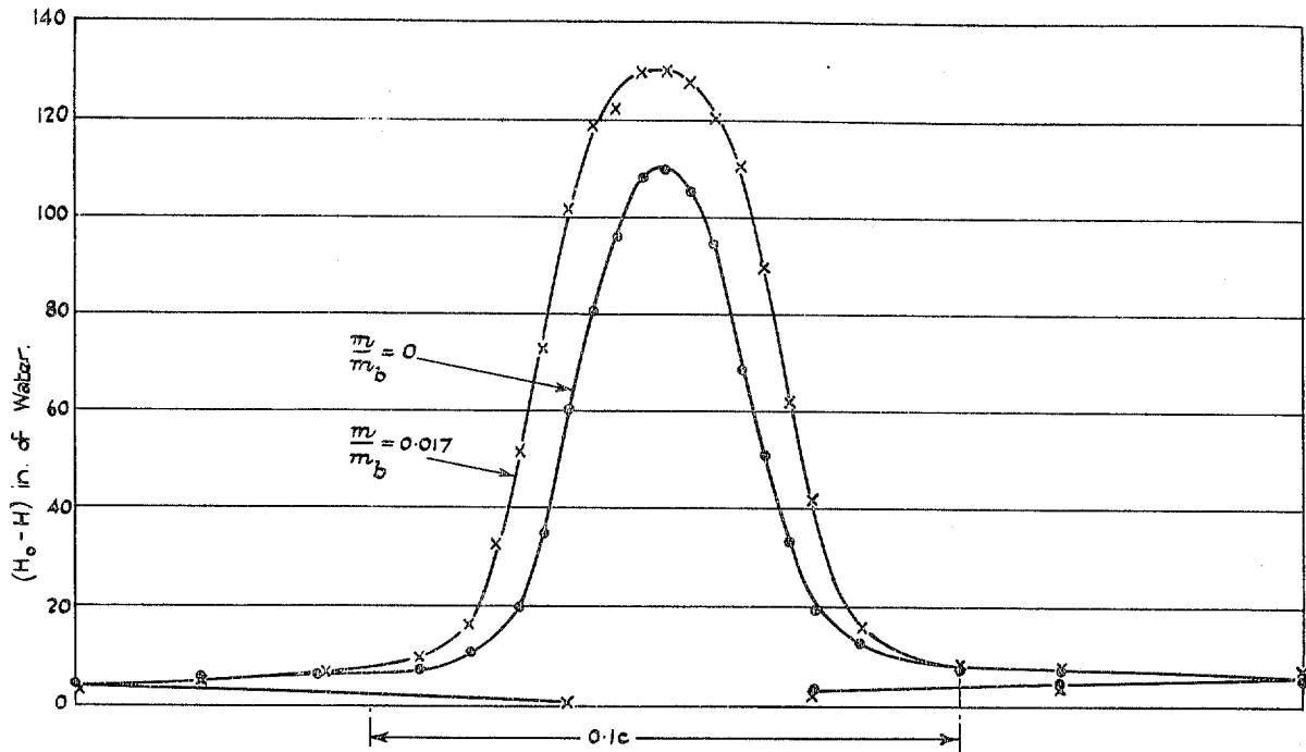
FIG. 6. Aerofoil EC 1250. 0 deg. Incidence. M = 0.762 . Total-head Loss in Wake at 0.017c behind Trailing Edge.
