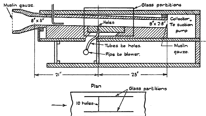
FIG. 1. Elevation View of Smoke Tunnel.
