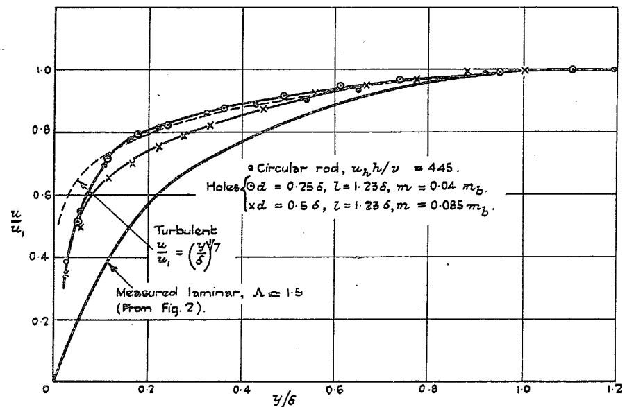
FIG. 3. Velocity Distribution at Section 22 \delta behind Standard Section.
