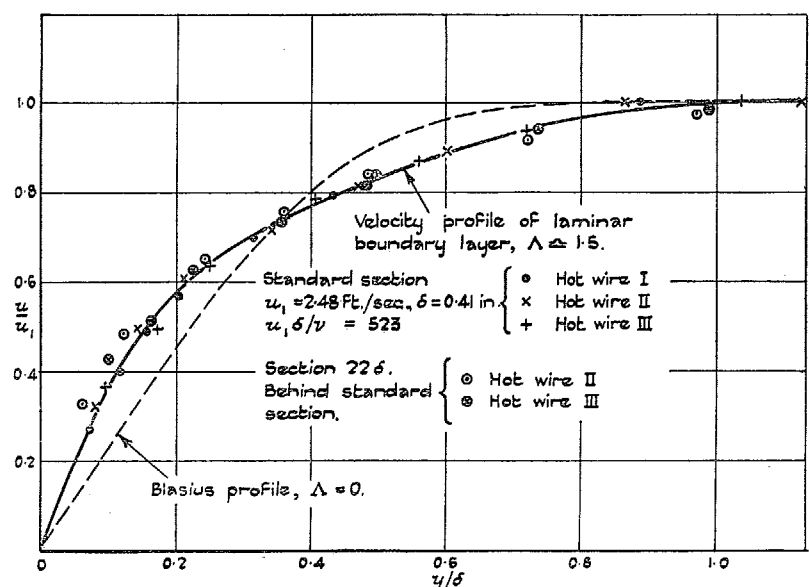
FIG. 2. Velocity Distribution in Boundary Layer on Floor.
