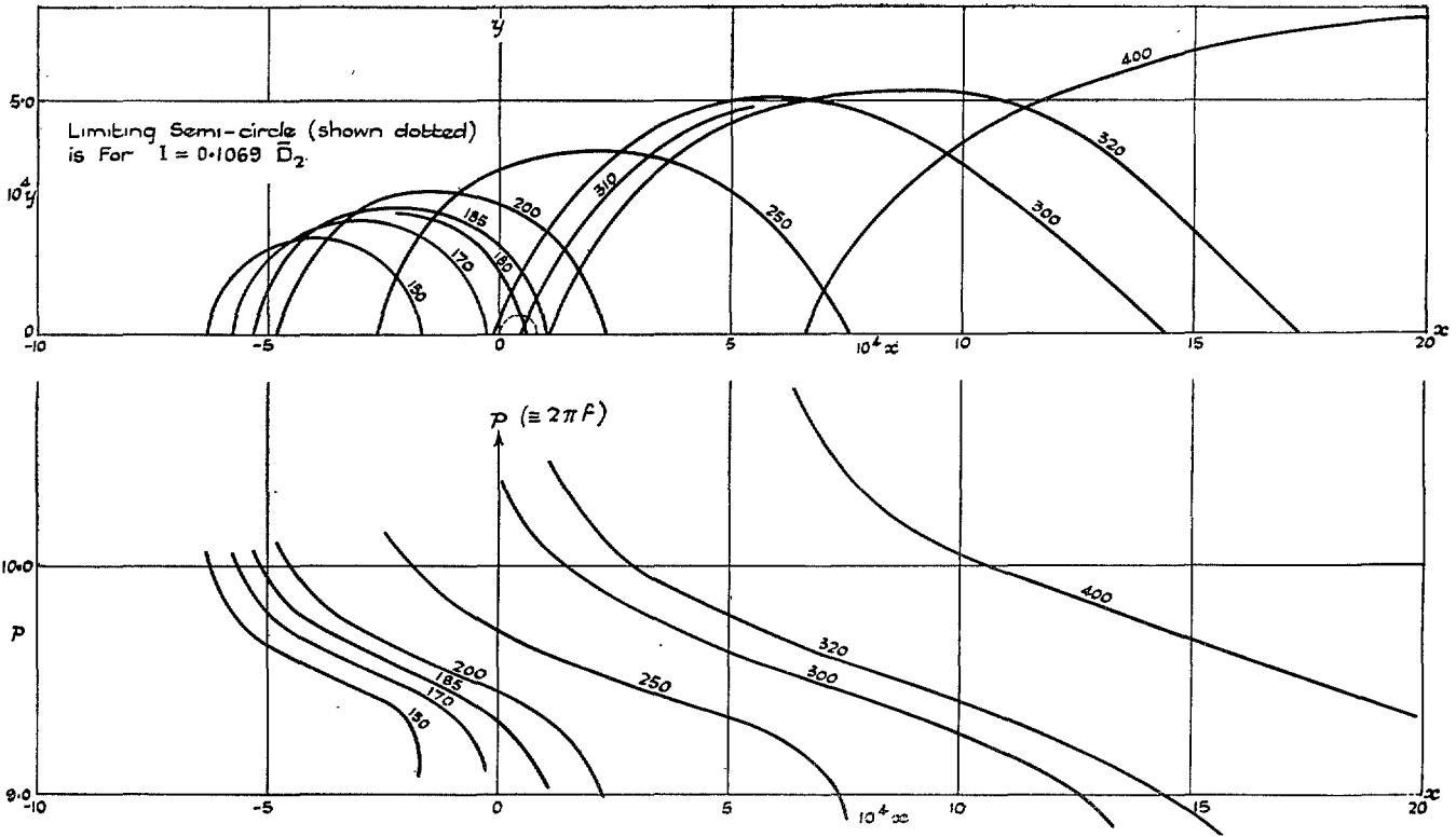
FIG. 7. (x, y) diagram for balanced aileron-carried damper. Tank empty; h = 30,000 , h_E = 0 .
