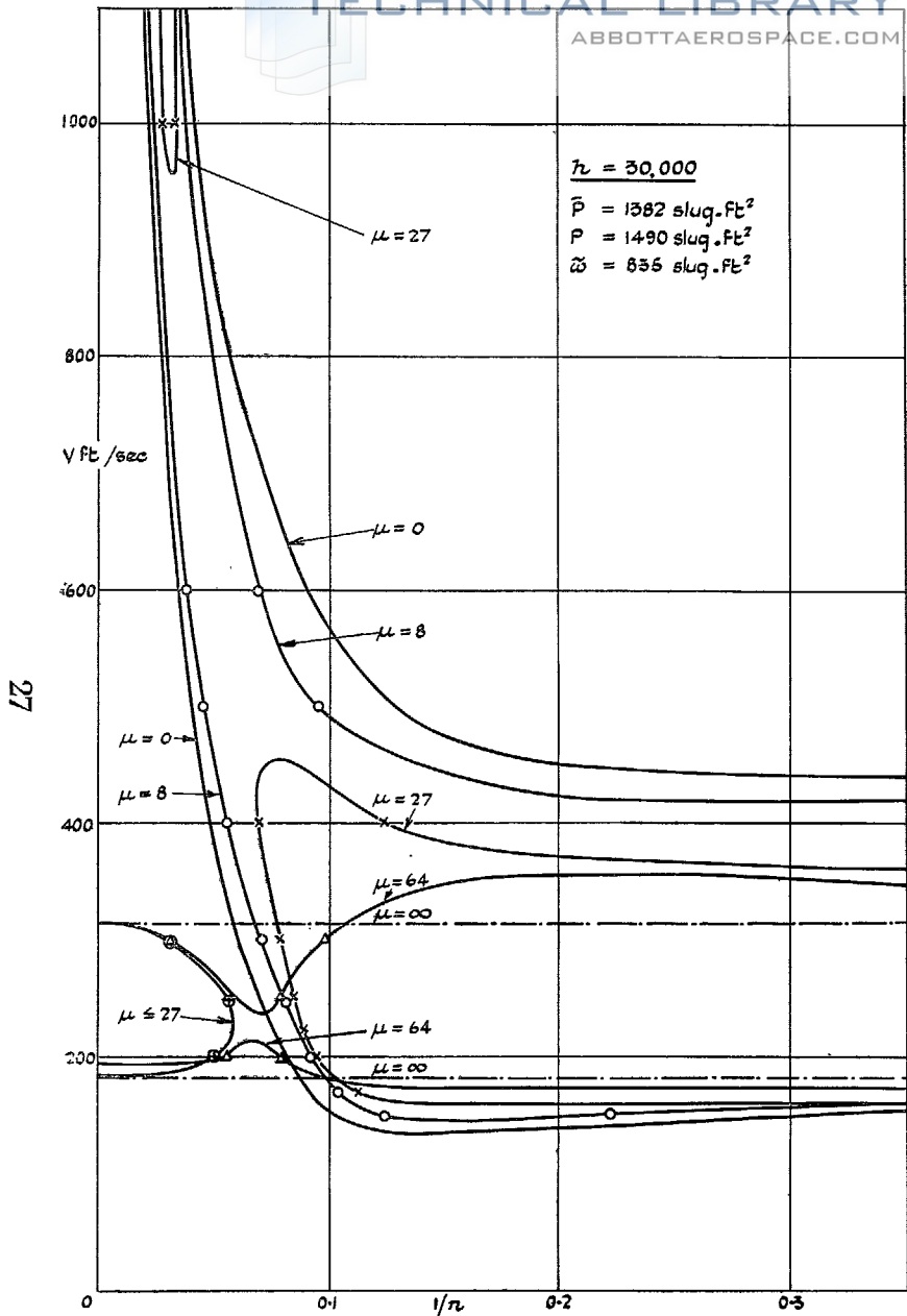
FIG. 24. Final damping diagram for a partly mass-balanced aileron-damper system (altitude effect).
