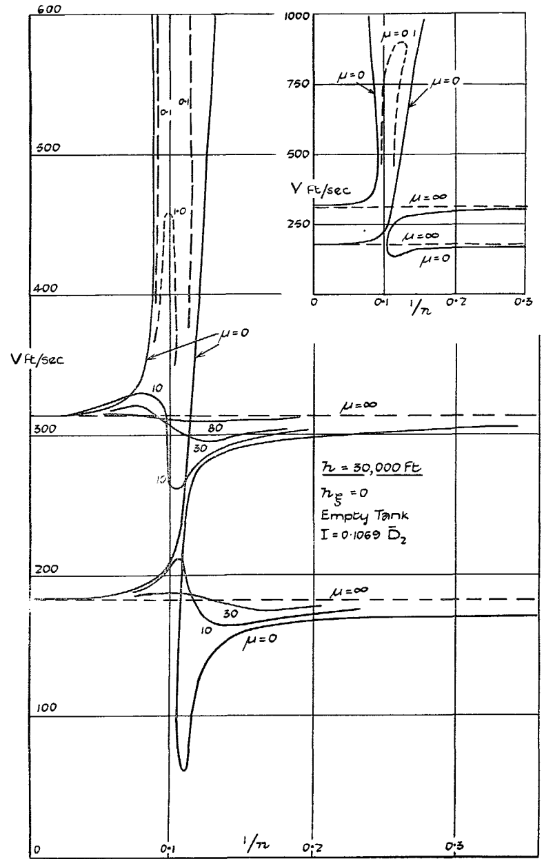
FIG. 9. Final damping diagram for balanced aileron-carried damper.
