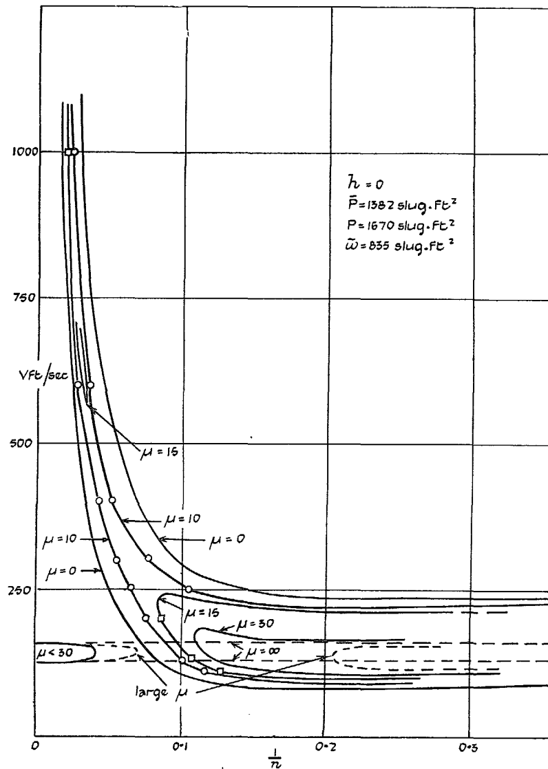
FIG. 23. Final damping diagram for a partly mass-balanced aileron-damper system.
