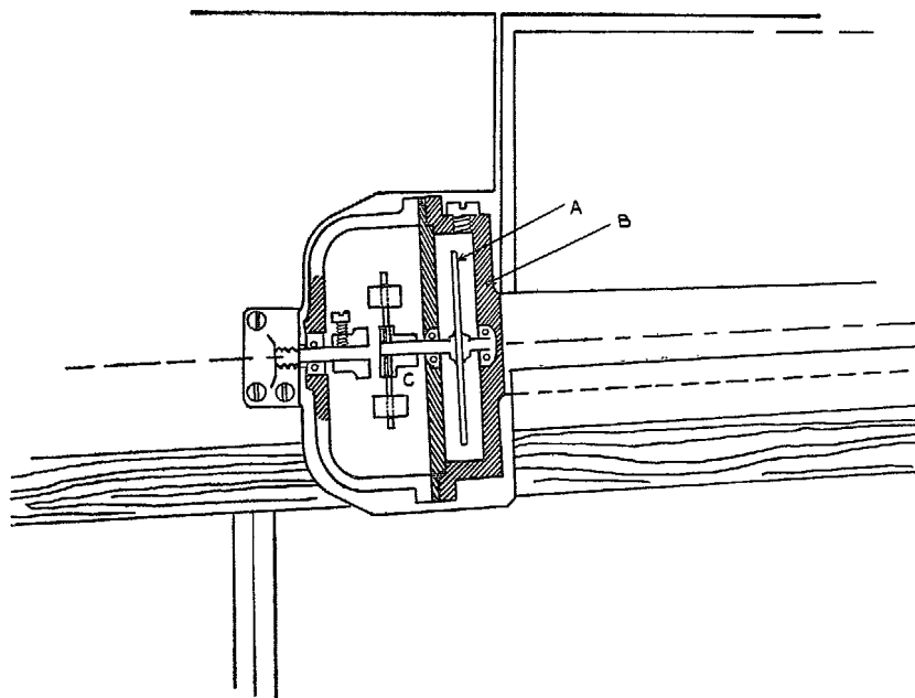
FIG. 29. Arrangement of damper.
