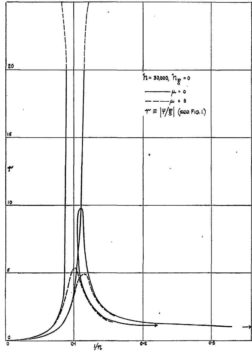
FIG. 17. Amplitude ratio diagram for case of Fig. 9.
