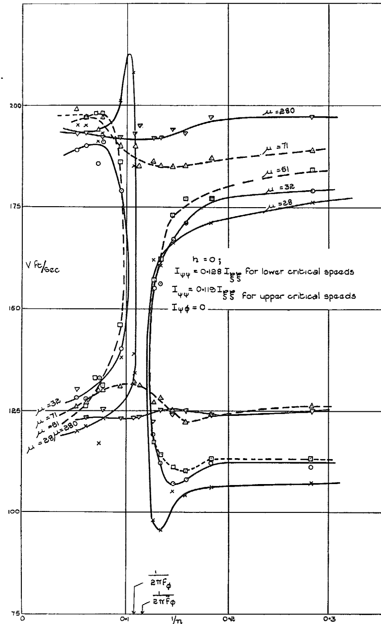
FIG. 30. Influence of balanced aileron-carried damper on antisymmetrical wing flexure-aileron flutter.
