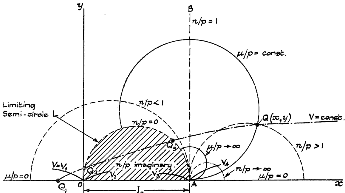
FIG. 2. Detail of (x, y) diagram for balanced aileron-carried damper.
