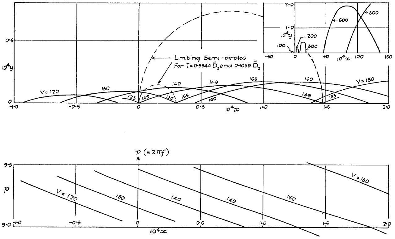
FIG. 3. (x, y) diagram for balanced aileron-carried damper. Tank empty; h = 0 , h_{\xi} = 0 .
