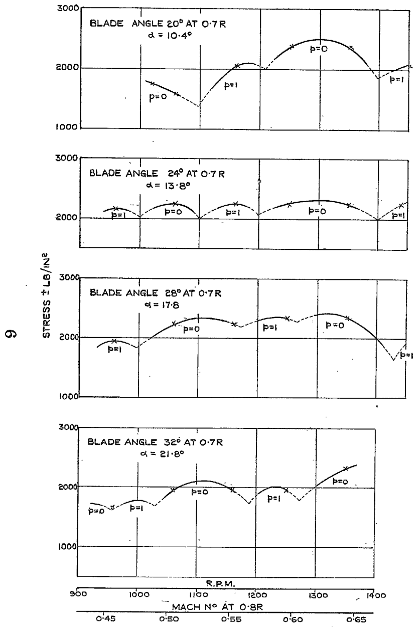
FIG. 3. Two-blade propeller. Torsional stress at 0.75R and blade phasing.
