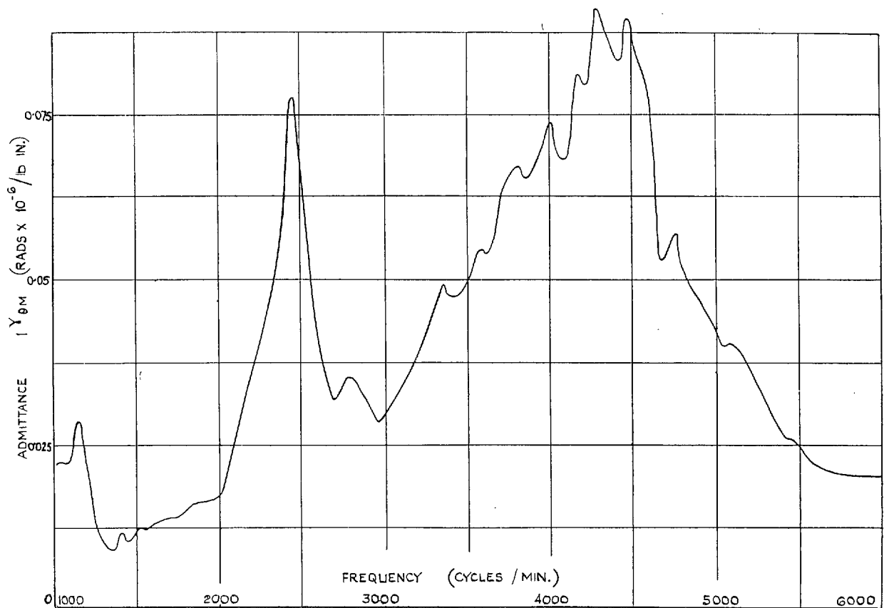
FIG. 6. Admittance measured on airframe. Angular deflection per unit moment.
