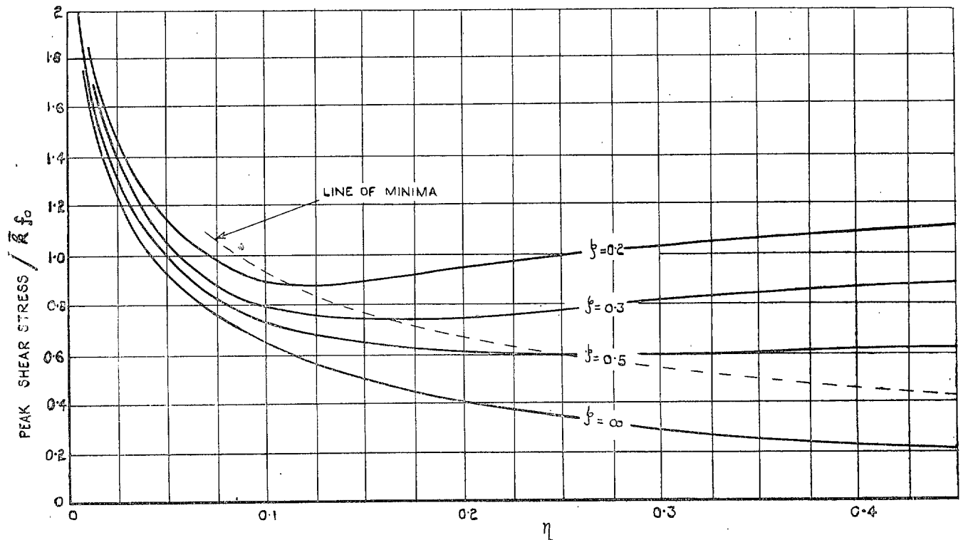
FIG. 33. Peak values of shear adjacent to the boom (variation with \eta ).
