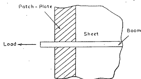
DIAG. 12. Shear-stiffener.
