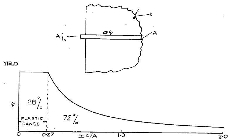
FIG. 7. Modified theoretical curve showing that about 28 per cent of the boom load might be taken by skin in the plastic range which extends about 0.27A/l along the boom.
