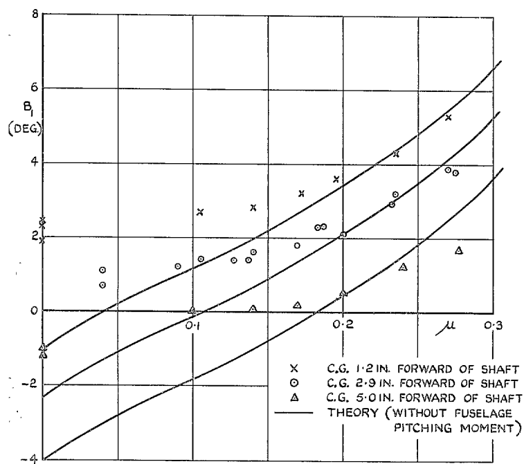
FIG. 12. Longitudinal control to trim. S-51. Level flight. 172 r.p.m.
