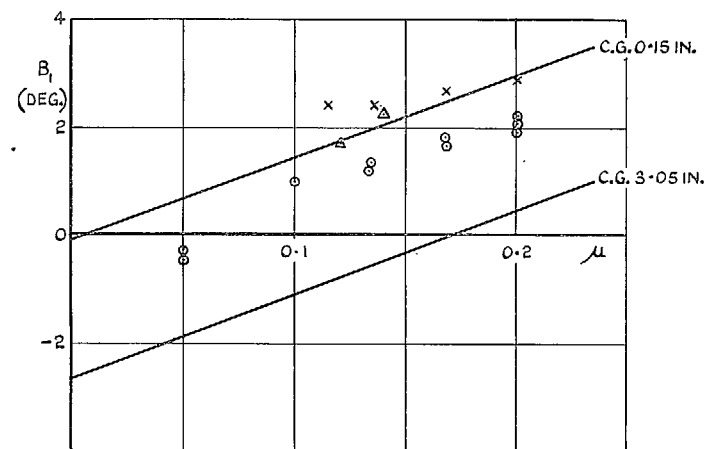
FIG. 10. Longitudinal control to trim. R-4B. Autorotation.
