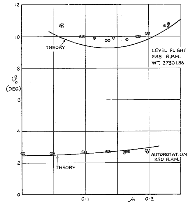
FIG. 7. Collective pitch angles. R-4B helicopter.
