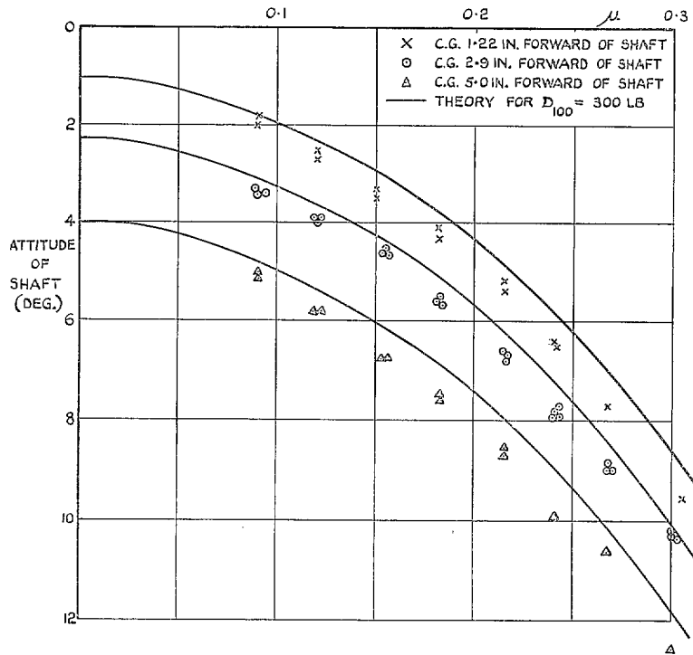
FIG. 27. Attitude of S-51 in level flight.
