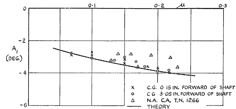
FIG. 19. Lateral control to trim. R-4B. Level flight.
