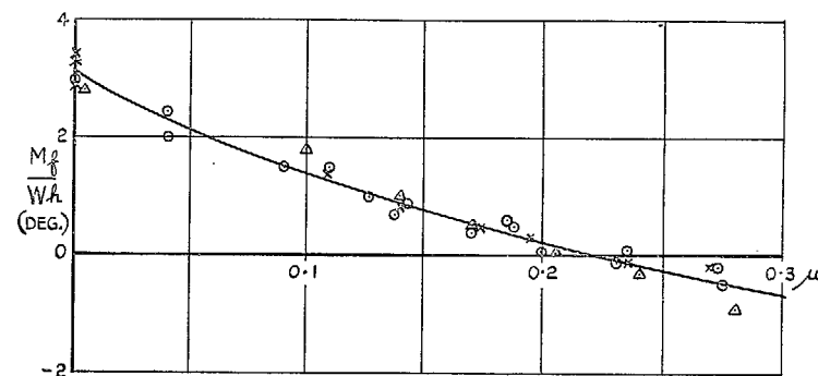
FIG. 17. Fuselage pitching moment. S-51. Level flight. 172 r.p.m.
