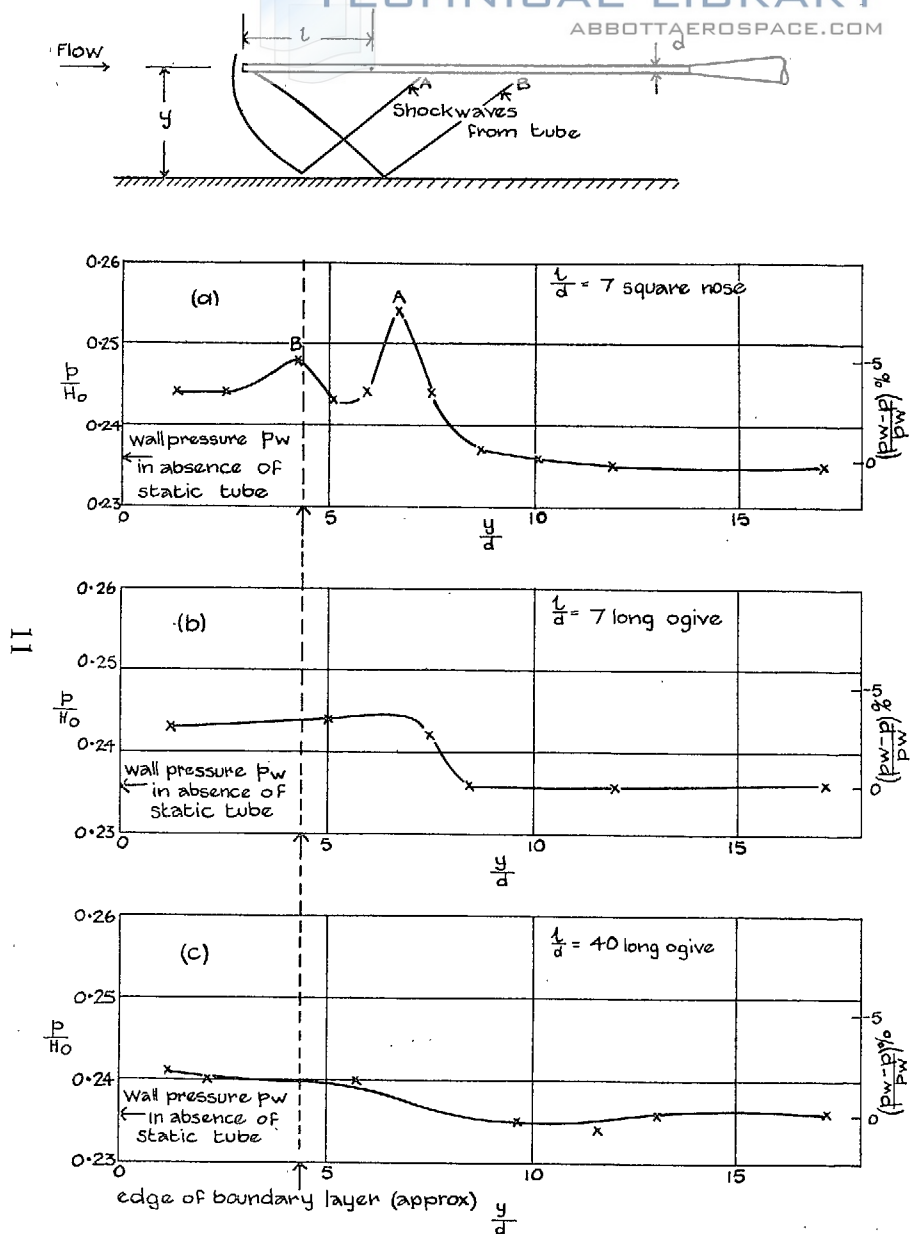
FIG. 5. Static-tube reading near a wall.
