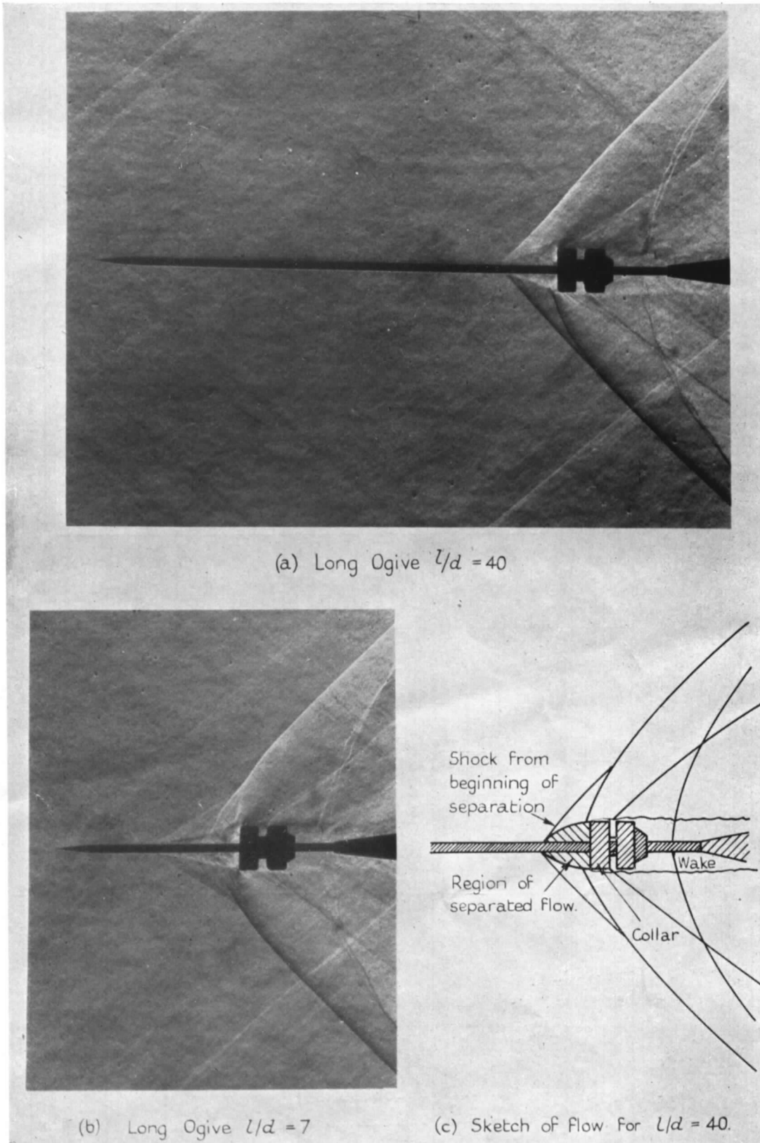
FIG. 4. Interaction of a shock wave with the boundary layer on a static-tube.
