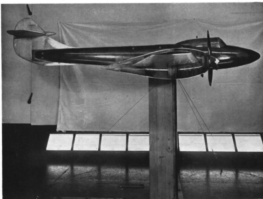
FIG. 15. Case H. Side view of model, fitted with propellers, faired nacelles and with upper and lower dorsal fins.
