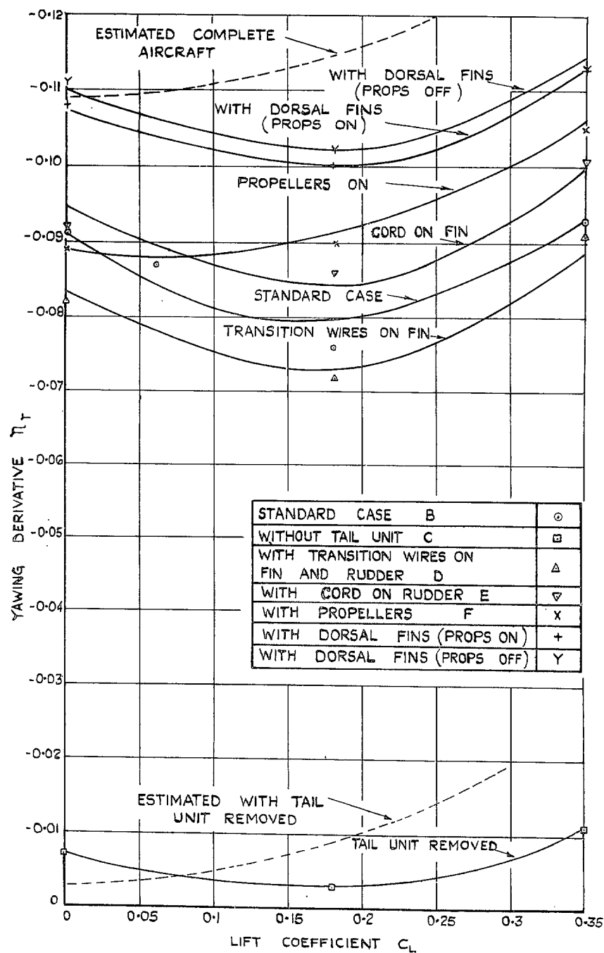
FIG. 16. Variation of lateral stability derivative n_r with lift coefficient for various conditions of model.
