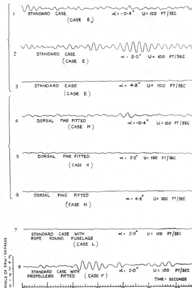
FIG. 9. Typical 'free run' records for various conditions of model.
