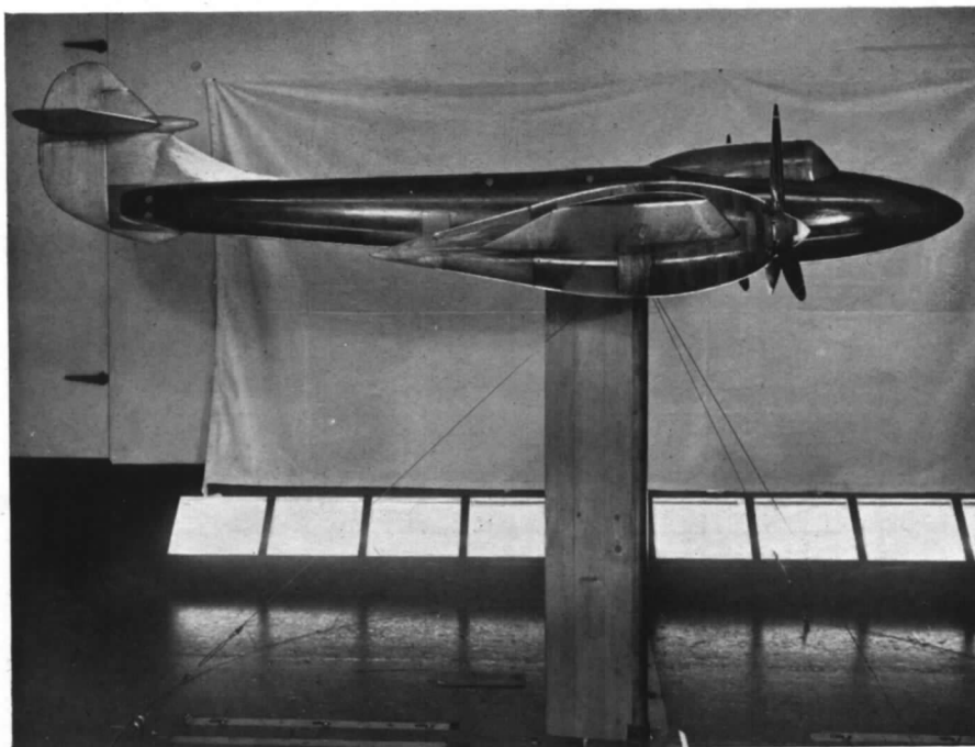
FIG. 14. Case G. Side view of model, fitted with propellers, faired nacelles and upper dorsal fin.
