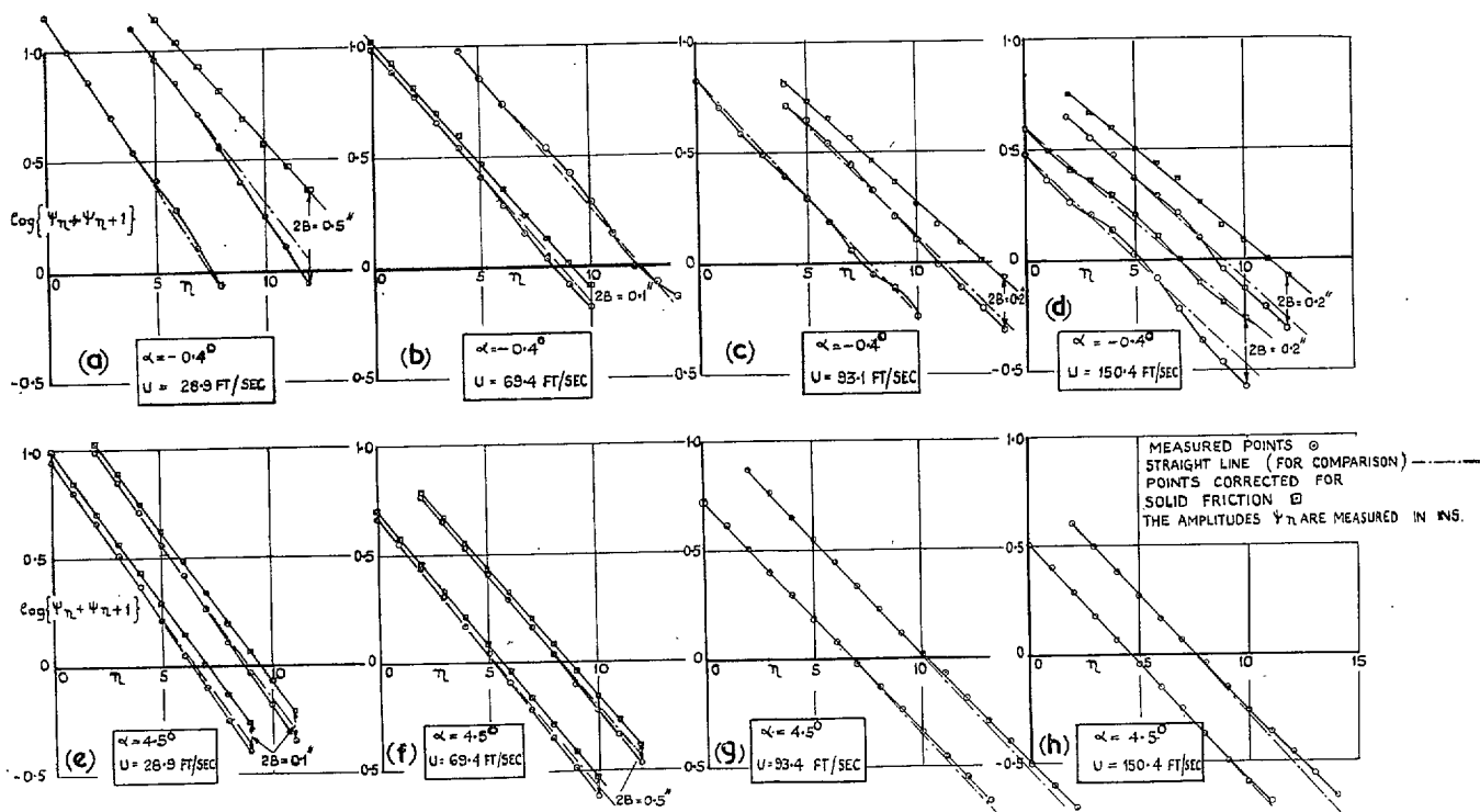
FIG. 17. Effect of solid friction on results.
