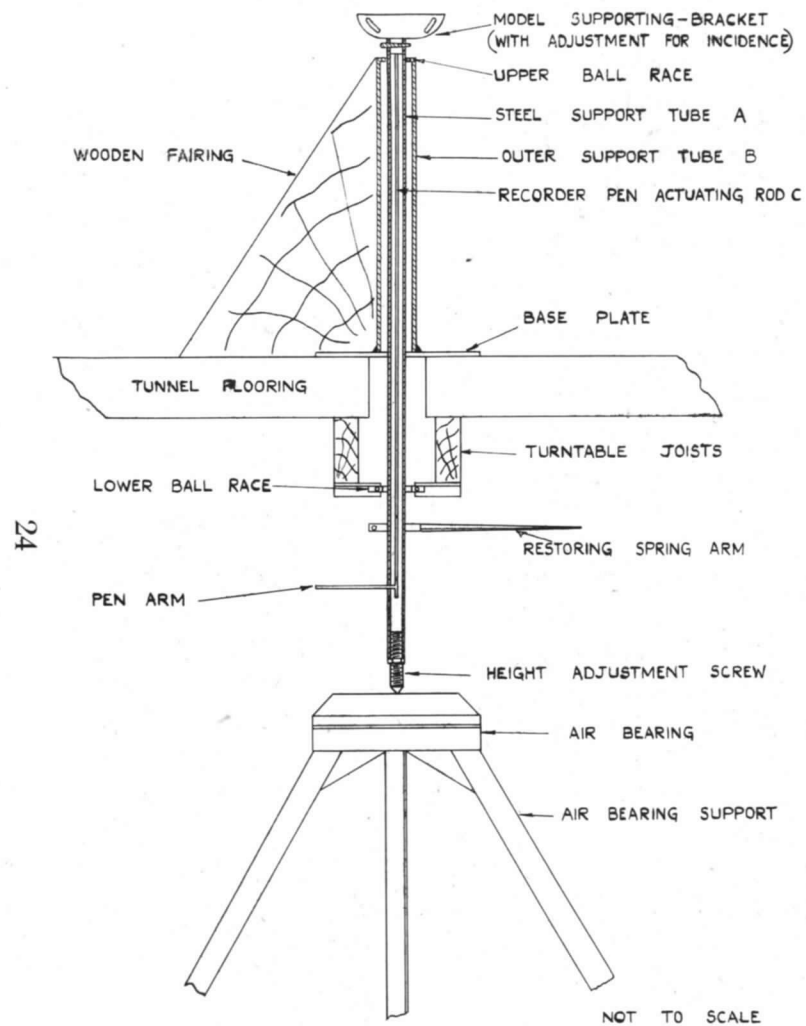
FIG. 3. Details of supporting rig for model.
