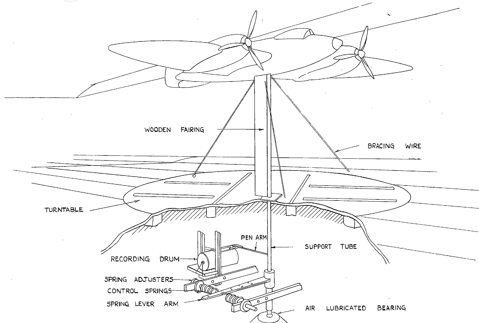
FIG. 2. Sketch showing general arrangement of model rig in wind-tunnel.
