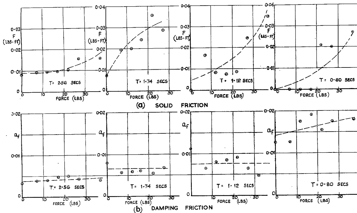
FIG. 18a and b. Effect of Drag force on friction.
