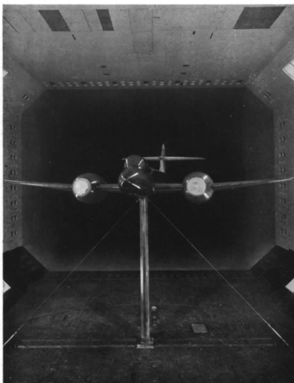
FIG. 11. Case B. Front view of standard model with nacelles blocked and faired.
