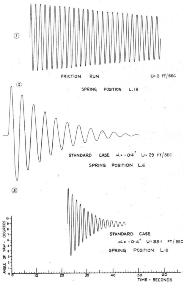
FIG. 8. Typical records of n_r runs.
