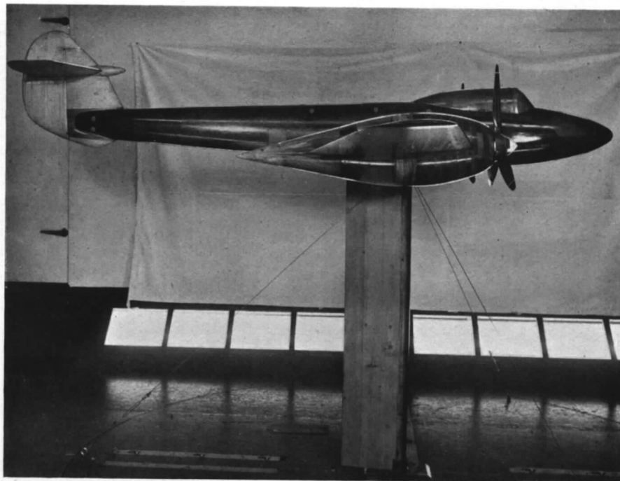
FIG. 12. Case F. Side view of model fitted with propellers and faired nacelles.
