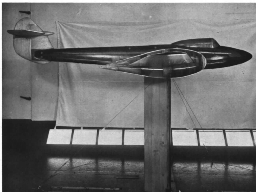
FIG. 10. Case B. Side view of standard model with nacelles blocked and faired.
