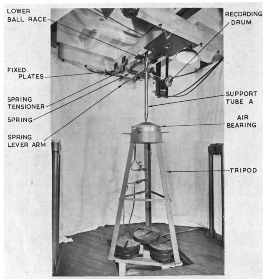
FIG. 4. Lower part of supporting rig beneath tunnel working-section.
