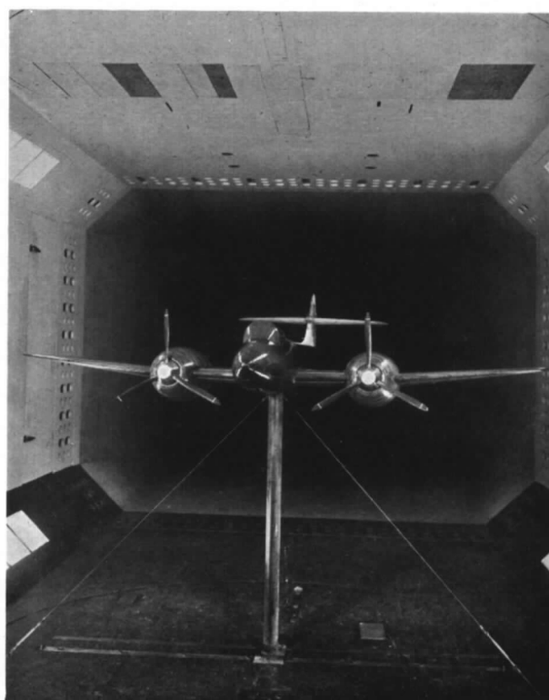
FIG. 13. Case F. Front view of model, fitted with propellers and faired nacelles.
