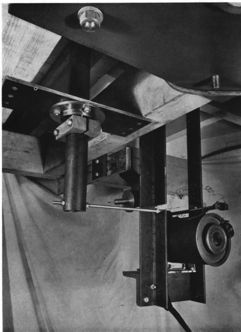
FIG. 5. Arrangement of recording gear. (Air-bearing removed.)
