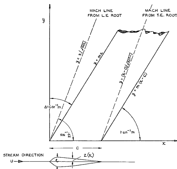
FIG. 2. Symbols for swept wings.
