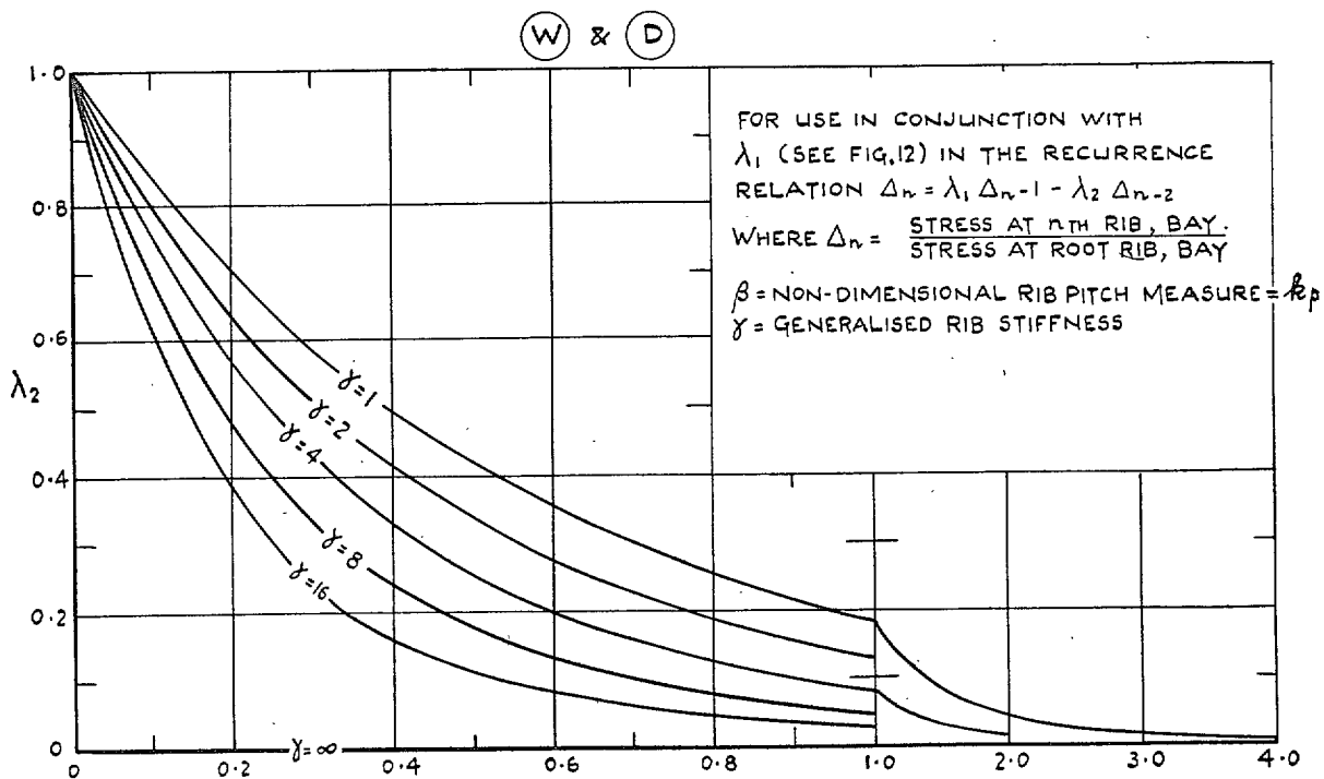
FIG. 13. \lambda_2 - \beta - \gamma family of curves.
