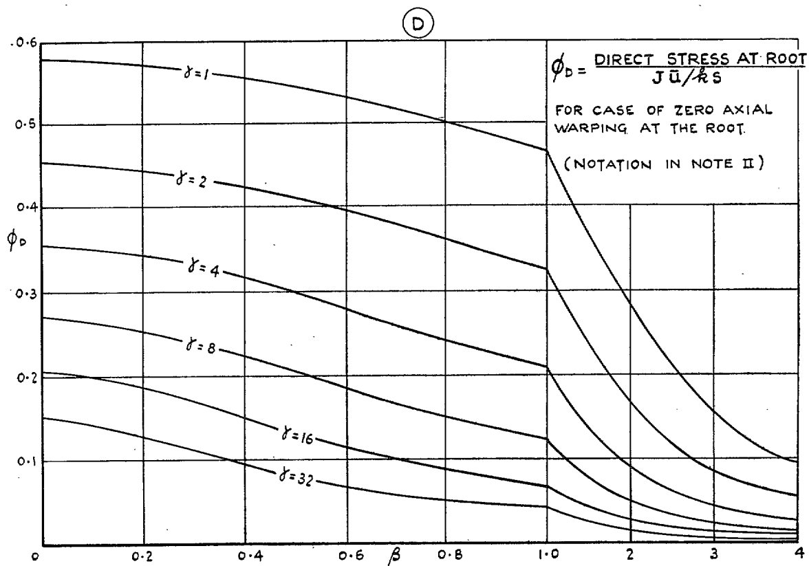
FIG. 14. Direct stress at root due to shear-distortion at root.
