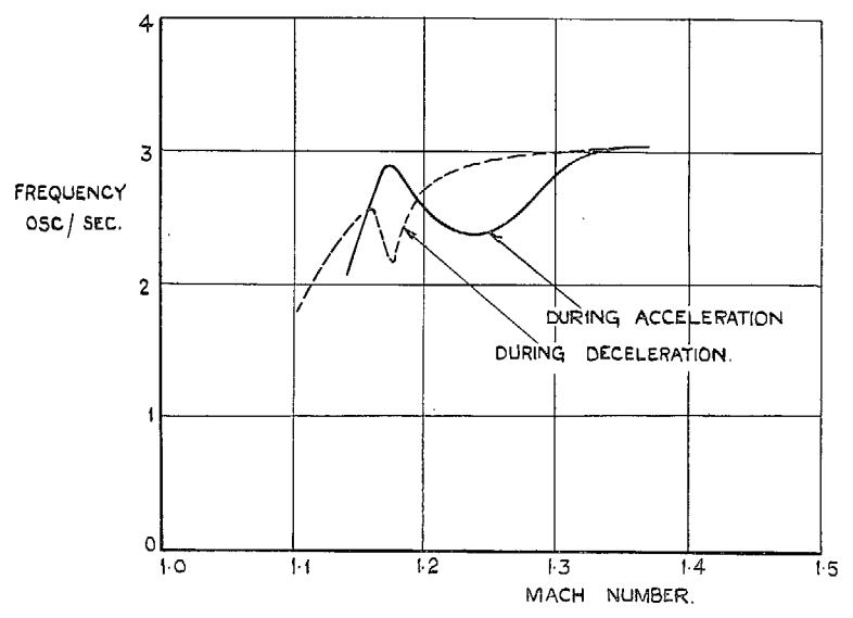
FIG. 20. Variation of frequency of oscillations in tailplane angle and normal acceleration with Mach number.
