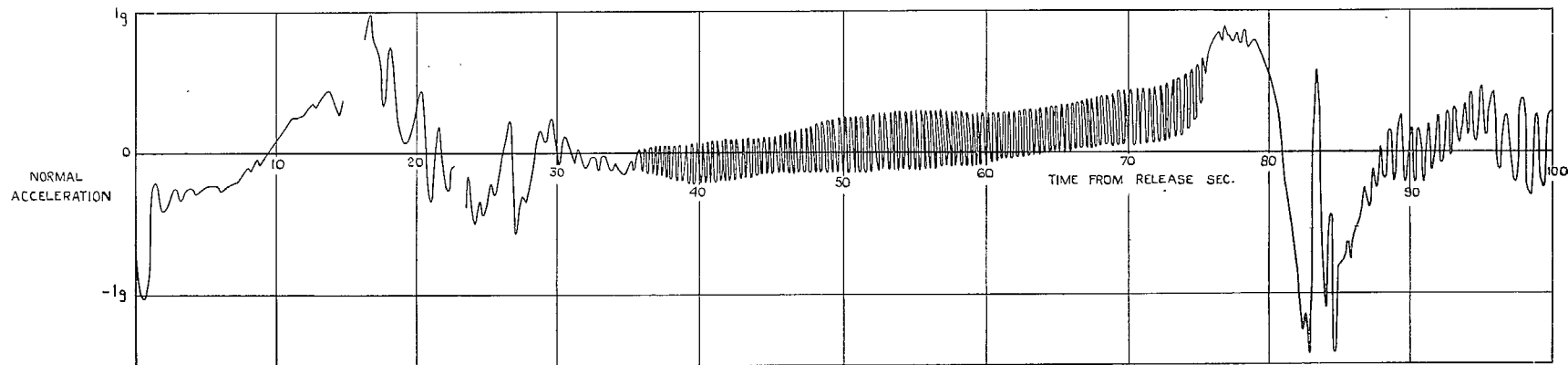
FIG. 18. Variation of normal acceleration during flight.
