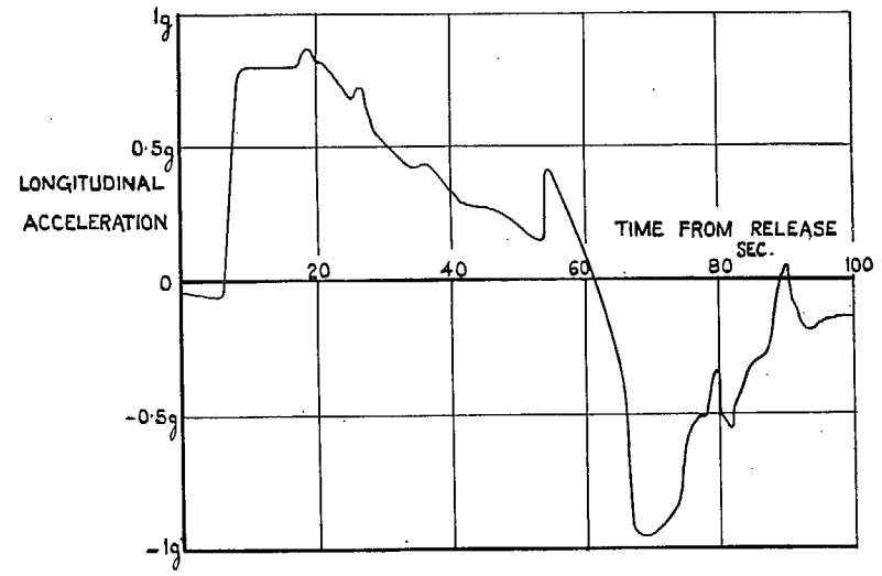
FIG. 8. Variation of longitudinal acceleration during flight.
