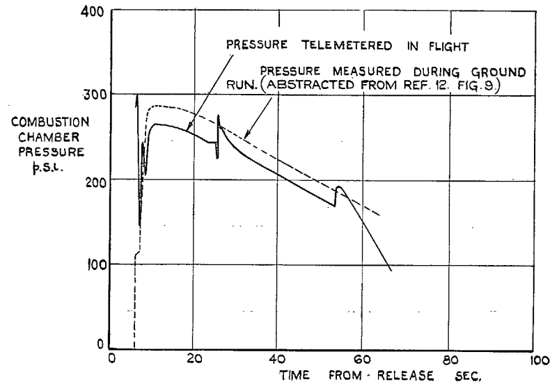
FIG. 13. Variation of combustion-chamber pressure during flight.
