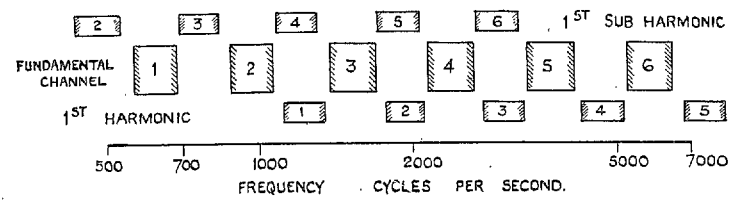
FIG. 31. Telemetering system audio-frequency spectrum.
