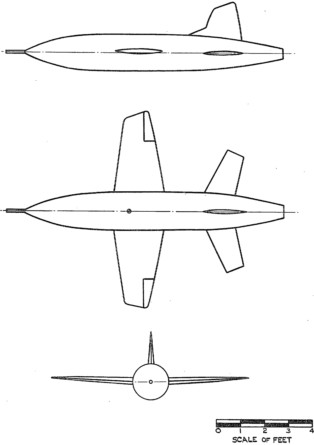
FIG. 1. General arrangement of test vehicle. R.A.E.-Vickers rocket model.
