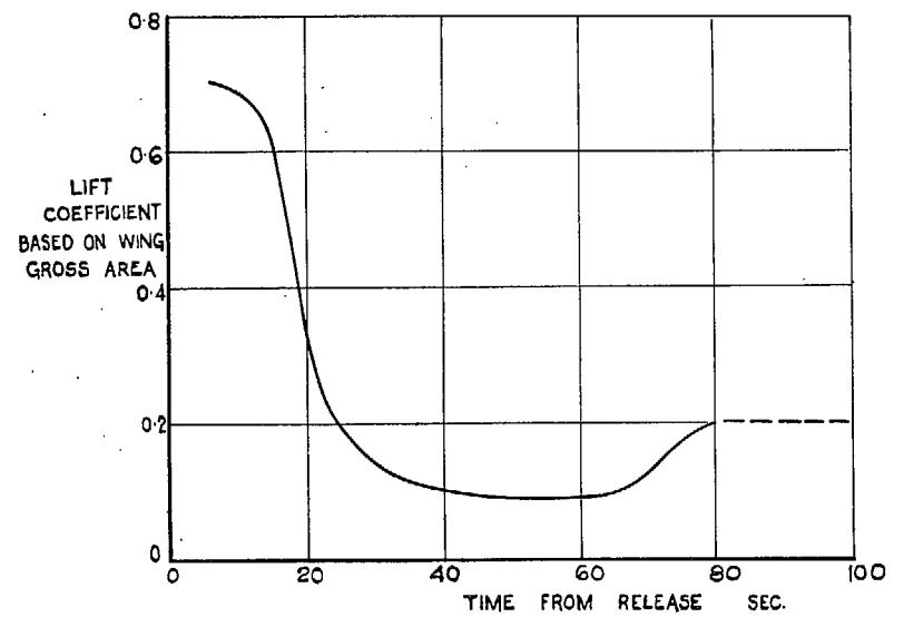
FIG. 10. Variation of lift coefficient during flight.
