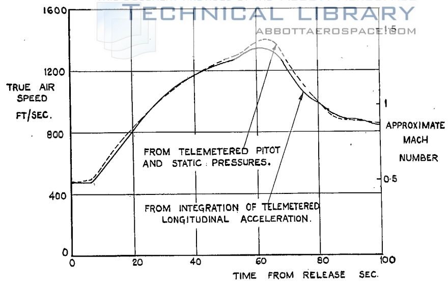
FIG. 7. Variation of speed during flight.
