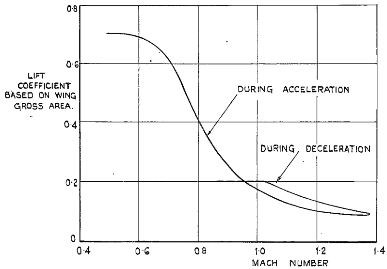
FIG. 16. Variation of lift with Mach number.
