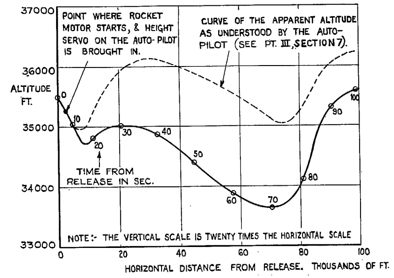
FIG. 9. Variation of altitude during flight.
