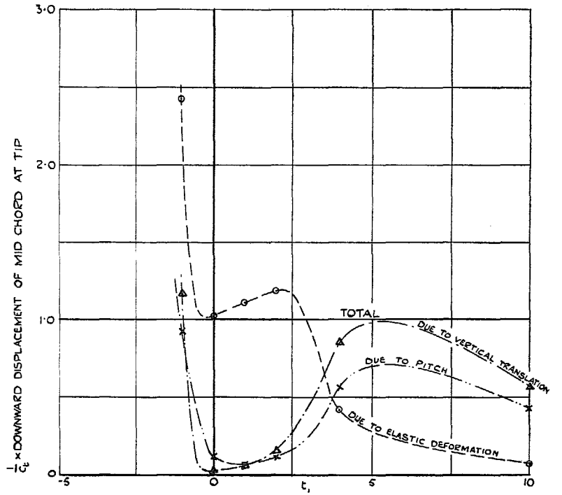
FIG. 26. Flexure-torsion flutter modes for (f_2/f_1)^2 = 5.0 : amplitudes.
