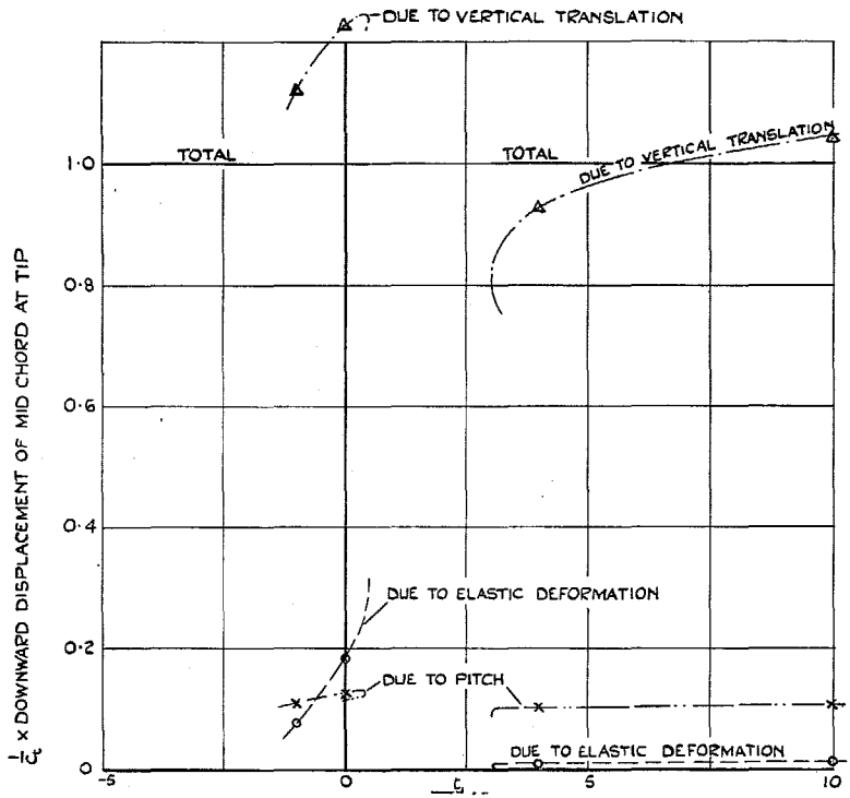
FIG. 24. Body-freedom flutter modes at lower critical speed for (f_2/f_1)^2 = 5.0 : amplitudes.
