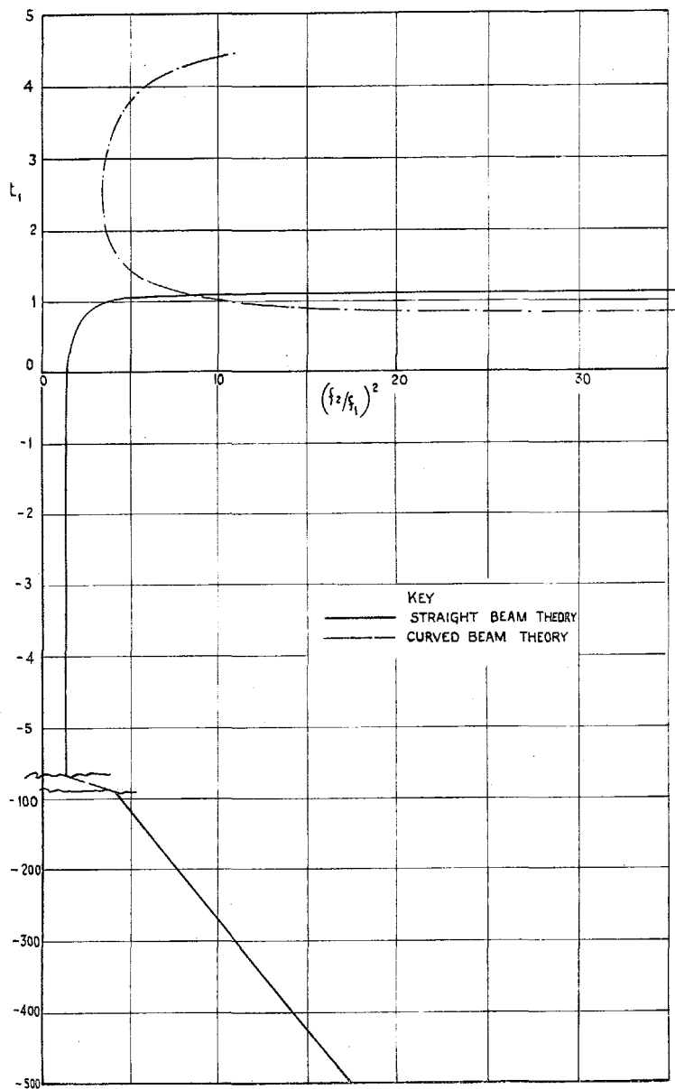
FIG. 29. Relationship between the modal parameter t_1 and the frequency ratio for two assumed structural forms.
