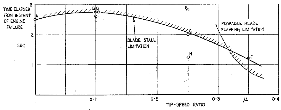
FIG. 9. Time available after engine failure.
