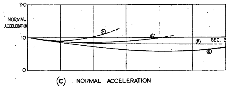
Figs. 5a, 5b and 5c. Effect of movements of pilot's control. \mu = 0.25 . \vartheta_0 = 8.6 deg. \Omega = 192 r.p.m.
