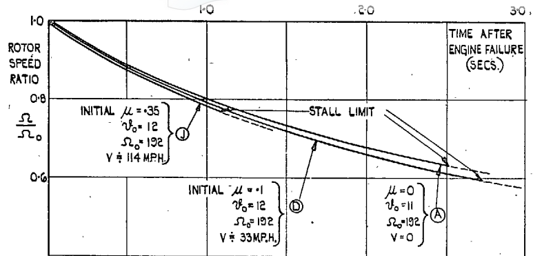
FIG. 1. Effect of forward speed on loss of rotor speed.
