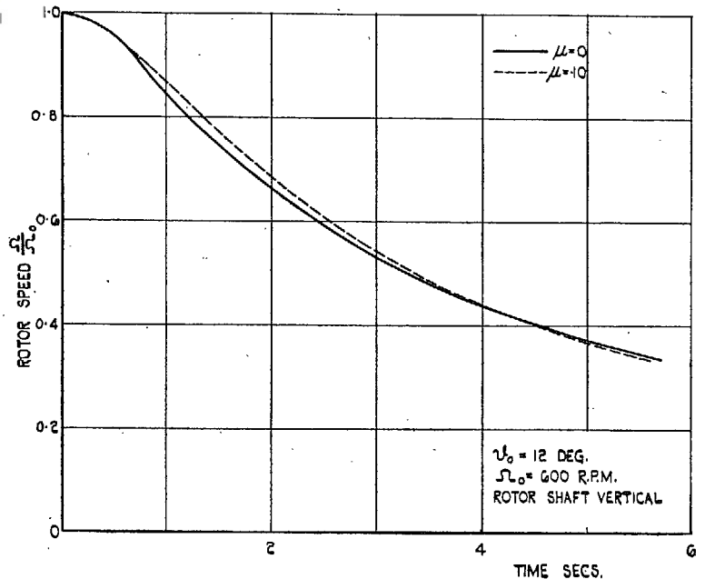
FIG. 8. 12-ft diameter model rotor tests.
