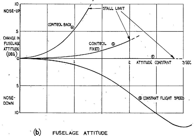
Figs. 6a and 6b. Effect of movements of pilot's control. \mu = 0.25 . \vartheta_0 = 8.6 deg. \Omega = 192 r.p.m.
