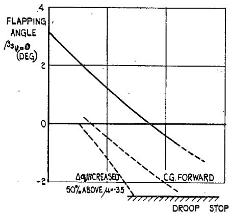
(c) FLAPPING ANGLE AT \psi = 0
