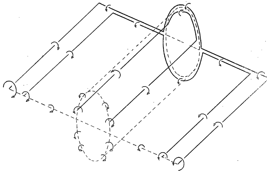
FIG. 6. Vortex system for wing-body combination.
