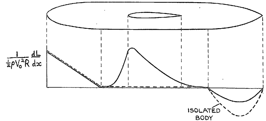
FIG. 3. Sketch of load distribution over body when attached to a wing.
