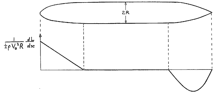
FIG. 2. Load distribution on isolated body with cylindrical middle part; equation (1).
