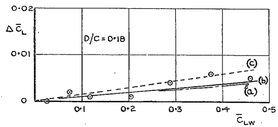
FIG. 11. Overall lift increment cylindrical bodies on swept wing. AR = 3 , \varphi = 45 deg, taper ratio = 1.0, t/c = 0.12 , Reynolds number = 0.7 \times 10^6 .
