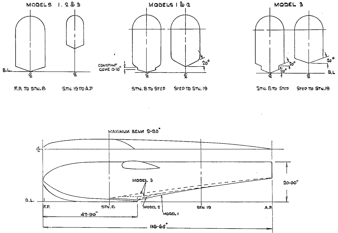
FIG. 5. Lines of Langley tank models with deep step faired in elevation and plan form. Fig. 1 of Ref. 5.
