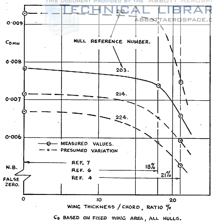
FIG. 15. Hull drags with and without wing interference.
