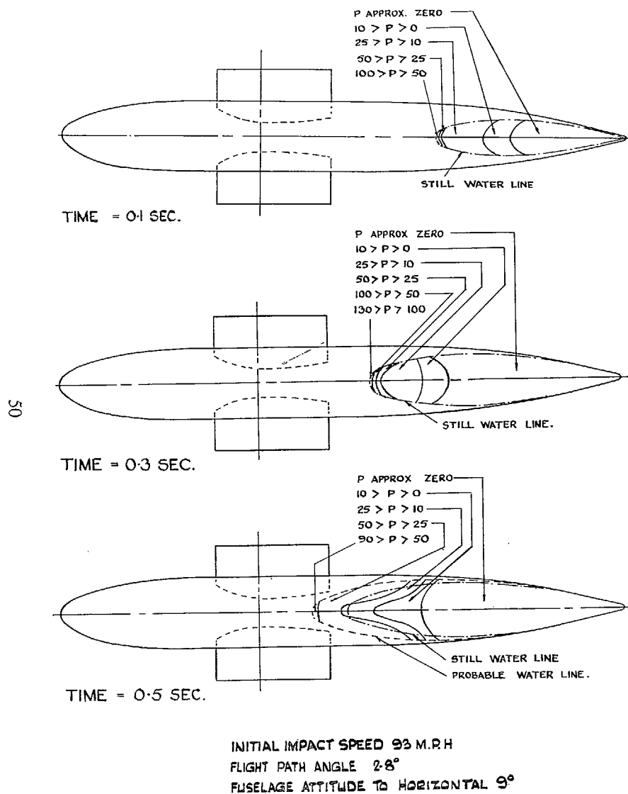
FIG. 21c. Pressure distribution at intervals of 0.2 sec.
