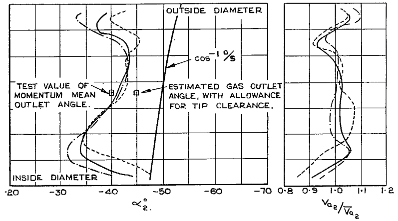
FIG. 5. Conventional rotor. Distributions of axial velocity and gas angle relative to rotor blade.
