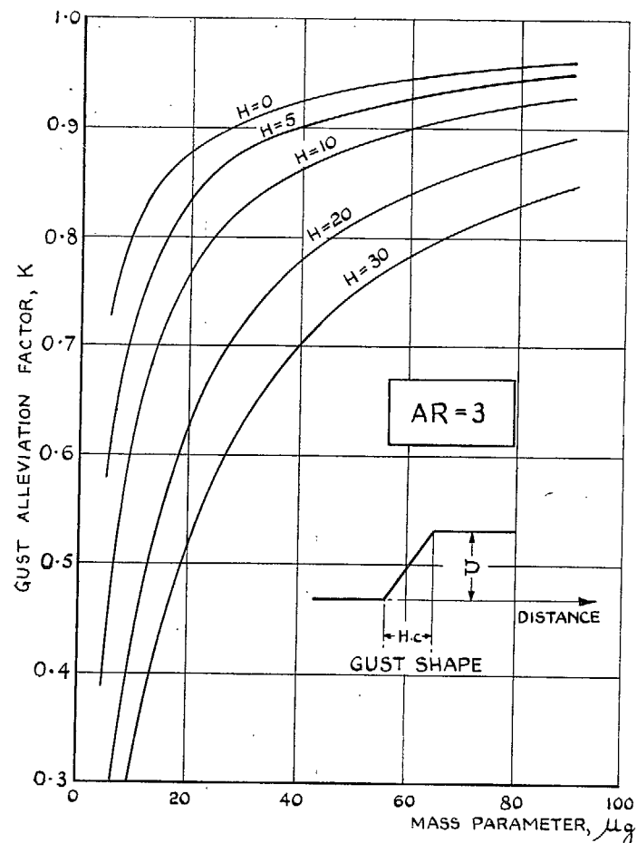
FIG. 5c. Gust alleviation factor vs. mass parameter for different gust gradients. Flat-topped gust. Aspect ratio 3.
