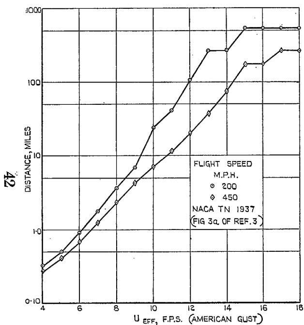
(a) WITHOUT COMPRESSIBILITY CORRECTION.
