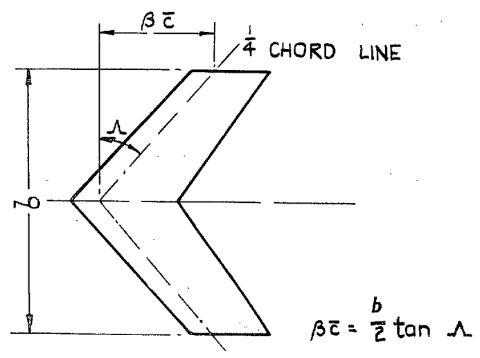
FIG. 1. Definition of sweep coefficient.
