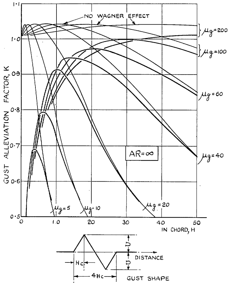
FIG. 8. Gust alleviation factor for the second, negative peak of double-triangular gust plotted against gust length. Aspect ratio \infty .
