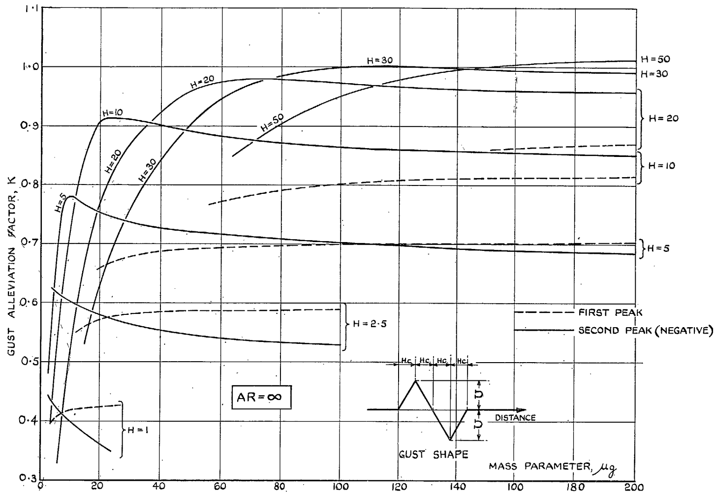
FIG. 9. Gust alleviation factor for double-triangular gust. Comparison of first and second (negative) peaks plotted against mass parameter for the range of gust gradients.
