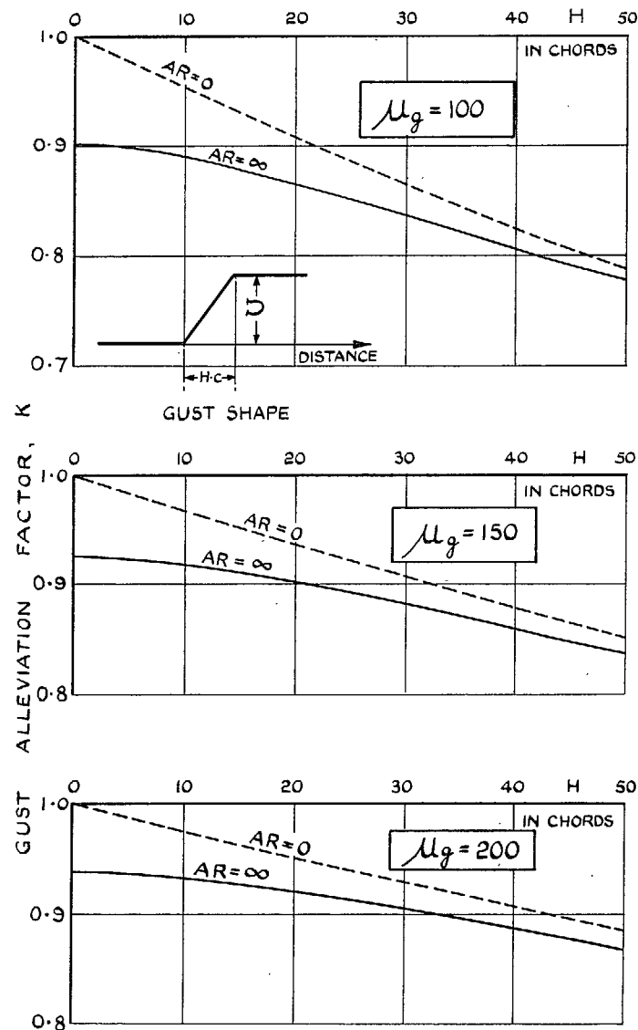
FIG. 4f. Gust alleviation factor vs. gust gradient for aspect ratios 0 and \infty . Flat-topped gust.
