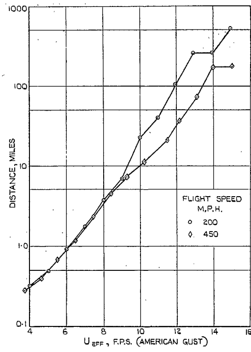
(c) LIFT SLOPE AND ALLEVIATION FACTOR CORRECTED FOR COMPRESSIBILITY.
