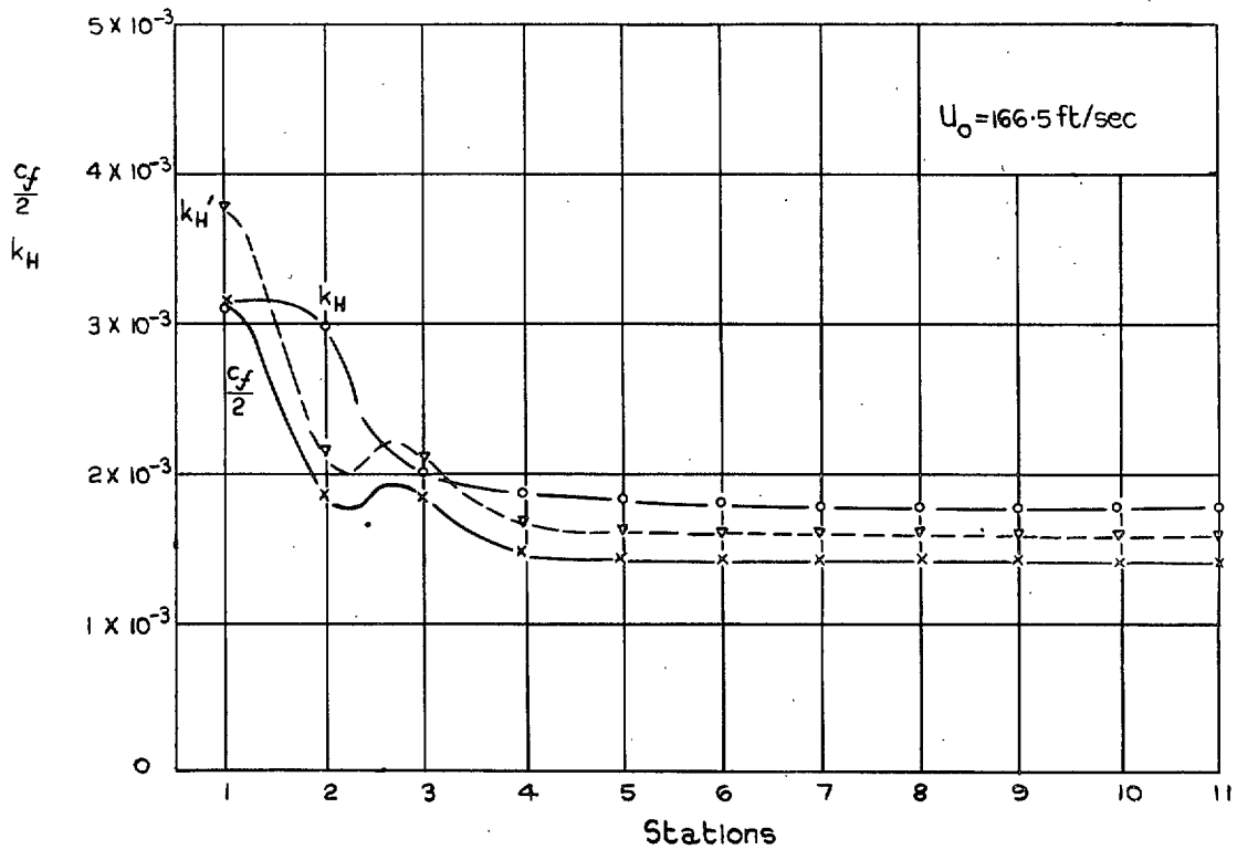
FIG. 5. Variation of c_f (S.T.) and h_H along 4-deg diffuser.
