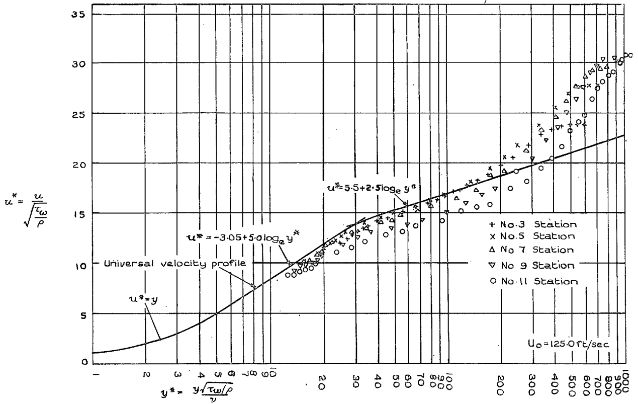
FIG. 12. Non-dimensional velocity profile (4-deg diffuser).
