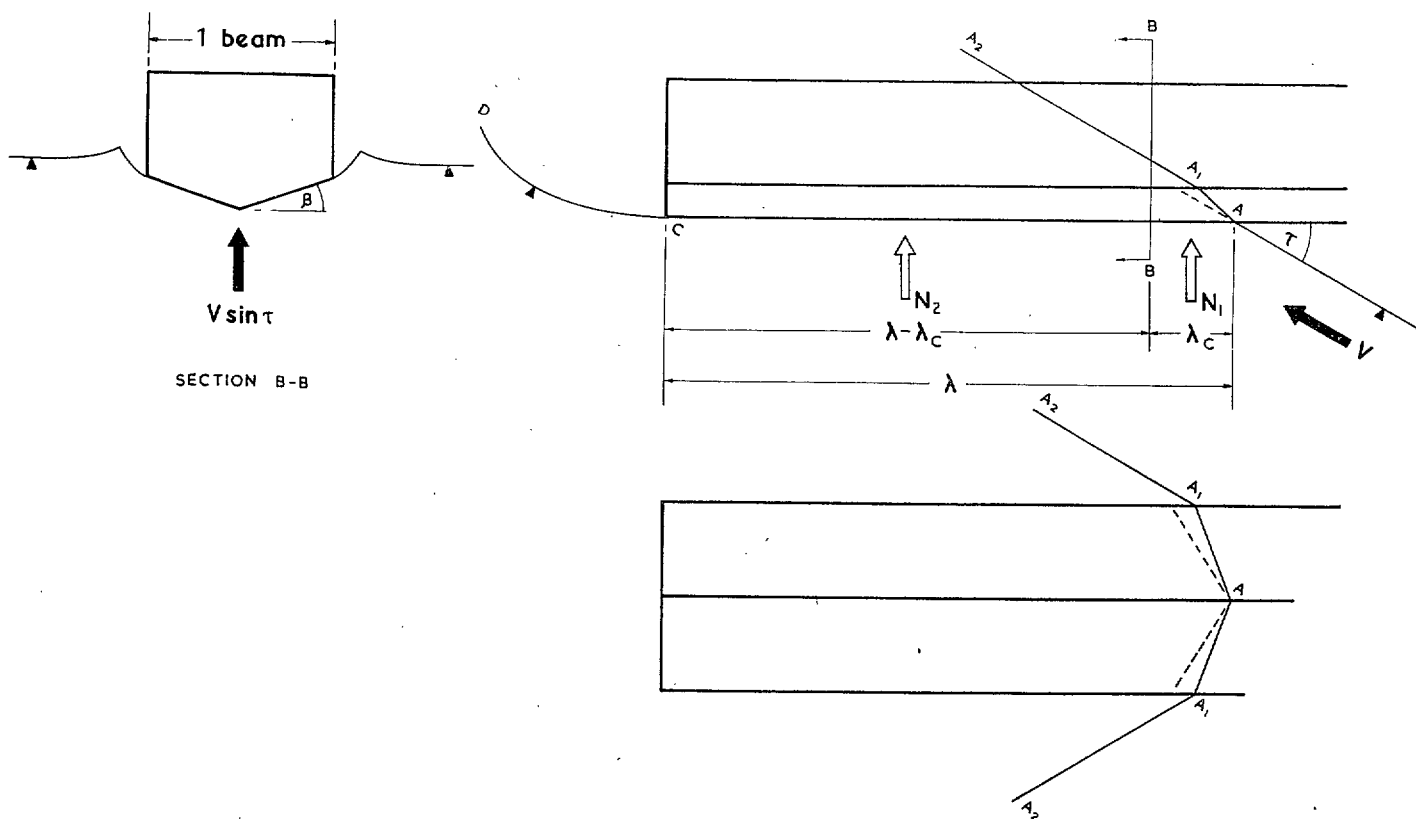
FIG. 1. Wedge planing chines wet.
