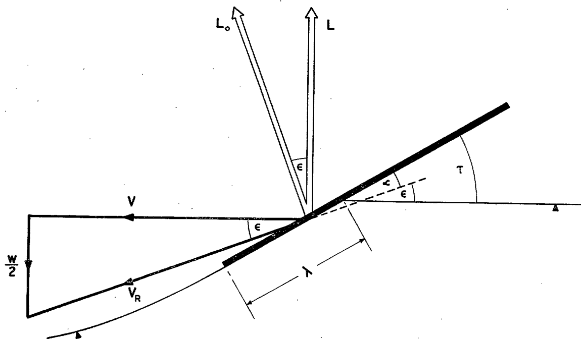
FIG. 2. Flat-plate planing.
