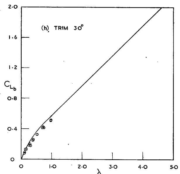
FIG. 6.— continued . Lift coefficient against wetted length. Zero deadrise.
