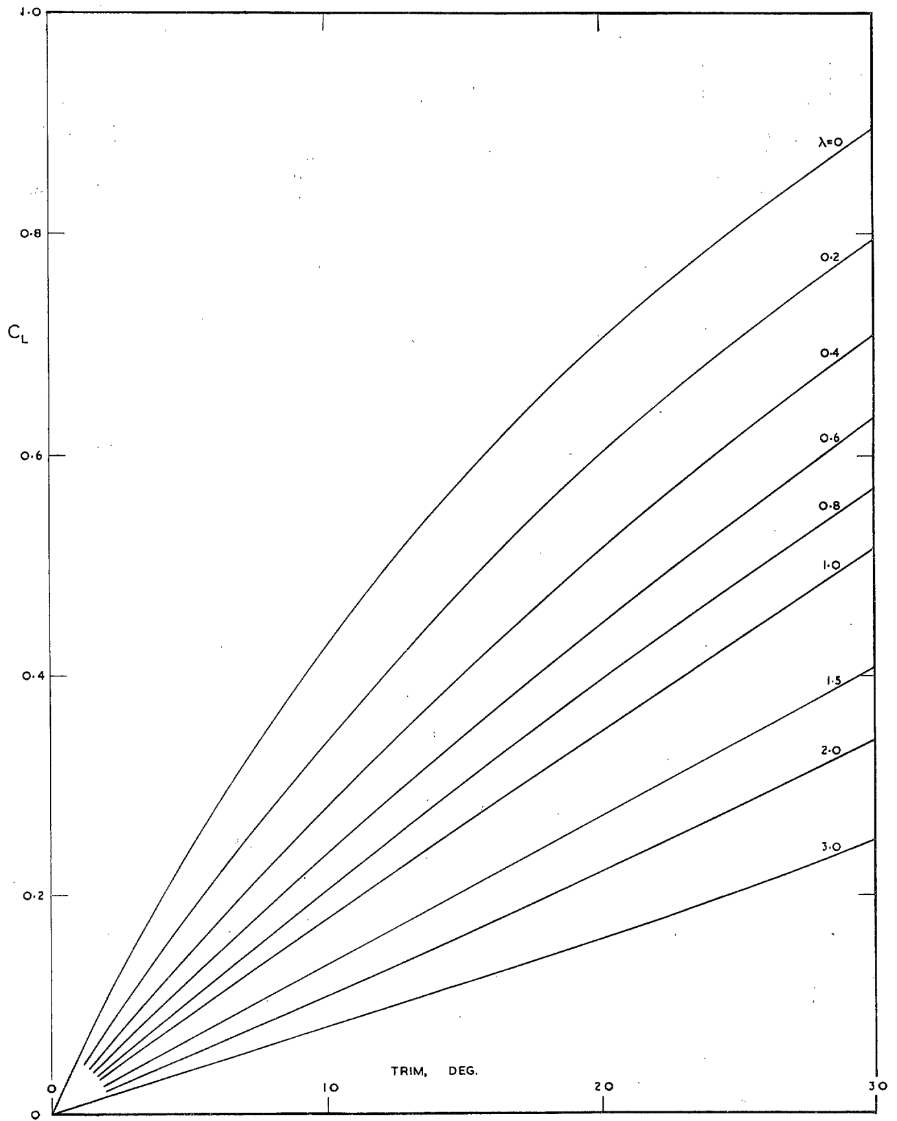
FIG. 3. Theoretical flat-plate lift coefficient.
