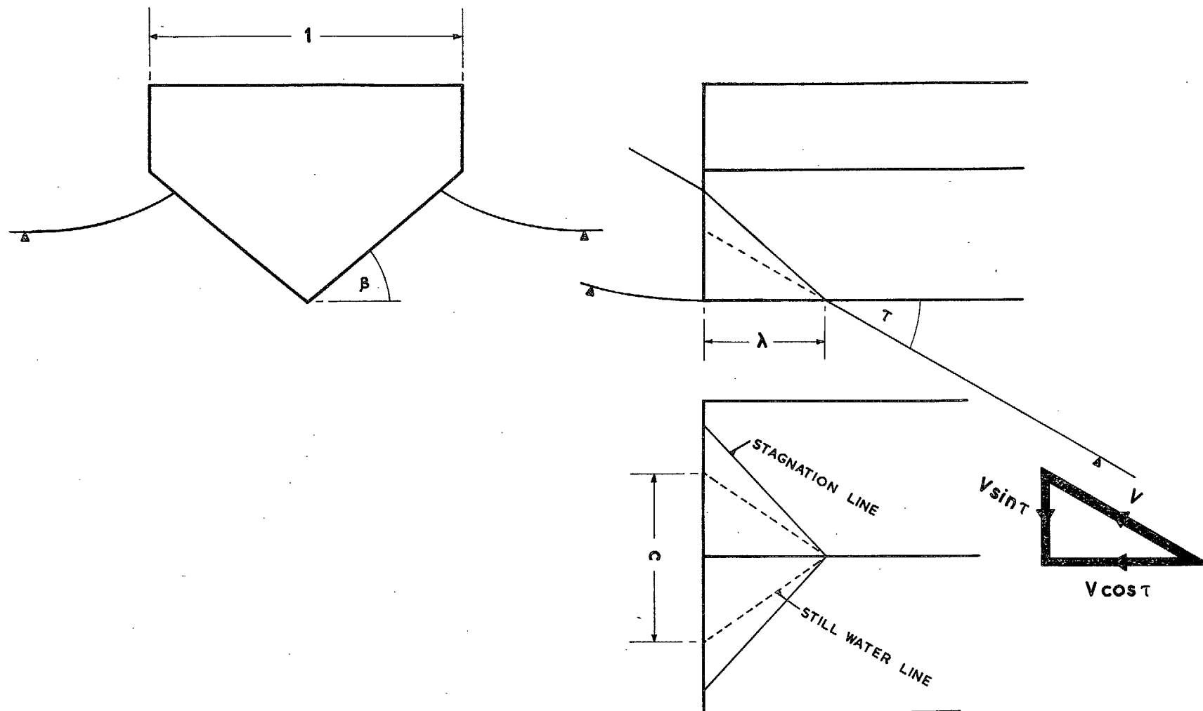
FIG. 5. Wedge planing chine dry.
