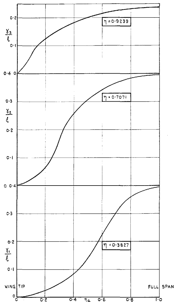
FIG. 35. Variation of span-loading coefficients ( \gamma/\epsilon ) at three spanwise stations for the limit A \rightarrow 0 with aileron span ratio ( \eta_a = 1 - \eta_0 ) for antisymmetrical deflection.
