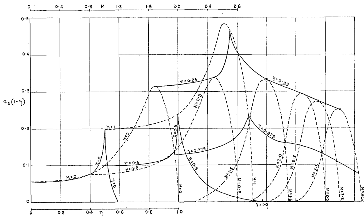
FIG. 28. Variation of the local lift coefficient due to symmetrical deflection of controls of span ratio 0.261 with spanwise location and Mach number for a delta wing A=2.31 .
