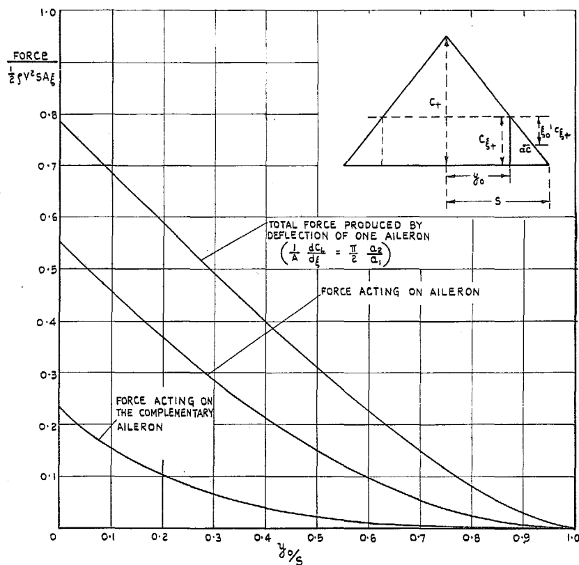
FIG. 19. Lift produced on the various parts of the wing by deflection of the control on one side only (Sonic speed).
