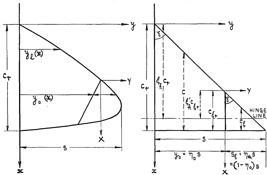
FIG. 1a. An all-moving wing-tip control fitted to typical wings, the sections of which consist of one segment only.
