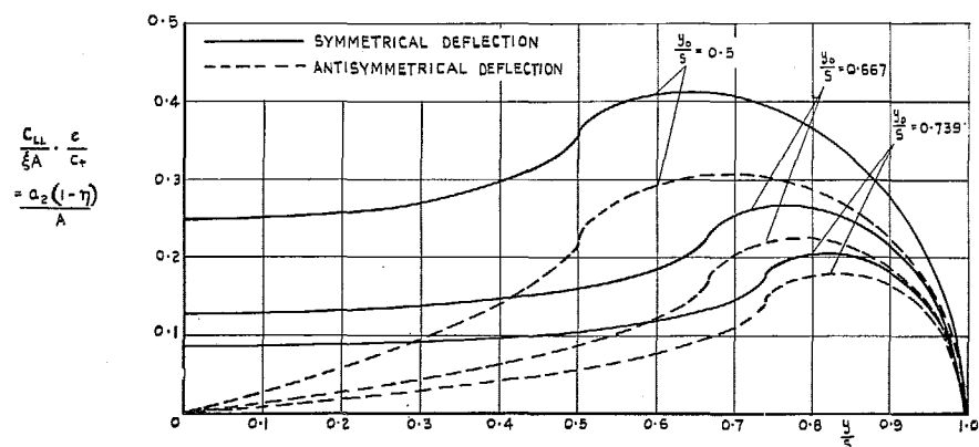
FIG. 16. Spanwise loadings due to symmetrical and antisymmetrical deflection of controls of various span ratio, fitted to a delta wing, at sonic speed.
