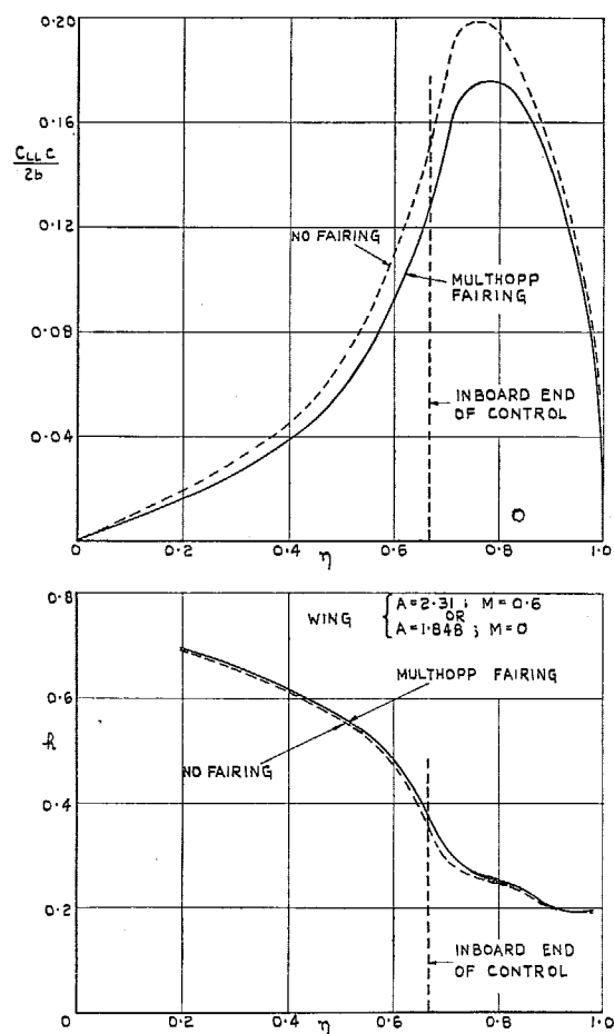
FIG. 11. Effect of fairing the incidence distribution on the span loading and aerodynamic-centre locus for antisymmetrical deflection of the controls of span ratio 0.335.
