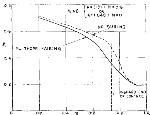
FIG. 9. Effect of method of fairing the discontinuity in incidence on the span loading and aerodynamic-center locus due to antisymmetric deflection of controls of span ratio 0.261.
