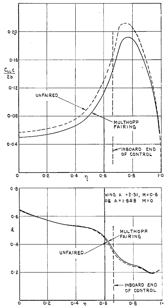
FIG. 12. Effect of fairing the incidence on the span loading and aerodynamic-centre locus for symmetrical deflection of controls of span ratio 0.335.
