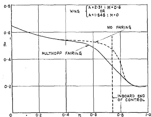
FIG. 10. Effect of method of fairing the discontinuity in incidence on the span loading and aerodynamic-center locus due to symmetric deflection of controls of span ratio 0.261.
