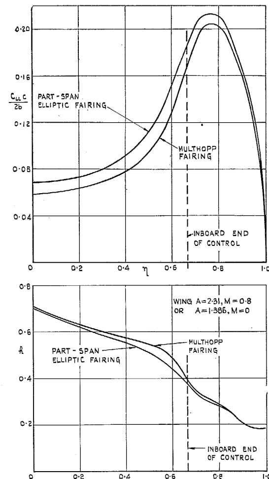
FIG. 13. Comparison of two methods of fairing the discontinuity in incidence for symmetrical deflection of a tip control of span ratio 0.335 on a delta wing.
