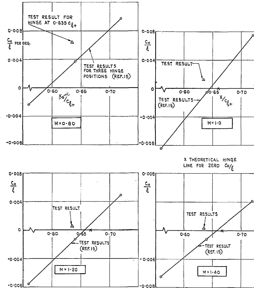
FIG. 34. Variation of mean slope of hinge-moment coefficient (per degree) over control-angle range 0 to -5 -deg. at various Mach numbers.
