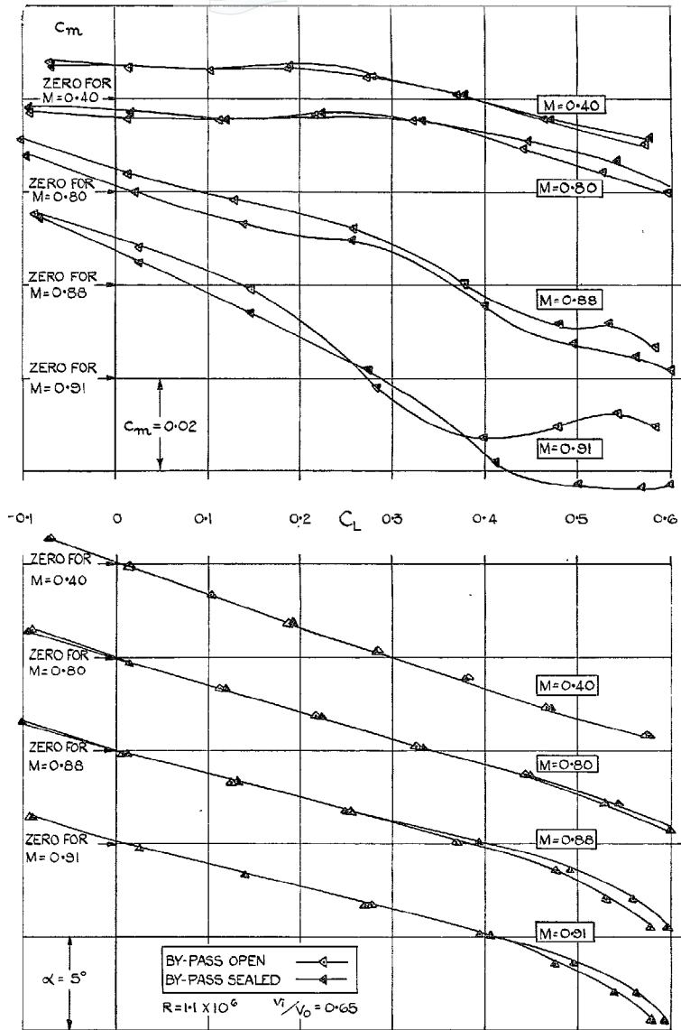
FIG. 21a. Effect of sealing boundary-layer by-pass of wing-root intake. C_m vs. C_L , C_L vs. \alpha .
