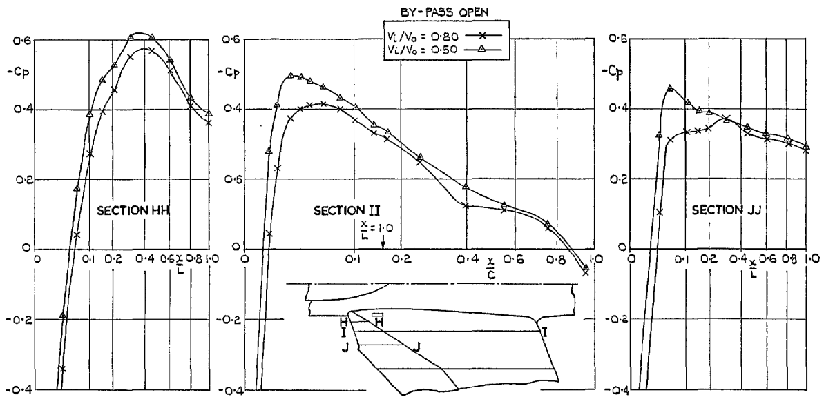
FIG. 28a. Effect of velocity ratio on pressure distribution over the wing-root intake at M = 0.40 ( \alpha = 0 deg).
