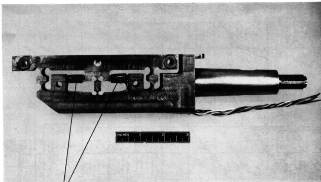
FIG. 6b. The strain-gauge 'drag balance'.
