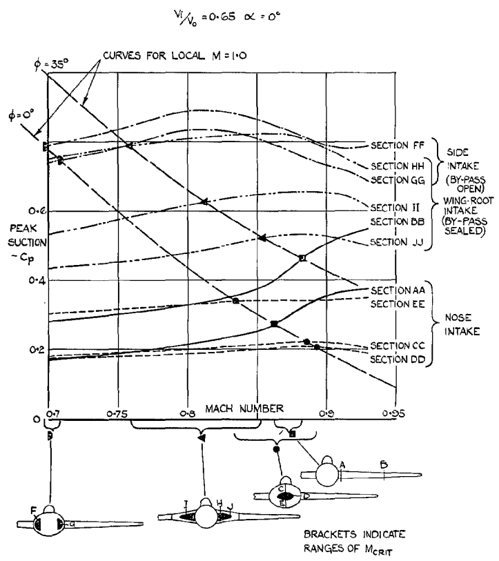
FIG. 17. Variation of measured peak suction with Mach number at \alpha = 0 deg, showing critical Mach numbers for the intake fairings. Comparison between the different intake designs.
