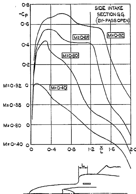
FIG. 11b. Comparison between the pressure distributions at \alpha = 0 deg on the side and nose-intake lip fairings ( V_i/V_0 = 0.65 ).
