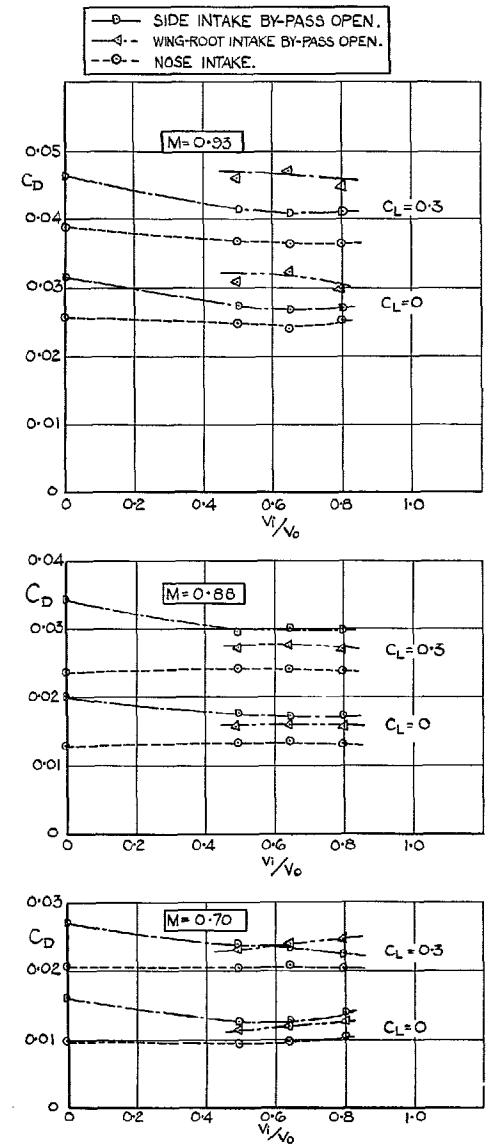
FIG. 24. Effect of velocity ratio on the drag of the three intake designs. Gross C_D vs. V_i/V_0 .
