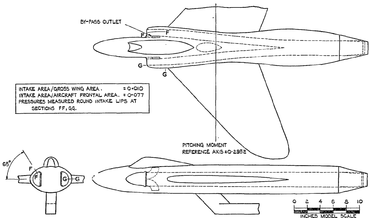
FIG. 2c. General arrangement of side-intake model.
