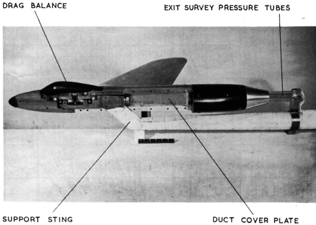
FIG. 6a. Interior view of side intake model.
