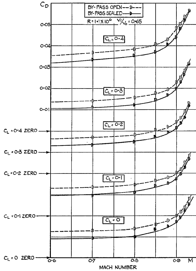
FIG. 19. Effect of sealing boundary-layer by-pass of side intake. Gross C_D vs. Mach number at constant C_L .
